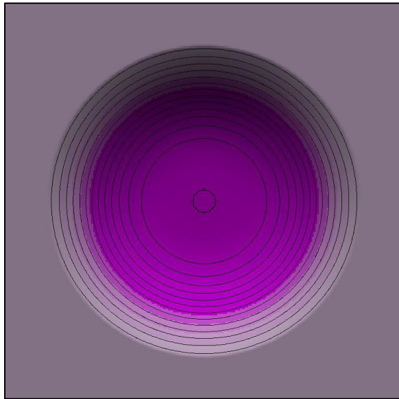
Figure 1. Shaded relief of hill. 30 meter contour lines are shown.
