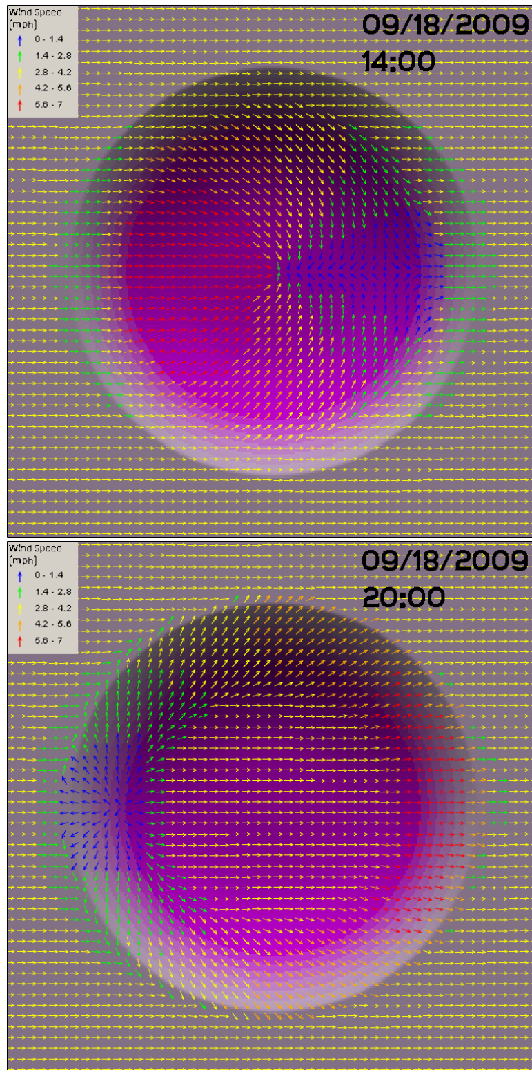
Figure 4. Surface winds for 1.3 \text{ m s}^{-1} (3 mph) ambient cross flow.
