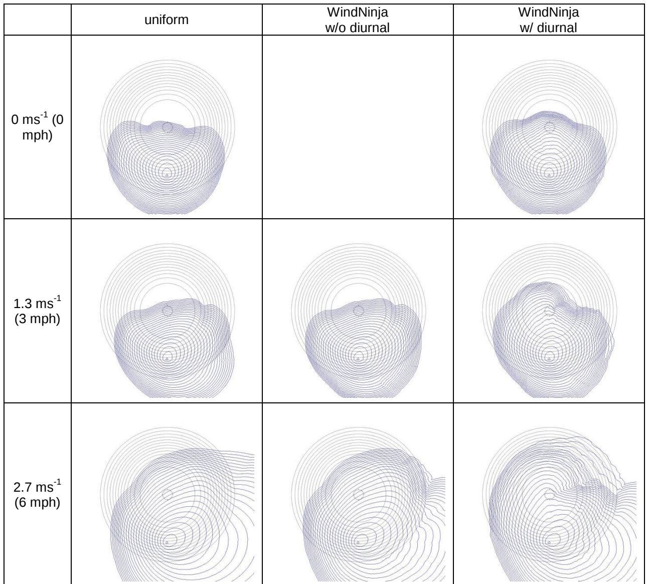
Figure 6. Comparison of fire progression from 0800-2000 on September 18 th using different wind fields. Fire isochrons, shown in blue, represent 30 minute spacing. Gray lines are 30 meter elevation contours.
