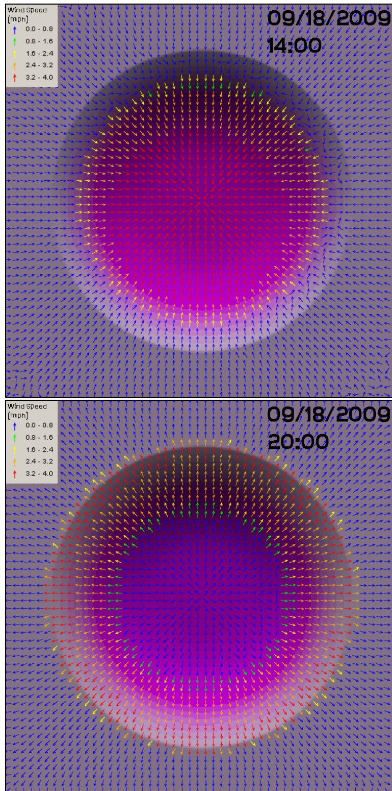
Figure 3. Surface winds for 0 mph ambient cross flow.
