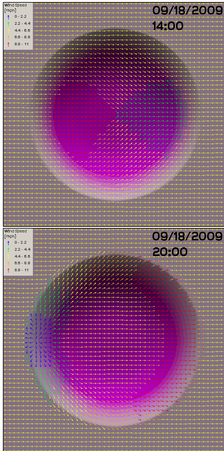
Figure 5. Surface winds for 2.7 \text{ m s}^{-1} (6 mph) ambient cross flow.
