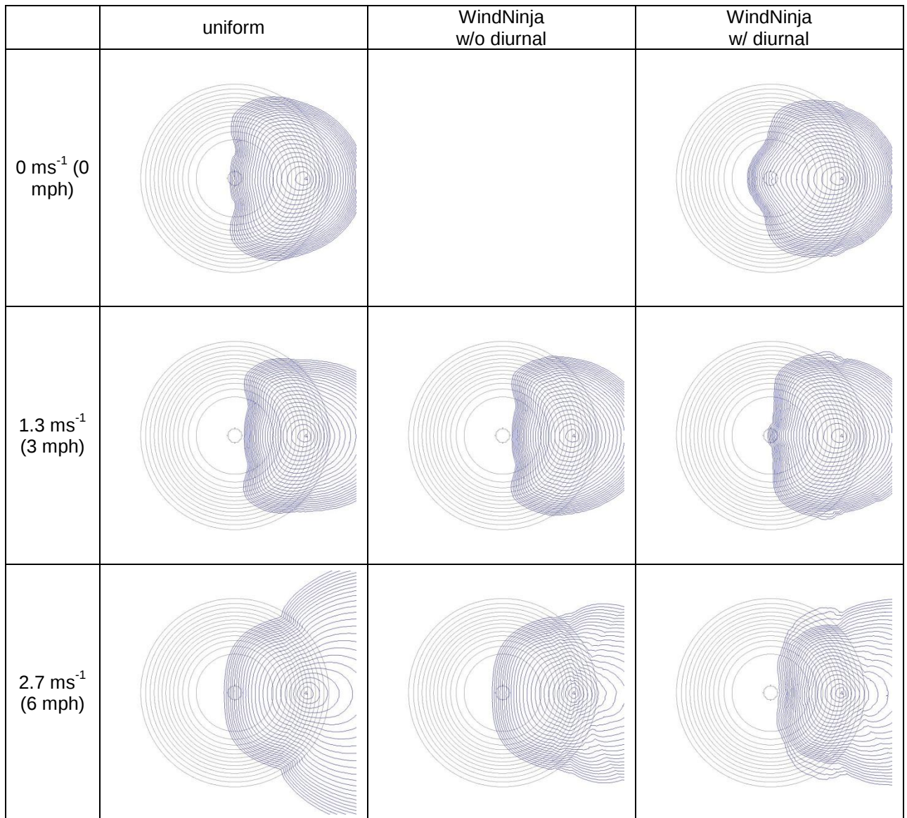
Figure 7. Comparison of fire progression from 0800-2000 on September 18 th using different wind fields. Fire isochrons, shown in blue, represent 30 minute spacing. Gray lines are 30 meter elevation contours.
