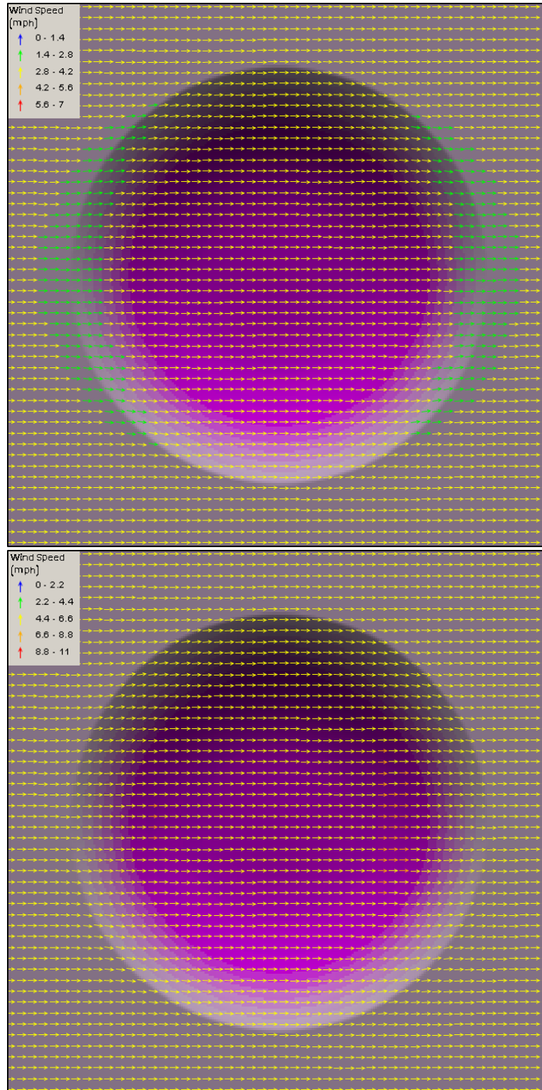
Figure 2. Surface winds for ambient cross flow speeds of 1.3 m s -1 (3 mph) (top image) and 2.7 m s -1 (6 mph) (bottom image) with no diurnal winds. Note different wind speed legends.
