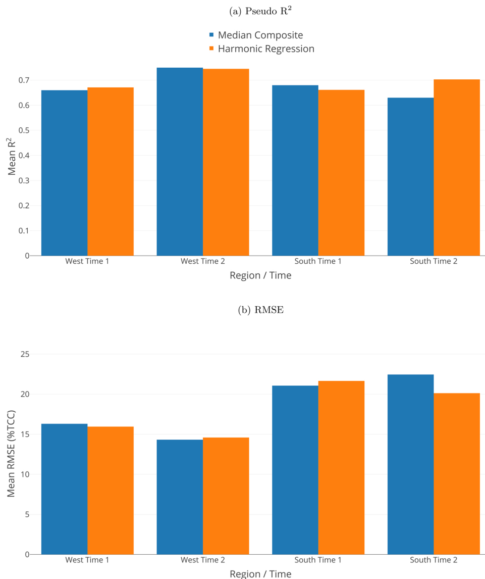
Fig. 8. Comparison of models using the full suite of median composite and terrain variables used in the original 2011 TCC product to models using the harmonic regression coefficients for NDVI, SWIR1, and SWIR2.
