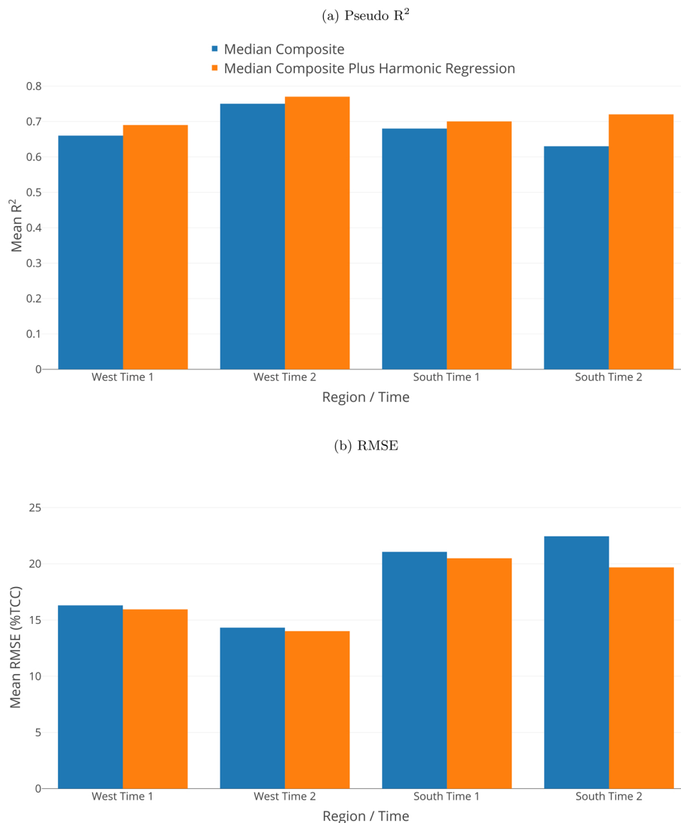
Fig. 7. Comparison of models using the full suite of median composite and terrain variables used in the original 2011 TCC product to models using the full suite of median composite and terrain variables used in the 2011 TCC product plus the harmonic regression coefficients from NDVI, SWIR1, and SWIR2.
