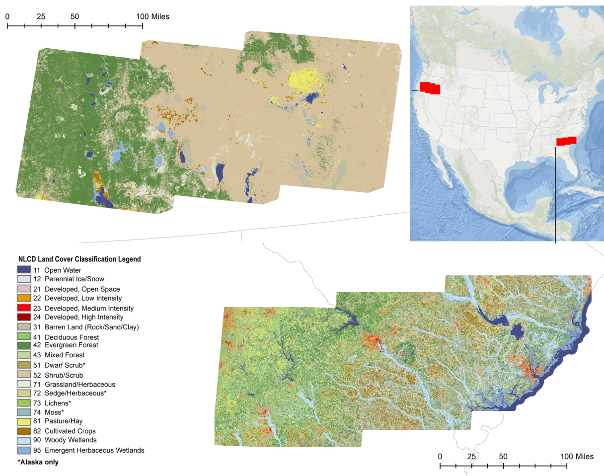
Fig. 3. Western(top) and Southern(bottom) study areas with 2011 National Land Cover Database classification.
