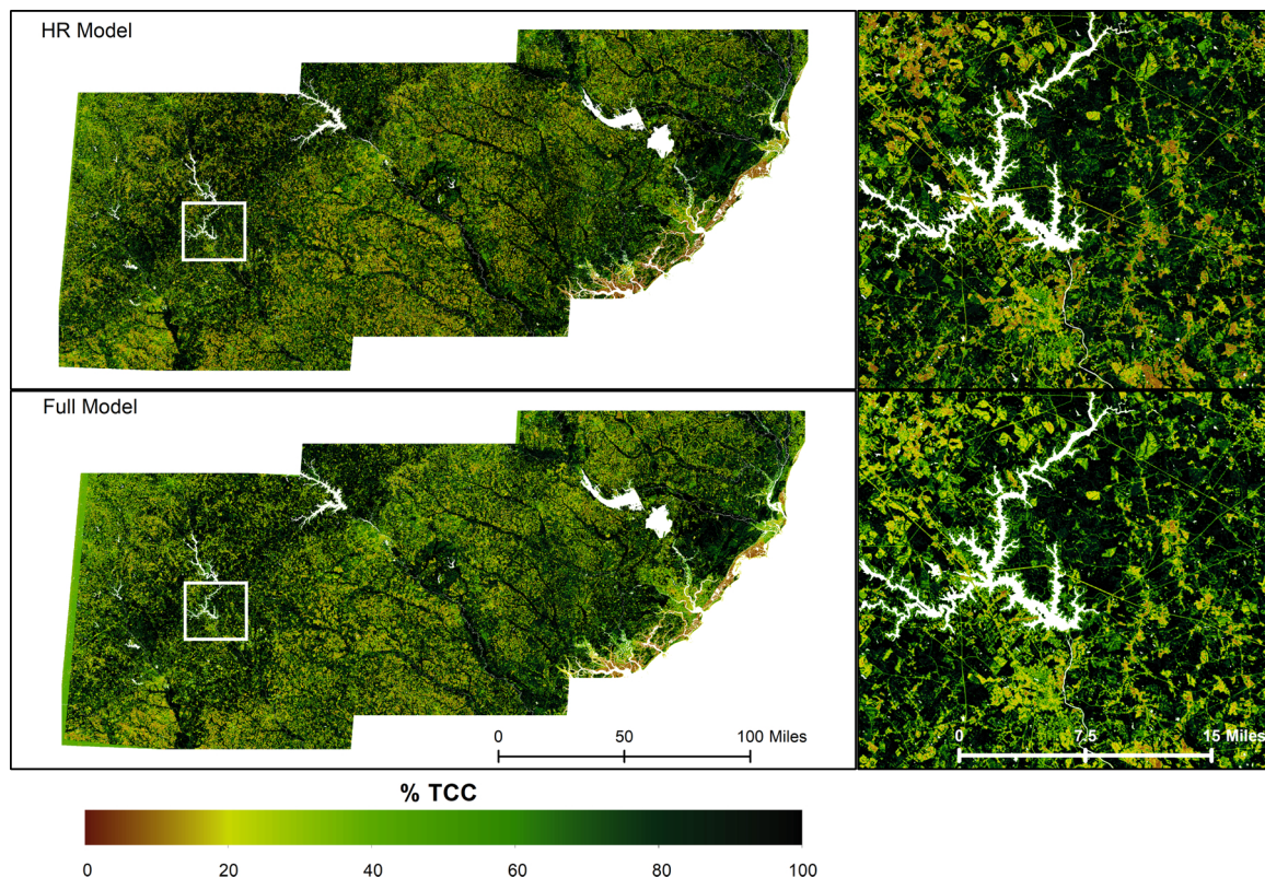
Fig. 12. TCC maps (Time 2) for the southern study area for the two models ( HR and Full ) using harmonic regression coefficients as part of the predictor variable suite.
