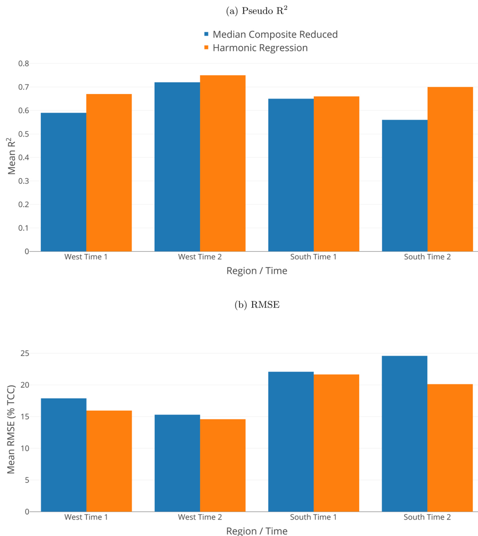
Fig. 6. Comparison of models using harmonic regression coefficients for NDVI, SWIR1 and SWIR2 to the median composite values for those same three bands.
