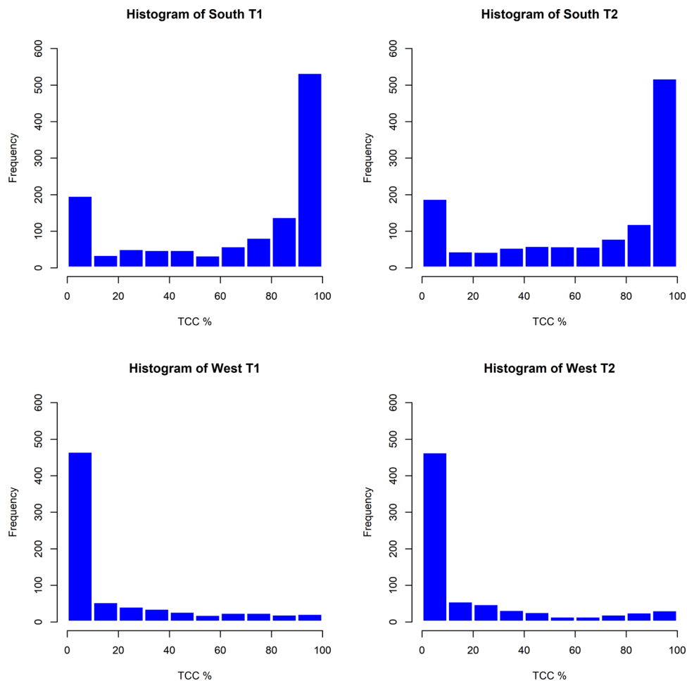
Fig. 4. Histograms of photo interpreted TCC observations for T1 (time 1) and T2 (time 2) in the South and West.
