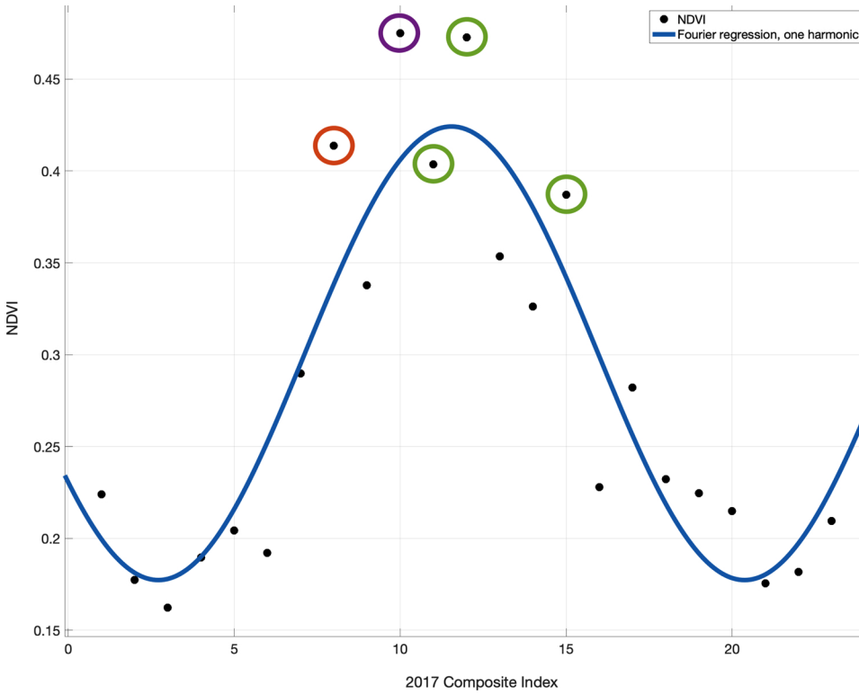
Fig. 1. Median composite and harmonic regression. This figure illustrates the median composite method using NDVI data from MODIS 250 m 16-day composites from 2017 (MYD13Q1 collection 6, coordinates 37.4378°, -80.2727°). Landsat median composite images are calculated using the median reflectance value from up to 15 images from three years preceding the target year. In this example, the maximum MODIS NDVI value is shown, circled, in violet. The Landsat median composite selects observations within 0.1 GLOVIS maximum annual NDVI value (circled in green or red for this example, using annual maximum MODIS NDVI) are used to calculate the median composite, circled in red. (Note that for non-composited Landsat data the earliest and latest value within 0.1 NDVI of the maximum serve to define the range of data used, and the pixel-specific effects of cloud cover result in a median being computed with different numbers of values from pixel to pixel.) The figure also demonstrates the harmonic regression method with MODIS NDVI data. Harmonic regression of surface reflectance observations uses all available observations (black dots) and fits a harmonic curve (blue line) following Eq. (1). Both methods exclude observations identified as cloud cover. (For interpretation of the references to color in this figure legend, the reader is referred to the web version of this article.)
