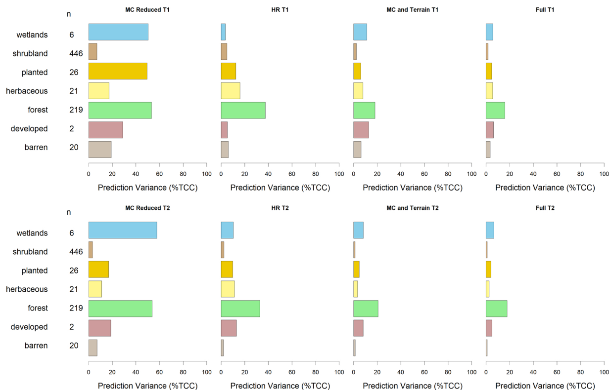
Fig. 14. Mean variance by NLCD land cover class (water excluded) for West, all models.
