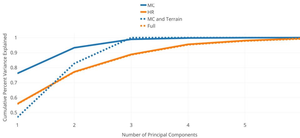
Fig. 11. Eigen analysis of predictor variable sets (South Time 2 shown). The cumulative percent variance explained for a given principal component is calculated as the sum of the eigen values up to and including that principal component divided by the sum of all eigen values for that predictor variable set. Only six principal components are shown for clarity, but the number of principal components for a given predictor variable set is the same as the number of predictor variables in that set. Inherent dimensionality as used here is the number of principal components it takes to explain nearly all the variance, defined as 99%. Note the following: (1) harmonic regression coefficients, alone, or in combination with other predictor variables, have higher inherent dimensionality (and thus information content),
