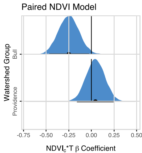
FIGURE 5 Mean \beta coefficient values (black dots) and 95% credible intervals (black lines) for the interaction variable NDVI_c * T in the paired Normalized Difference Vegetation Index (NDVI) model (Equation 1), separated by watershed grouping. Negative \beta values indicate that the NDVI_t vs NDVI_c relation had a lower slope in the posttreatment period, which we attribute to less forest mortality in the treated watersheds relative to the control watershed. Blue area represents density plot of 10,000 individual model runs
