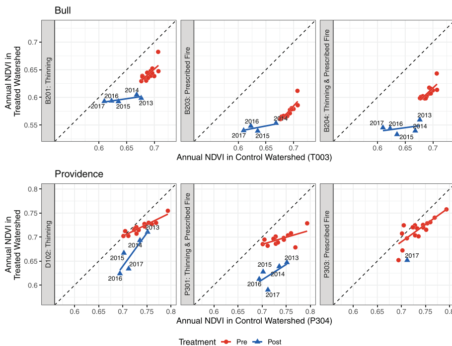
FIGURE 4 Relation between the watershed-averaged annual May–September maximum Normalized Difference Vegetation Index (NDVI) in the treated watershed ( NDVI_t ) and the control watershed ( NDVI_c ). Linear regression lines were separately fit to pretreatment and posttreatment values. Corresponding years are displayed for all posttreatment values. Dashed line designates 1:1 line
