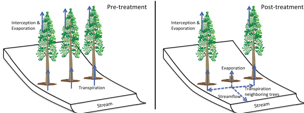
FIGURE 1 Conceptual model of pre- and post-treatment water pathways
