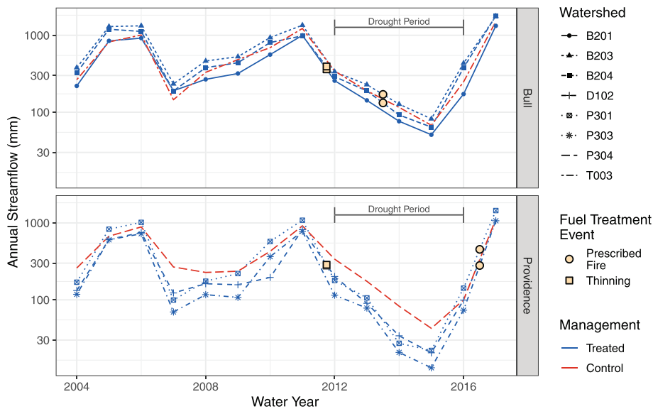
FIGURE 6 Time-series of observed annual streamflow for each watershed, separated by Bull and Providence groupings. Thinning events are shown as filled squares and prescribed fire events are shown as filled circles
