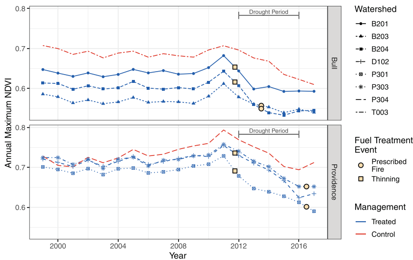
FIGURE 3 Time-series of the annual May to September maximum-value Normalized Difference Vegetation Index (NDVI) for each watershed, separated by Bull and Providence groupings. Thinning events are shown as filled squares and prescribed fire events are shown as filled circles
