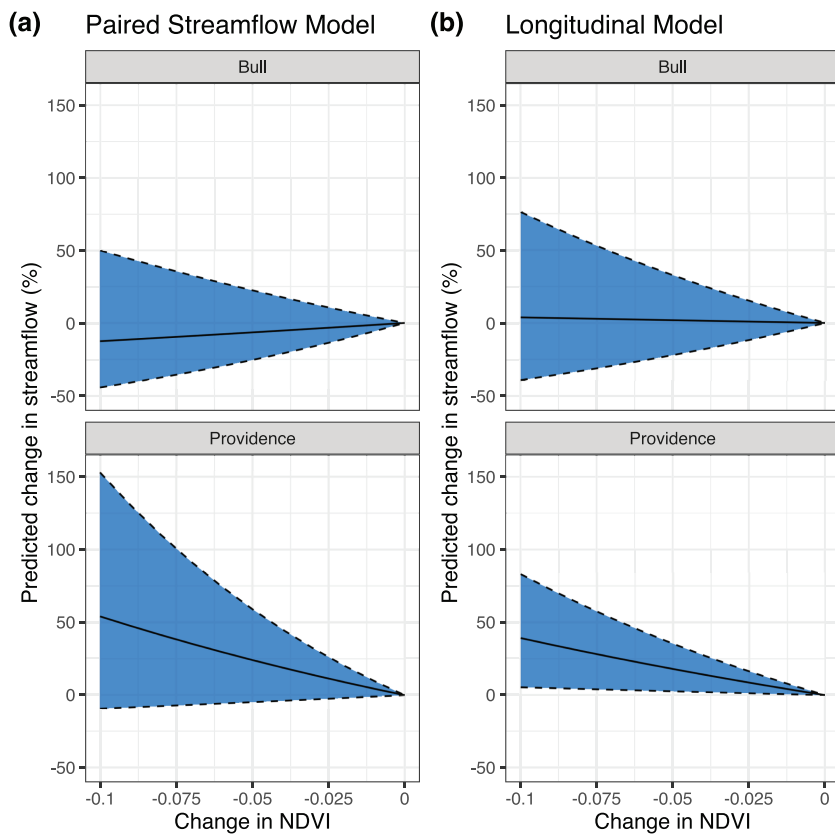
FIGURE 9 Predicted change in annual streamflow for a given change in Normalized Difference Vegetation Index (NDVI) based on the calibrated paired streamflow and longitudinal models. The blue area indicates 95% uncertainty intervals
