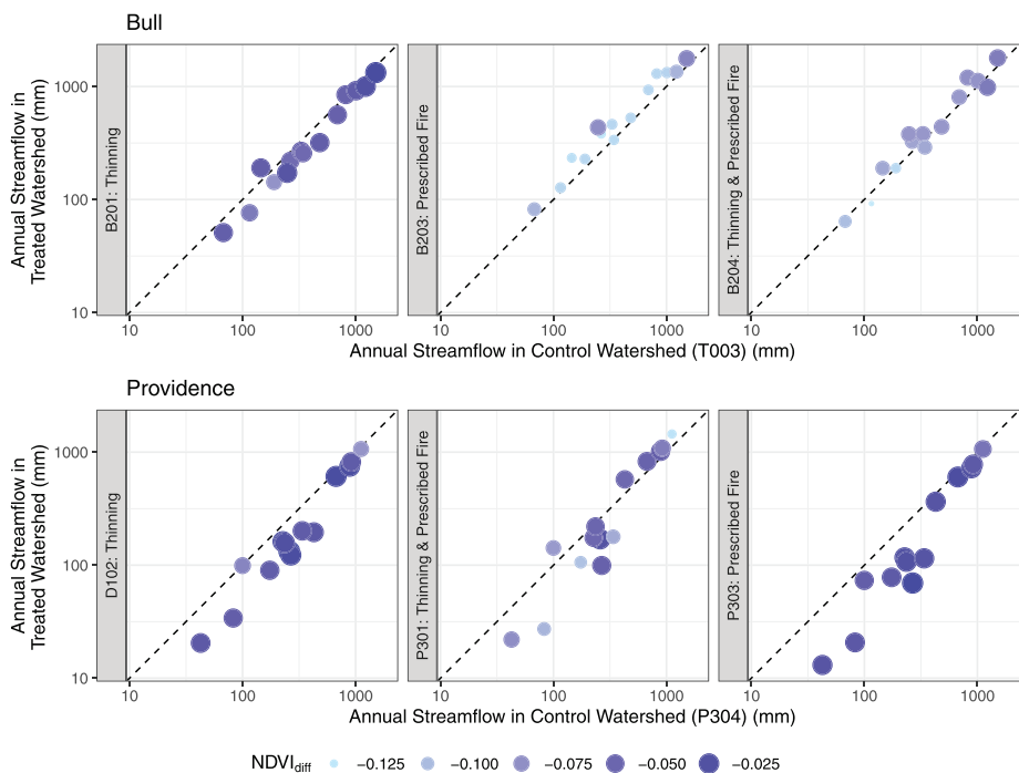
FIGURE 7 Relation between annual streamflow in the control watershed ( Q_c ) and the annual streamflow in the treated watershed ( Q_t ). Smaller and lighter blue circles correspond to lower Normalized Difference Vegetation Index (NDVI) values in the treated watershed relative to the control watershed (i.e., more negative NDVI_{diff} ). Dashed line designates 1:1 line
