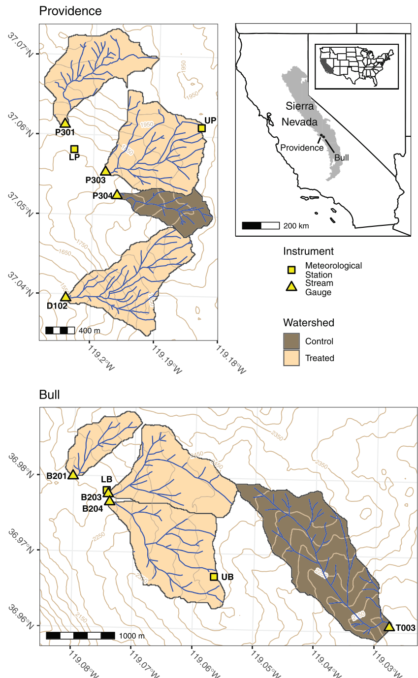
FIGURE 2 Map of the Kings River Experimental Watersheds. Meteorological stations UP, LP, UB and LB correspond to Upper Providence, Lower Providence, Upper Bull and Lower Bull, respectively
