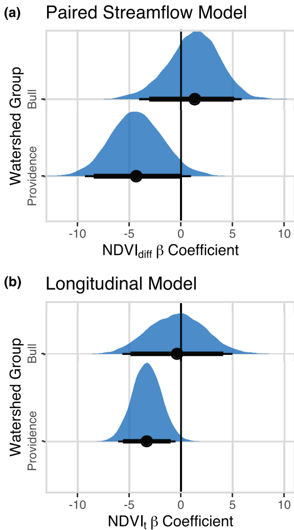
FIGURE 8 Mean \beta coefficient values (black dots), 90% credible intervals (thick line) and 95% credible intervals (thin line) for the variables NDVI_{diff} and NDVI_t in the paired streamflow model (Equation 2) and the longitudinal model (Equation 3), respectively. Negative \beta values indicate an increase in annual streamflow in the treated watershed for (a) a corresponding decrease in Normalized Difference Vegetation Index (NDVI) of the treated watershed relative to the control watershed (Paired Streamflow Model) or (b) a decrease in NDVI in the treated watershed (Longitudinal Model). Blue area represents density plot of 10,000 individual model runs
