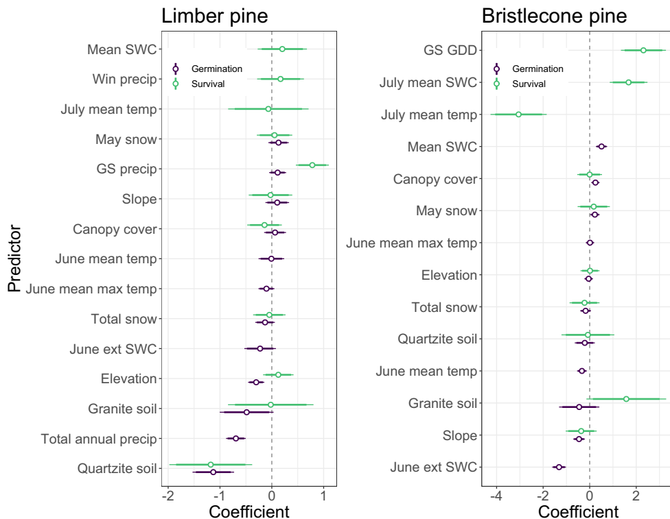
Fig. 7 Mean coefficient estimates from all binomial models with a \delta\text{AIC} < 4 for limber pine and bristlecone pine germination (purple) and survival (green). Error bars are the 90% and 95% confidence intervals but are not meant to represent “significance.” Parameter inclusion here by default makes them “significant” since they are included in the best model(s) as determined by AIC. The lack of a coefficient value for a predictor indicates
