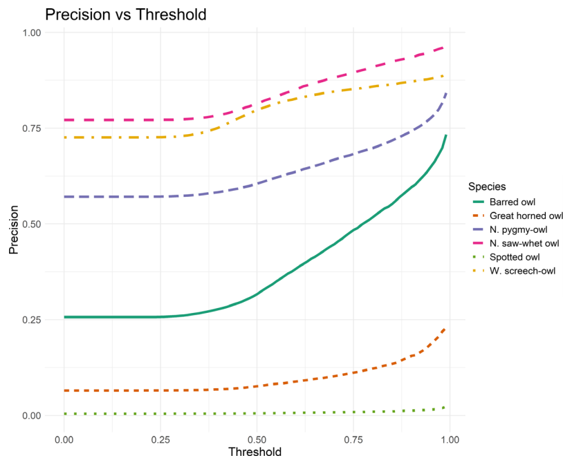
Figure 4. Precision vs threshold for six owl species. Precision or True Positive Rate is calculated as [\text{True Positives}] / [\text{True Positives} + \text{False Positives}] , considering only clips with p_{\text{Max}} \geq \text{Threshold} , where p_{\text{Max}} is the maximum class score predicted by the convolutional neural network. Precision represents the proportion of apparent detections that correspond to real target species calls.
