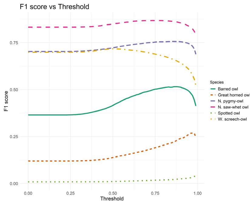
Figure 5. F1 score vs threshold for six owl species. F1 score is interpreted as a balanced measure of overall classifier performance combining precision and recall. The F1 score can be weighted to emphasize either precision or recall; we have plotted the unweighted version, calculated as 2 * [\text{Precision} * \text{Recall}] / [\text{Precision} + \text{Recall}] , considering only clips with p_{\text{Max}} \geq \text{Threshold} , where p_{\text{Max}} is the maximum class score predicted by the convolutional neural network. The highest point on each curve represents the threshold at which the model gives the best overall performance for each species if we consider precision and recall to be equally important.
