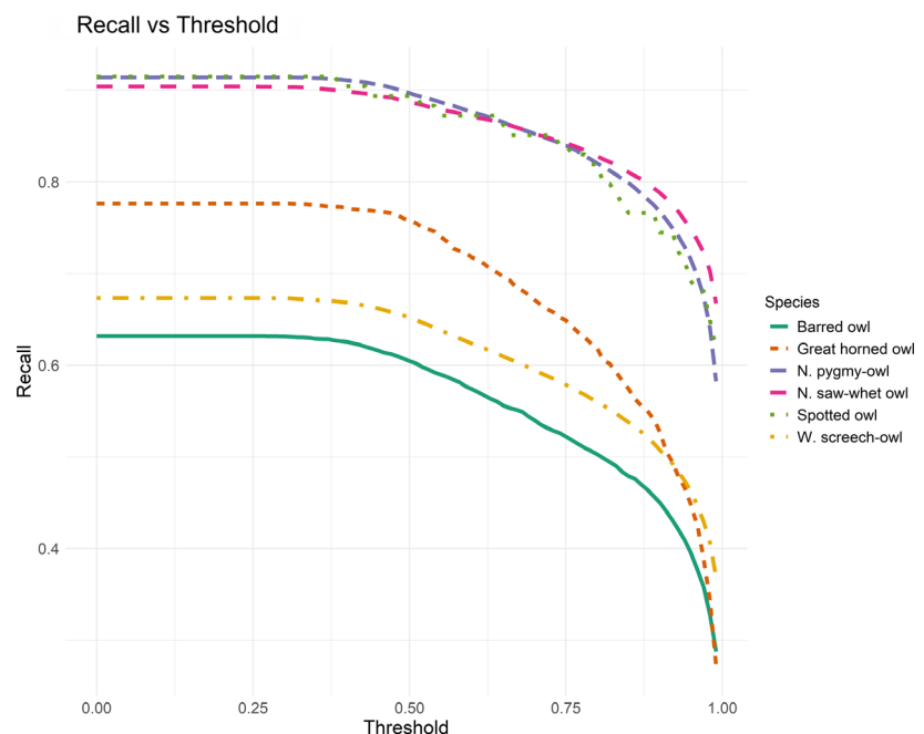
Figure 3. Recall vs threshold for six owl species. Recall is calculated as [\text{True Positives}]/[\text{True Positives} + \text{False Negatives}] , considering only clips with p_{\text{Max}} \geq \text{Threshold} , where p_{\text{Max}} is the maximum class score predicted by the convolutional neural network. Recall represents the proportion of target species calls present in the dataset that were detected and correctly labeled by the convolutional neural network.
