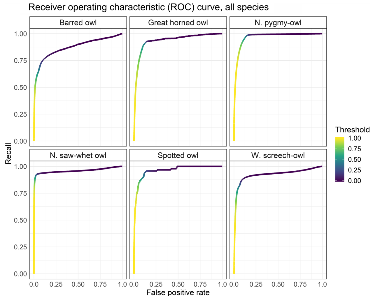
Figure 7. Receiver operating characteristic (ROC) curves for convolutional neural network classification of six owl species. The ROC curve plots the recall (AKA true positive rate) against the false positive rate. Recall is calculated as [\text{True Positives}] / [\text{True Positives} + \text{False Negatives}] . False positive rate is calculated as [\text{False Positives}] / [\text{False Positives} + \text{True Negatives}] . The area under the ROC curve (AUC) corresponds to the probability that the classifier will assign a higher score to a randomly chosen true positive than to a randomly chosen true negative. AUC values by species were: Barred owl, 0.872; Great horned owl, 0.934; Northern pygmy-owl, 0.967; Northern saw-whet owl, 0.959; Spotted owl, 0.961; Western screech-owl = 0.922. ROC curves were generated using the PRROC package in R, which interpolates values across the full range of threshold values.
