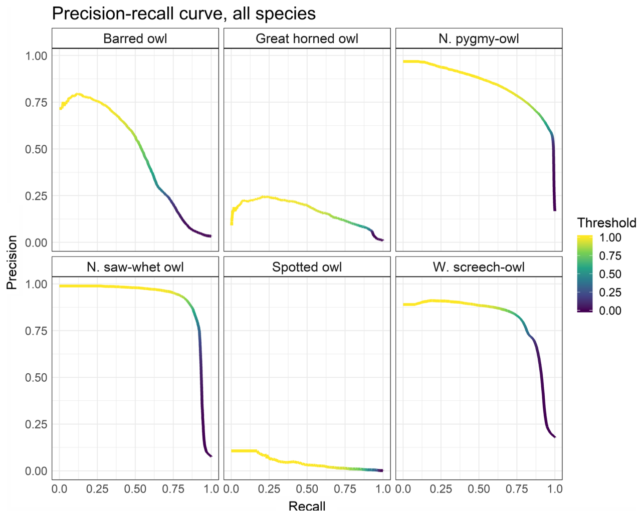
Figure 8. Precision-recall curves for convolutional neural network classification of six owl species. The precision-recall curve illustrates the tradeoff between sensitivity (recall) and specificity (precision). Area under the curve (AUC) serves as a general measure of model performance; a classifier with perfect precision and perfect recall would have AUC = 1 . AUC values by species were: Barred owl, 0.473; Great horned owl, 0.166; Northern pygmy-owl, 0.847; Northern saw-whet owl, 0.908; Spotted owl, 0.043; Western screech-owl, 0.807. Precision-recall curves were generated using the PRROC package in R, which interpolates values across the full range of threshold values.
