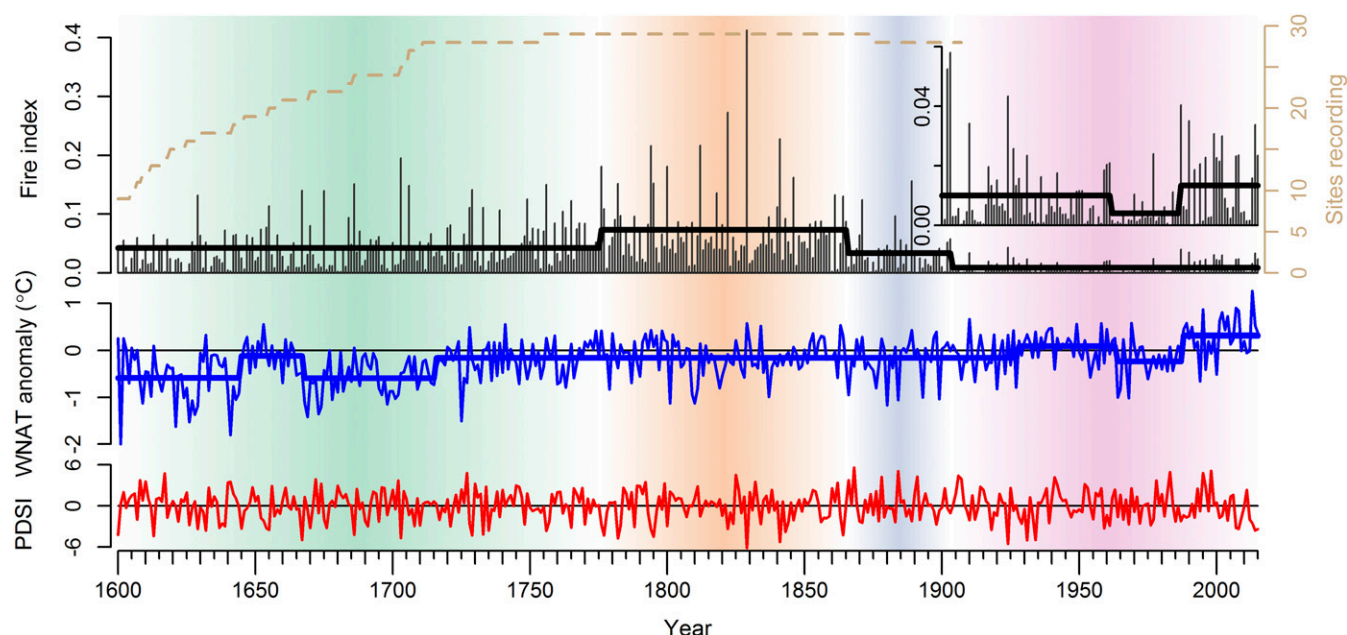
Fig. 2. Regime shifts in time series (1600–2015 CE) of Sierra Nevada fire index, summer moisture (i.e., PDSI) (60), and summer temperature (i.e., WNAT) (59). A switch to a new regime (fire or climate) is shown by a vertical line. The change point ( P < 0.05 ) was identified by using a 30-y window following Rodionov (58). A 15-y window and change point of P < 0.1 was used for the inset period (1900 to present). The number of tree-ring sites recording fires in each year for the 1600–1907 CE period is shown by the dashed line. The fire regime periods are indicated by color shading: 1600–1775 CE (green), 1776–1865 CE (orange), 1866–1903 CE (blue), and 1904 CE to present (pink).
