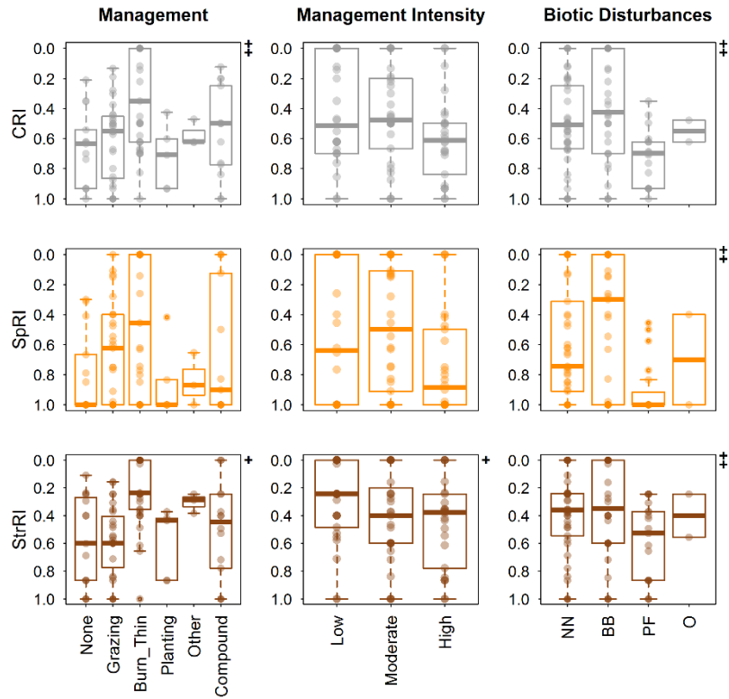
Fig. S8. Replacement patterns in relation to management, management intensity, and biotic disturbances within the 131 field sites included in our analysis. From top to bottom, CRI – joint compositional and structural resemblance index, SpRI – compositional resemblance index, StrRI – structural resemblance index are displayed. CRI corresponds to a measure of community resemblance of the pre-drought and post-drought vegetation in terms of composition and structure, computed as the mean of dissimilarity indices of composition (SpRI) and structure (StrRI). Compositional and structural indices were computed by means of the functions ‘vegdist’ and ‘vegdiststruct’ of the R packages vegan (52) and vegclust (51). In all cases, 0 indicates no change and 1 indicates complete change. Please see Methods description in the main text for additional details about assessment of composition and structural differences.
