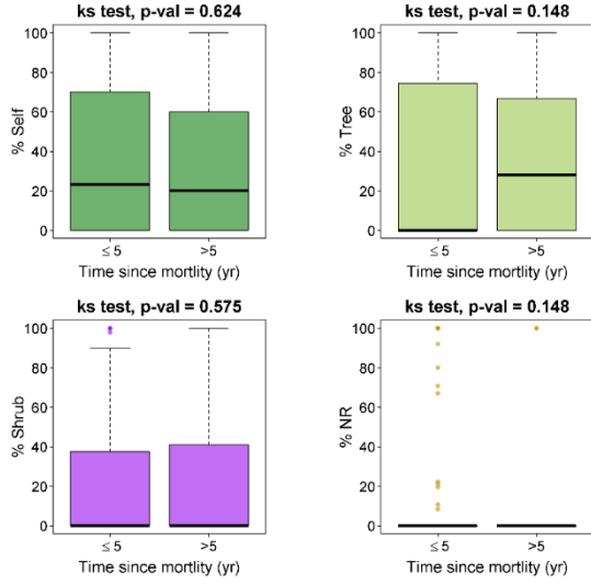
Fig. S3. Replacement patterns in relation to (a) 'recovery time' or the lag between the observed mortality and sampling time and (b) the successional state (Dataset D1 and D3) of the assessed forest and woodlands. In (a) boxplots display the proportion of: '%Self' - self-replacement (i.e., replacement of dominant tree species with itself), '%Tree' and '%Shrub' - replacement by other woody species including trees and shrubs, respectively, or '%NR' - lack of replacement by woody vegetation in sites sampled \leq 5 years and > 5 years after drought-induced tree mortality. In (b) boxplots display the proportion of: '%Self', '%Tree', '%Shrub', and '%NR' in sites within Early, Mid or Late successional state, that is whether forests are in compositional equilibrium and represent stable, self-reproducing populations (i.e., late) or transitional forests types (i.e., early, mid). The significance of Kruskal-Wallis rank sum tests is presented for each case, indicating that no significant differences exist among the groups of study sites.
