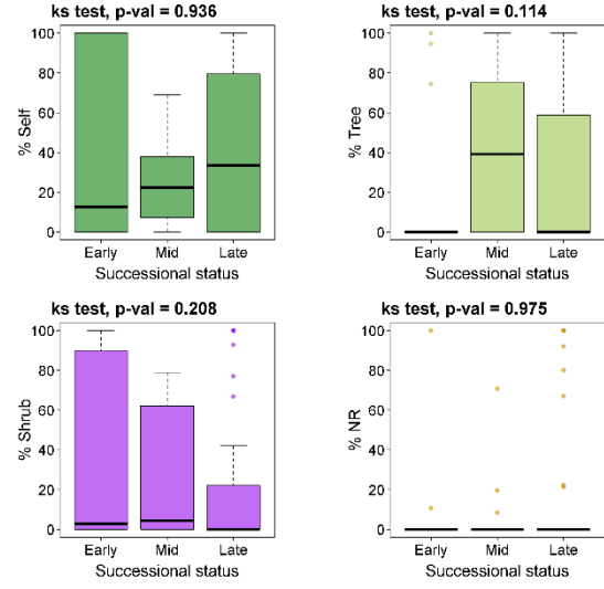
Fig. S3. Replacement patterns in relation to (a) 'recovery time' or the lag between the observed mortality and sampling time and (b) the successional state (Dataset D1 and D3) of the assessed forest and woodlands. In (a) boxplots display the proportion of: '%Self' - self-replacement (i.e., replacement of dominant tree species with itself), '%Tree' and '%Shrub' - replacement by other woody species including trees and shrubs, respectively, or '%NR' - lack of replacement by woody vegetation in sites sampled \leq 5 years and > 5 years after drought-induced tree mortality. In (b) boxplots display the proportion of: '%Self', '%Tree', '%Shrub', and '%NR' in sites within Early, Mid or Late successional state, that is whether forests are in compositional equilibrium and represent stable, self-reproducing populations (i.e., late) or transitional forests types (i.e., early, mid). The significance of Kruskal-Wallis rank sum tests is presented for each case, indicating that no significant differences exist among the groups of study sites.
