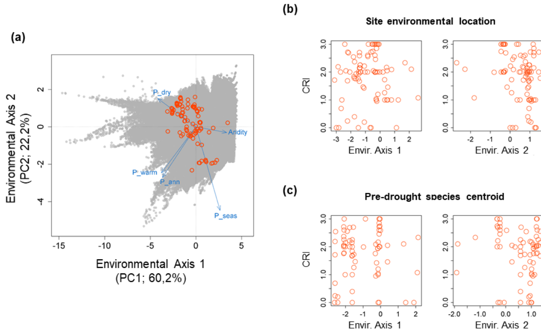
Fig. S4. (a) Environmental space used to characterize the bioclimatic characteristics of the species and reporting sites. Each grey dot corresponds to all 10 \times 10 km pixels within the forested biomes included in our analysis (see Fig. 1 within the main text) and the orange circles depict the field sites included in our analyses. Right panels show replacement patterns, characterized by means of the joint compositional and structural community resemblance index CRI, in relation to (b) the bioclimatic characteristics of the study sites and (c) the environmental centroids of the dominant (pre-drought) species at each site. The environmental space (a) was defined through Principal Component Analysis (PCA) on the basis of four precipitation regime variables plus the aridity index at the global scale (excluding species-rich tropical biomes, following Olson et al. 2001 biome classification; Bioscience 51 , 933–938 (2001)); P_seas – precipitation seasonality, P_dry – precipitation of the driest quarter, P_warm – precipitation of the warmest quarter, P_ann – annual precipitation, and Aridity – Aridity Index expressed as 1- aridity. Precipitation data for baseline conditions were obtained from WorldClim Version 2.0 at a 10 \times 10 km resolution ( http://www.worldclim.org/ ) and the aridity index from CGIAR-CSI website ( http://www.cgiar-csi.org ). The bioclimatic optima or environmental centroids of all species within the study sites (orange circles) were defined as the density centroid (center of mass of the point distribution within the environmental space) of the 95% density distribution kernel of the species observations (i.e., presence data) as obtained from the Global Biodiversity Information Facility (GBIF; https://www.gbif.org/ ). In (b) mapped PCA loadings represented in graph (a) were used to extract the principal components PC1 and PC2 values at the x-y coordinates of the sites. In (c) the environmental centroid of each site was computed as the weighted mean (based on species abundance) of the environmental centroids of the dominant (pre-drought) tree species.
