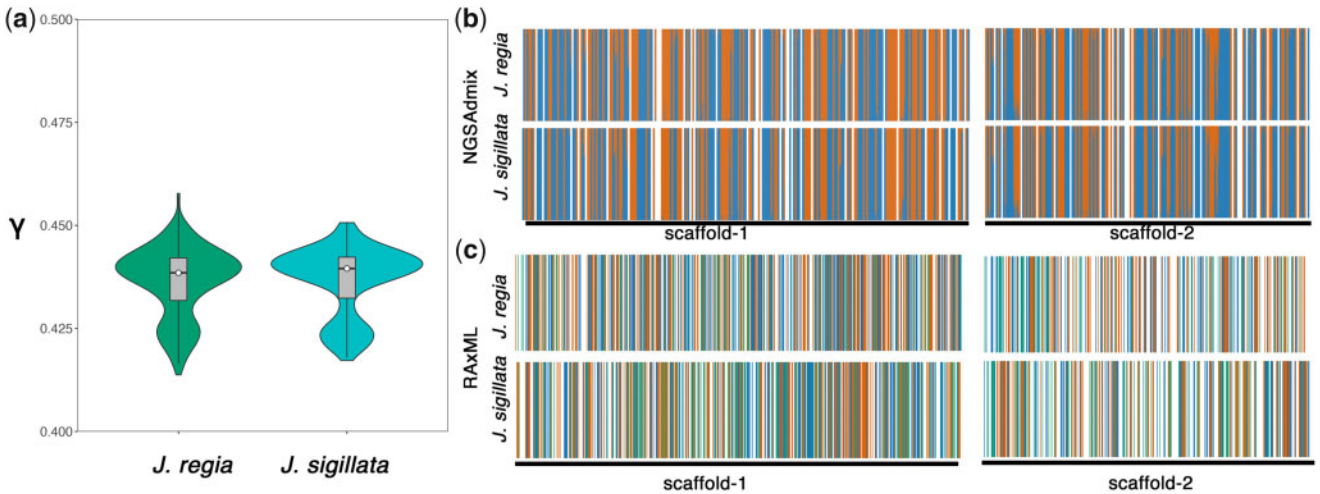
FIG. 3. HyDe individual test and stepping-windows admixture and phylogenetic analyses for Juglans regia and J. sigillata . (a) Violin plots of the distribution of \gamma with HyDe for six individuals of J. regia and five individuals of J. sigillata . \gamma indicates the inheritance probabilities from the parental species of sect. Cardiocaryon to the inferred individual. (b) Results of the NGSADMIX-analysis assignments for 10-kb nonoverlapping windows across scaffolds 1 and 2 of J. regia and J. sigillata . The windows show J. regia windows clustering with J. mandshurica in red, J. regia windows clustering with J. nigra in blue, and J. regia clustering by itself in white. (c) RAXML analysis on 10-kb windows depicting whether J. regia or J. sigillata grouped monophyletically with J. mandshurica (red), J. nigra (blue), formed their own clade (green), or remained unresolved (white).
