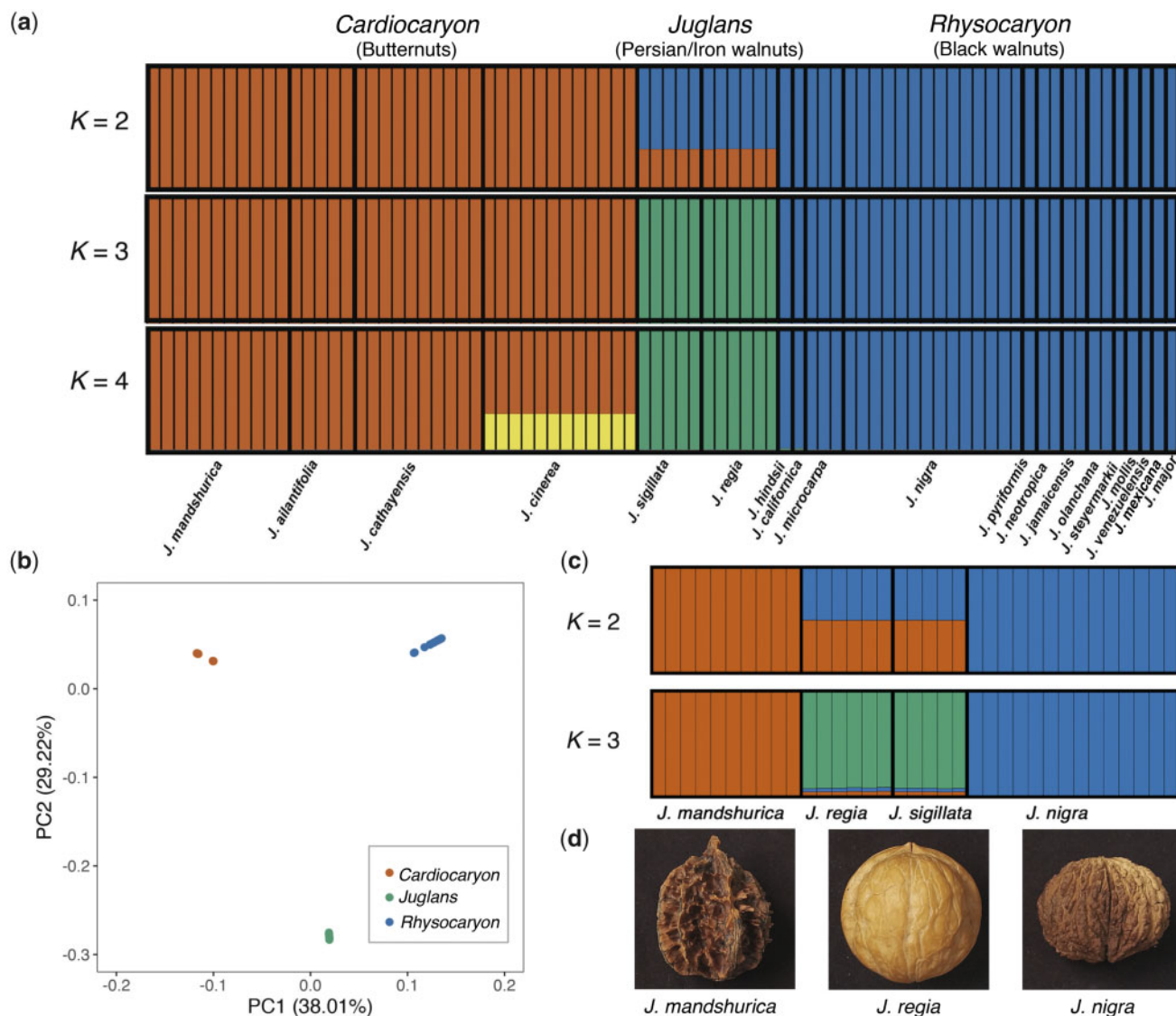
Fig. 1. Population structure based on independent nonmissing SNPs. (a) Results of STRUCTURE analyses of 80 individuals of Juglans . (b) PCA of the same 80 individuals. (c) Assignment probabilities for Juglans regia and J. sigillata individuals in STRUCTURE analyses when using population information of J. mandshurica and J. nigra . (d) Nut photos of J. mandshurica , J. nigra , and J. regia .
