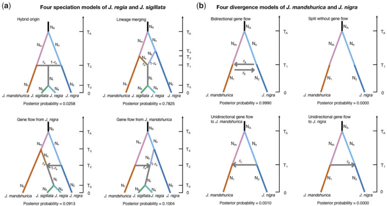
Fig. 4. ABC models and their corresponding posterior probabilities for the origin of Juglans regia and J. sigillata (a) and models for the divergence of J. mandshurica and J. nigra (b). The posterior probability of each model was estimated with logistic regression using 1% of simulated data closest to the observed data set in the model selection procedure.
