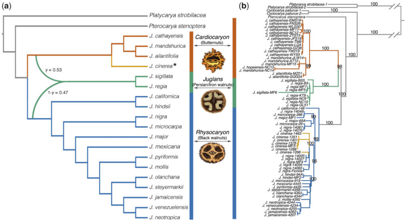
FIG. 2. Species network inference and chloroplast phylogeny. (a) Optimal species network inferred using the PhyloNet software. The result is maximum pseudo-likelihood tree with one reticulation. The \gamma value indicates the inheritance probability from the ancestor of sect. Cardiocaryon , whereas 1 - \gamma indicates that from the ancestor of sect. Rhysocaryon . (b) A ML phylogeny from 68 entire plastid genomes of Juglans and two outgroups, with bootstrap support values \geq 96 above branches. The asterisk marking Juglans cinerea refers to the only case of phylogenomic discord between the nuclear and plastid topologies (see Discussion).
