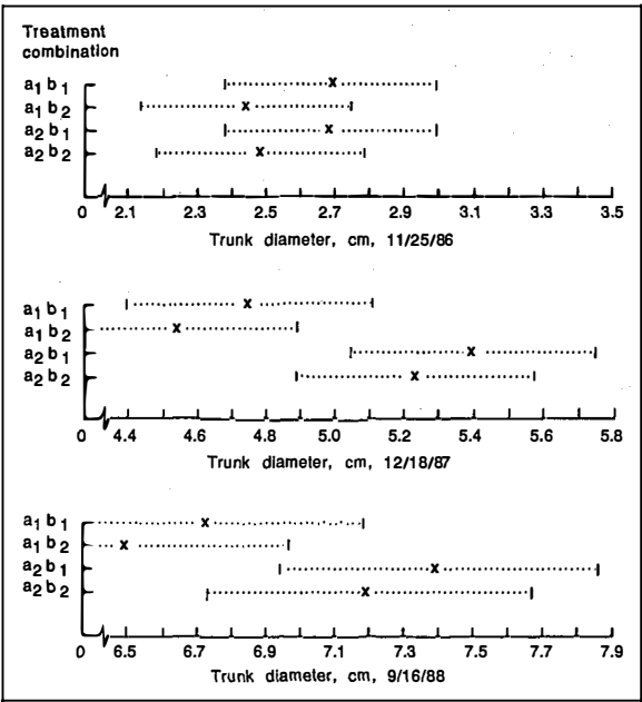
Figure 6. Simultaneous 95% confidence intervals, with Bonferroni adjustment, for trunk diameters based on pooled standard deviations for southwestern black cherry trees for each of four factorial treatment combinations (a 1 b 1 , 35-cm rootball without casing; a 1 b 2 , 35-cm rootball with casing; a 2 b 1 , 70-cm rootball without casing; a 2 b 2 , 70-cm rootball with casing) at the end of growing seasons 1986, 1987, and 1988.
