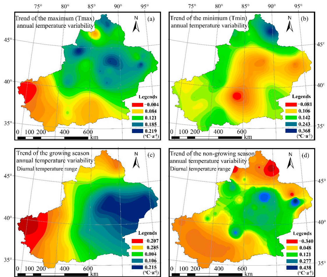
Figure 5. The spatial distribution of averaged T_{\max} and T_{\min} over 20 years in the arid and semiarid region, (a): the trend of T_{\max} , (b): the trend of T_{\min} , (c): diurnal range in the growing season of vegetations, (d): diurnal range in the non-growing season of vegetations. S1 and S2 represent two regions of the study area.
