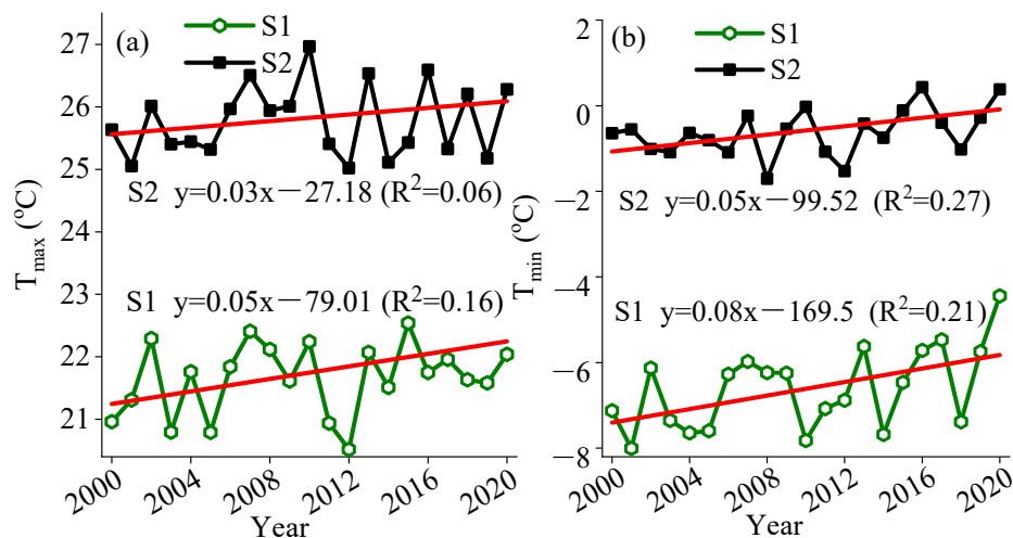
Figure 2. T_{\max} (a) and T_{\min} (b) trends in the S1 and S2 regions with arid and semiarid climate, 2000–2020.
