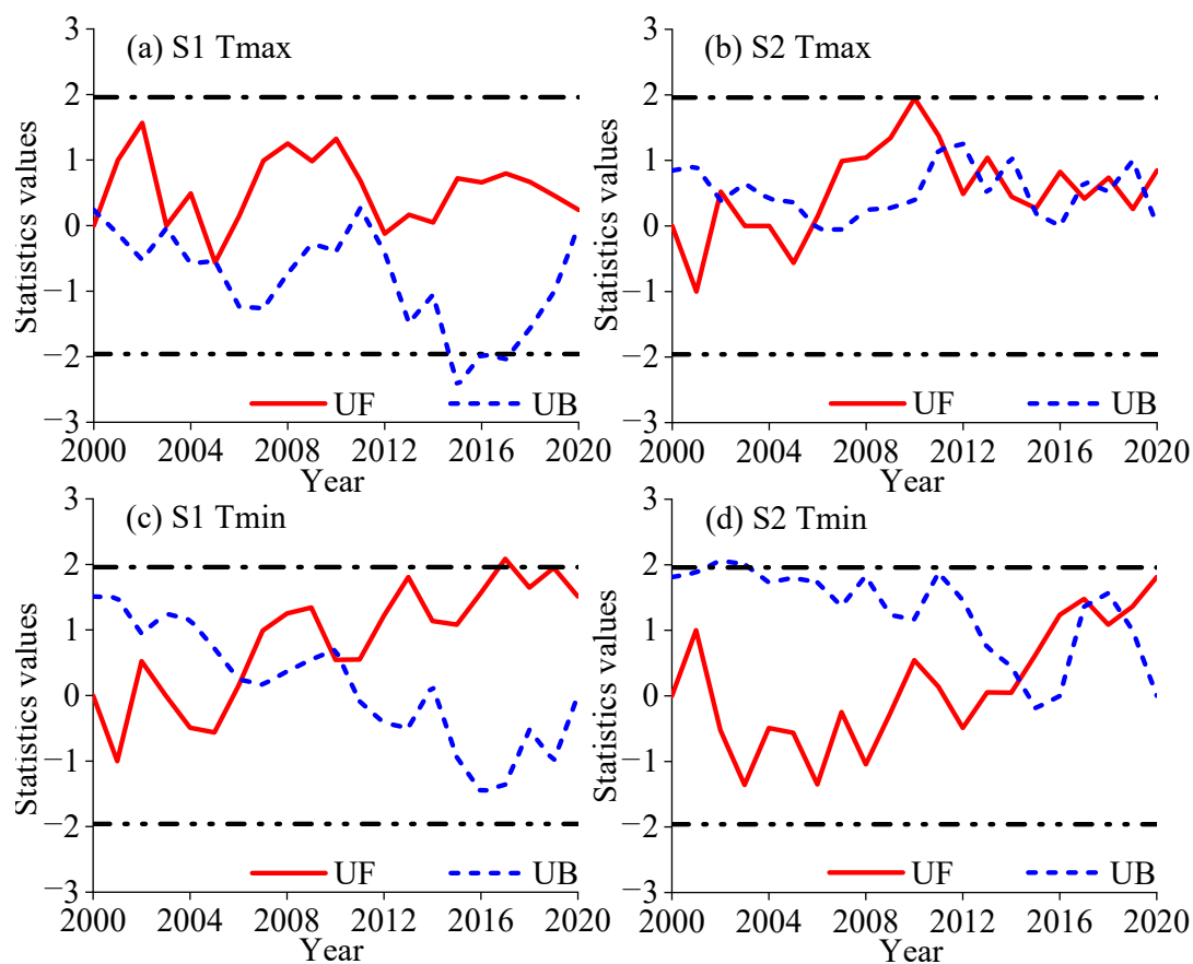
Figure 7. Mann–Kendall test for monotonic trend of (a) T_{\max} over S1 region, (b) T_{\max} over S2 region, (c) T_{\min} over S1 region, and (d) T_{\min} over S2 region. S1 and S2 represent two regions of the study area, UF and UB are statistics about temperature series, which obeys standard normal distribution. If UF and UB intersect, they represent the start time of an abrupt change.
