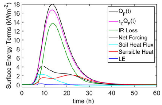
Figure 5. Soil surface energy balance components for the 26 April 2004 MEF burn resulting from the full surface energy balance model (Eq. 16). The parameters for the forcing function, Q_F(t) or Eq. (15), are Q_{in} = 120 \text{ W m}^{-2} , Q_{Fmax} = 18 \text{ kW m}^{-2} , t_m = 13.5 \text{ h} and t_d = 35 \text{ h} . The net forcing is defined as the difference between the radiative terms, i.e., \epsilon_0(\theta_0) Q_F(t) - \epsilon_0(\theta_0) \sigma [T_{K0}^4 - \epsilon_a(\rho_{va}) T_{Ka}^4] , which, from Eq. (16), is equal to the sum of the three nonradiative terms, i.e., \rho_a c_p a C_H [T_0 - T_a] + L_{v0}^* E_0 + G_0 . Figure 6 is an magnified version of the net forcing and these three energy components.
