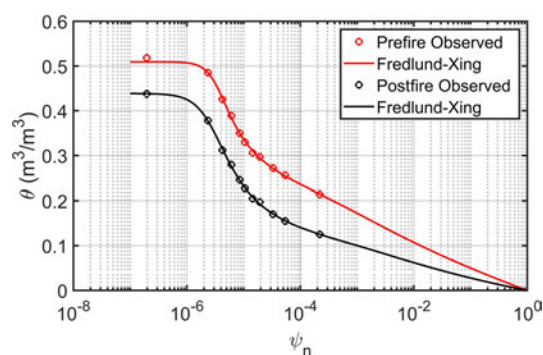
Figure 1. Pre- and postburn water retention curves at the 2004 Manitou Experimental Forest (MEF) burn site. Observations were fitted with the Fredlund and Xing (1994) model. The only difference between these two curves is that the total or air-filled porosity is about 0.51 for the preburn (red), and it is about 0.45 for the postburn (black).
