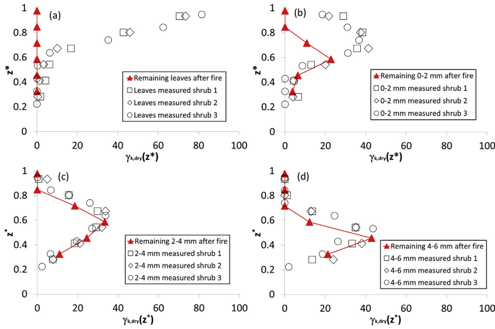
Fig. 8. Characterization of the fuel consumption at particle level: comparison of the mass fraction before (from the destructive measurements of 3 shrub samples) and after the burning (fire test 15), for the different particles size classes: (a) leaves, (b) twigs of 0–2 mm diameter, (c) twigs of 2–4 mm diameter and (d) twigs of 4–6 mm diameter.
