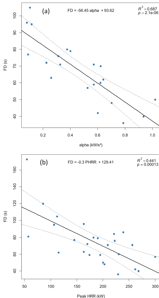
Fig. 7. Relationship between sustainability and combustibility (a) Flame duration FD (s) versus fire growth parameter \alpha ( \text{kW}\cdot\text{s}^{-2} ) and (b) Flame duration FD (s) versus peak HRR (kW).
