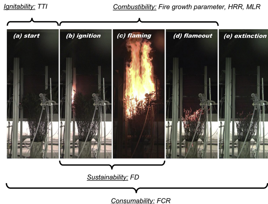
Fig. 3. Measurements of the 4 components of flammability during the different combustion process phases: (a) test start, (b) ignition, (c) flaming, (d) flameout and char oxidation, (e) extinction.
