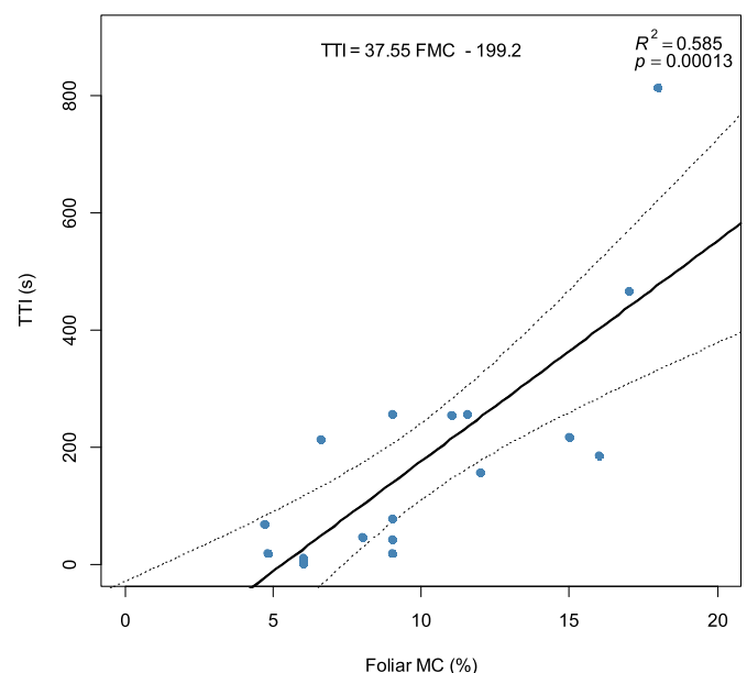
Fig. 4. Influence of foliar MC on ignitability.
