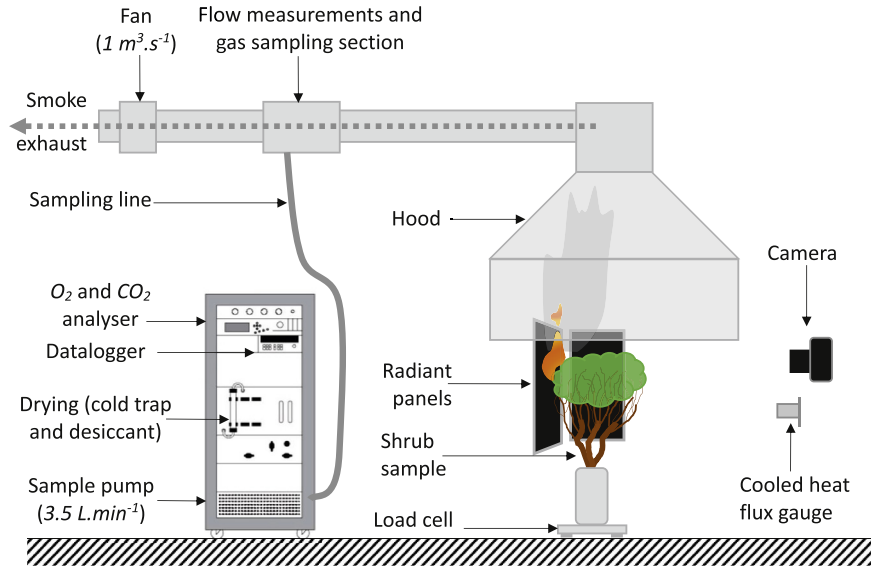
Fig. 1. Layout of the experimental setup.
