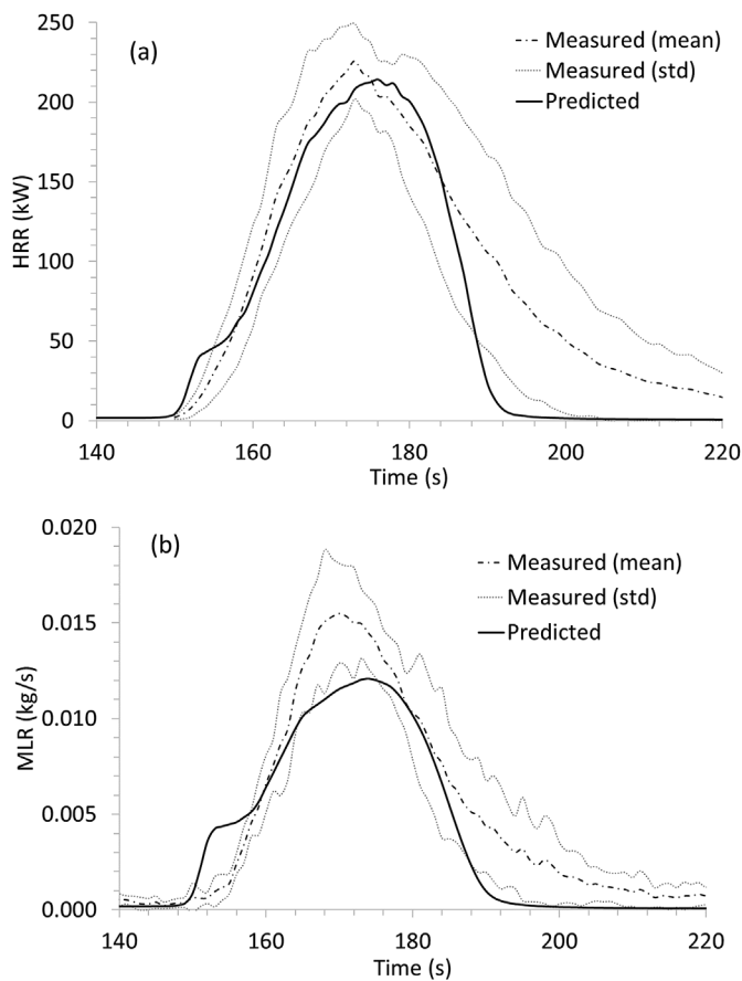
Fig. 12. Comparison of the predictions and measurements (a) HRR and (b) MLR. The experimental data are obtained from the mean (and standard deviation) of 5 fire tests corresponding to the high flammability with low sustainability regime.
