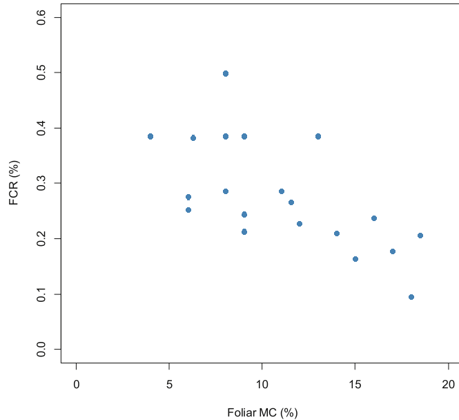
Fig. 9. Fuel consumption ratio versus foliar moisture content.
