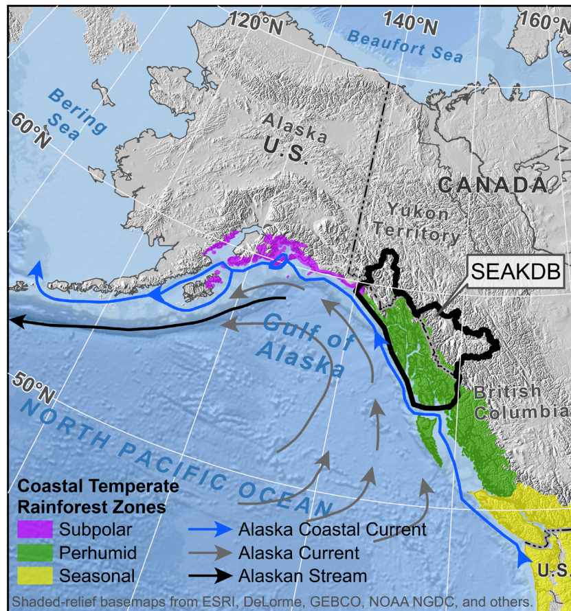
Figure 1. Location of the SEAKDB, coastal temperate rainforest zones, and Gulf of Alaska ocean currents. Source: ocean currents adapted with permission from Weingartner et al. (2005). Rainforest zones adapted with permission from vector data set “CTRF” by Ecotrust, Pacific GIS, and Conservation International, and Wolf et al. (1995).
