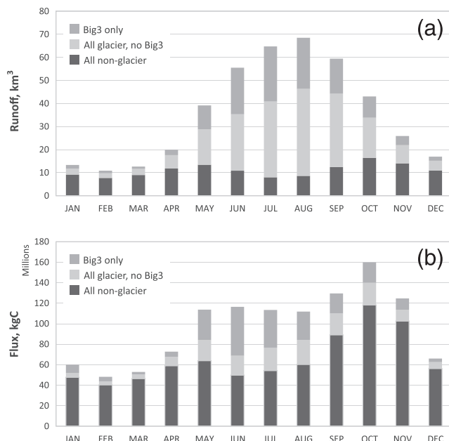
Figure 4. Monthly distribution of (a) mean freshwater discharge and (b) DOC flux from the SEAKDB watersheds.
