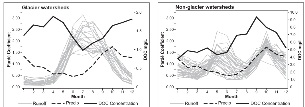
Figure 3. Mean monthly runoff, precipitation, and DOC concentration for glacier and nonglacier watersheds. Runoff and precipitation are normalized as Pardé coefficients (mean monthly discharge divided by mean annual discharge, times 12). Compared to glacier watersheds, freshwater discharge from nonglacier watersheds is higher in the winter, much lower in the summer, and either closely mimics the precipitation hydrograph, or generally follows the precipitation hydrograph but has an additional spring snowmelt peak. Glacier watersheds discharge a much higher proportion of their annual flow beginning in midspring and through summer and store significantly more precipitation over the winter. Precipitation source: PRISM mean monthly precipitation, 1981–2010 (Pacific Climate Impacts Consortium, University of Victoria, and PRISM Climate Group, Oregon State University, 2014).
