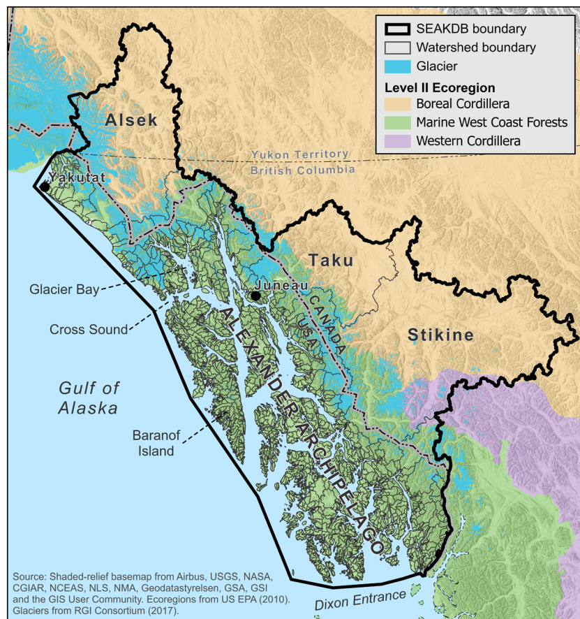
Figure 2. SEAKDB watersheds and area geography.
