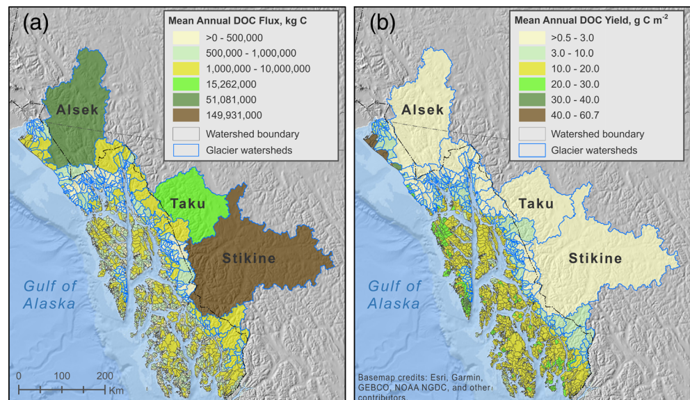
Figure 6. Distribution of mean annual DOC flux (a) and DOC yield (b) from SEAKDB watersheds.
