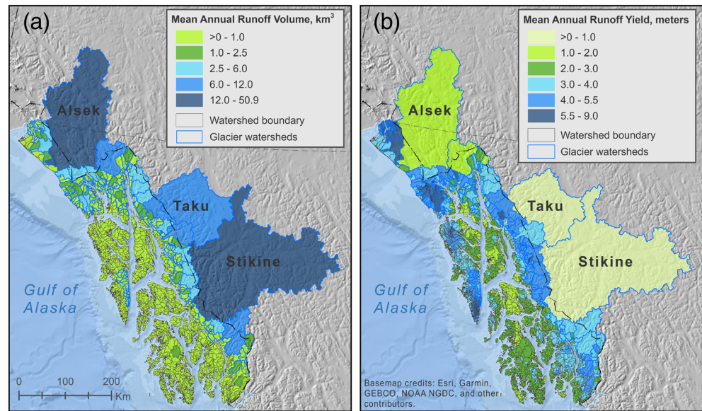
Figure 5. Distribution of mean annual freshwater runoff volume (a) and yield (b) from SEAKDB watersheds.
