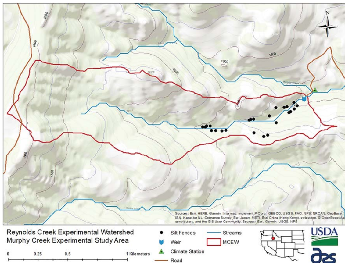
Figure 1. Map of the Murphy Creek Experimental Watershed (43° 15' 20.2" N latitude, 116° 49' 10.3" W longitude, 1390 m MSL) study area and instrumentation (silt fences, weir, and climate station) located along the South Fork of Murphy Creek and upslope of the Murphy Creek Weir in the Reynolds Creek Experimental Watershed, administered by the US Department of Agriculture (USDA), Agricultural Research Service (ARS), Northwest Watershed Research Center, in southwestern Idaho, USA.
