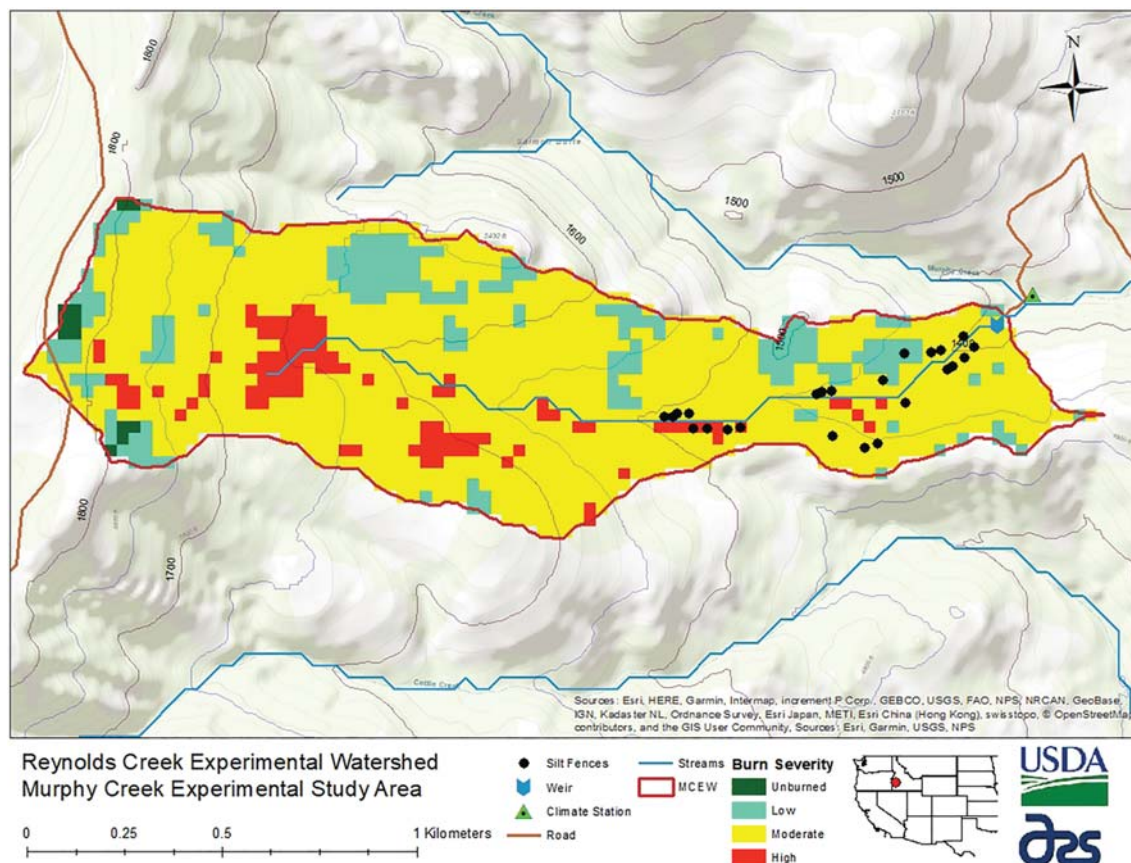
Figure 3. Map of burn severity and experimental instrumentation in the Murphy Creek Experimental Watershed immediately after the 2015 Soda Fire, as derived from burned area reflectance classification data (BARC) by the US Department of Interior, available online from the US Department of Agriculture (USDA) Geospatial Technology and Applications Center at: https://www.fs.fed.us/eng/rsac/baer/baer_request.html
