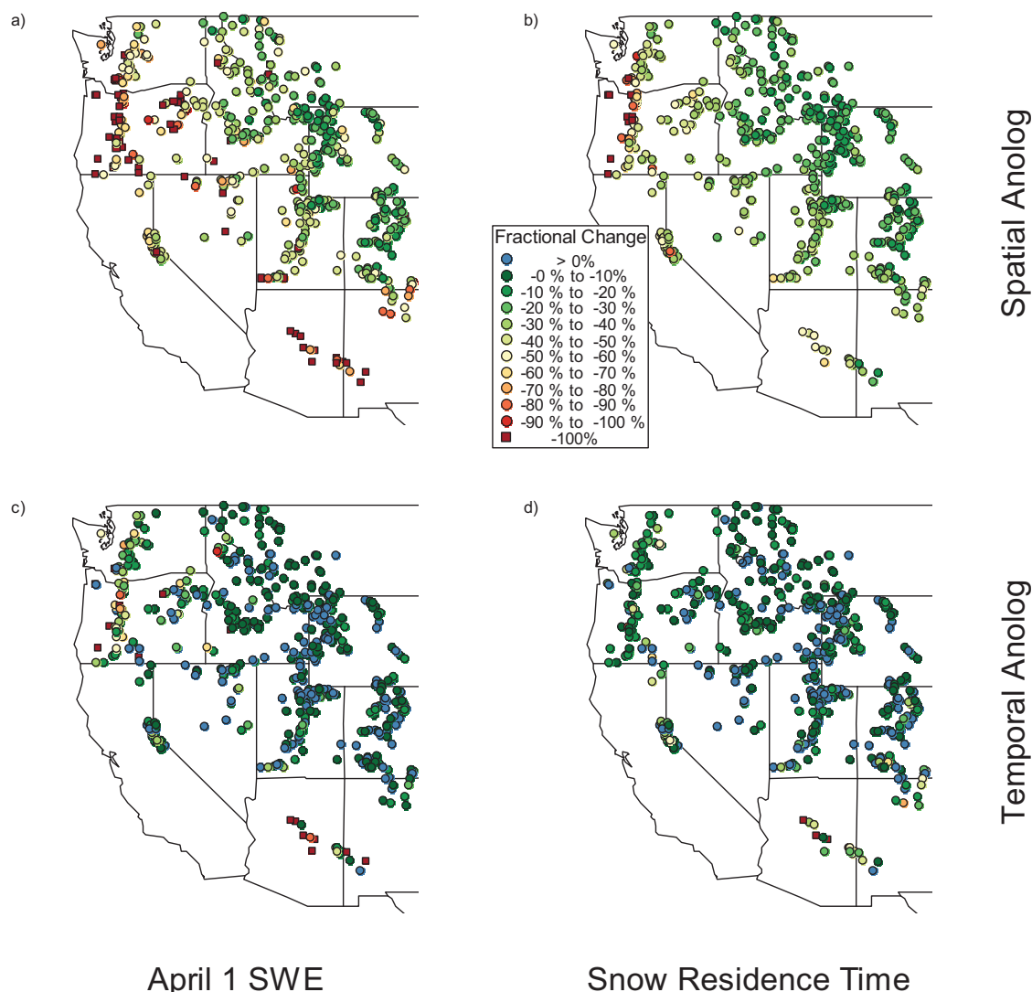
Figure 11. Comparison of fractional declines derived from spatial (a and b) versus temporal (c and d) analogs considering a 3^{\circ}\text{C} increase in winter average temperature at each SNOTEL station. Left hand (a and c) maps are for April 1 SWE and right hand (b and d) maps are for mean snow residence time (SRT). Blue points denote projected increases.
