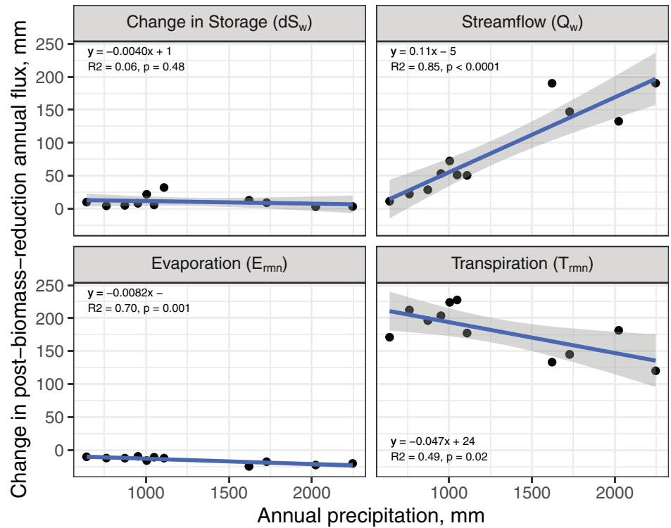
FIGURE 5 Relation between annual precipitation (mm) and post-biomass reduction annual flux change (mm) for the 50% biomass-reduction scenario averaged over all watersheds. Each point represents one water year. Blue line shows the calculated linear relation, and the shaded grey signifies the 95% uncertainty intervals
