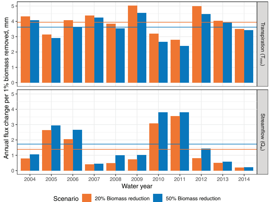
FIGURE 6 Increase in annual streamflow and transpiration flux from the remaining vegetation per 1% biomass removed increment for 20% and 50% biomass-reduction scenarios averaged over all watersheds. Horizontal lines indicate the mean annual flux change across all water years
