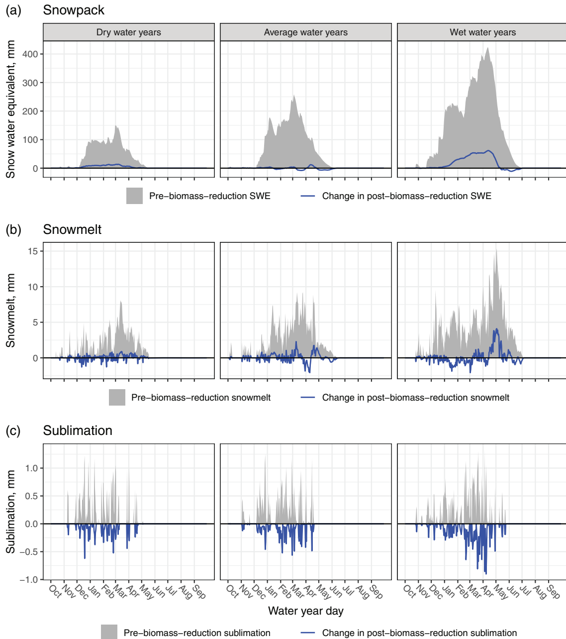
FIGURE 8 Mean daily pre-biomass-reduction (a) snow water equivalent (SWE), (b) snowmelt, and (c) sublimation, as well as changes in the respective post-biomass-reduction quantities averaged for the three driest, four average, and four wettest water years in the P303 watershed for the 50% biomass-reduction scenario
