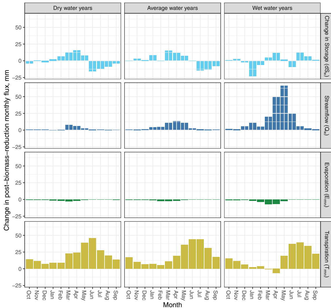
FIGURE 7 Change in mean monthly post-biomass-reduction storage, streamflow, evaporation, and transpiration; averaged for the three driest, four average, and four wettest water years in the P303 watershed for the 50% biomass-reduction scenario
