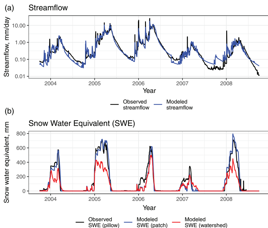
FIGURE 2 RHESSys calibration time-series for water years 2004 to 2008.
