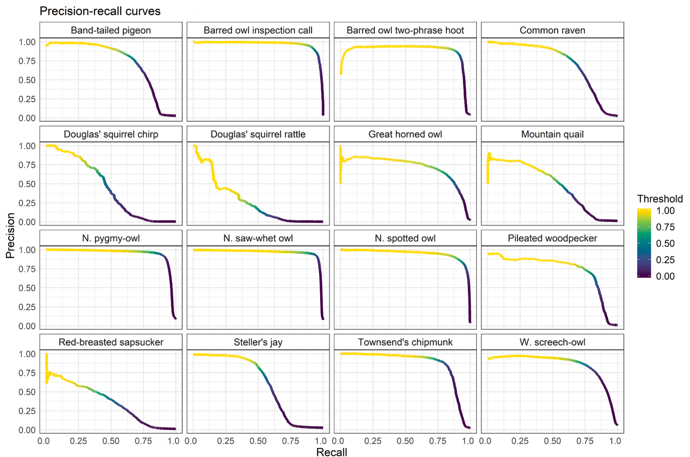
Fig. 7. Precision-recall curves for 16 sounds produced by 14 avian and mammalian species. The precision-recall curve plots precision (True positives/[True Positives + False Positives]) against recall (True Positives/[True Positives + False Negatives]) to illustrate a given model's performance and the magnitude of the trade-off between these metrics across a range of detection thresholds.
