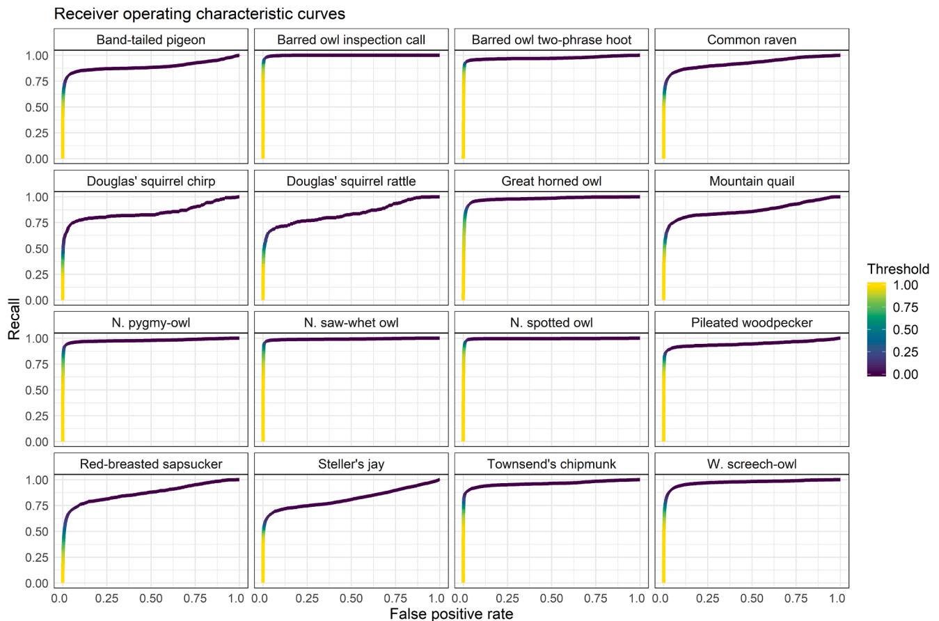
Fig. 6. Receiver operating characteristic curves for 16 sounds produced by 14 avian and mammalian species. The receiver operating characteristic curve plots the true positive rate (recall), calculated as [\text{True Positives}] / [\text{True Positives} + \text{False Negatives}] against the false positive rate, calculated as [\text{False Positives}] / [\text{False Positives} + \text{True Negatives}] .
