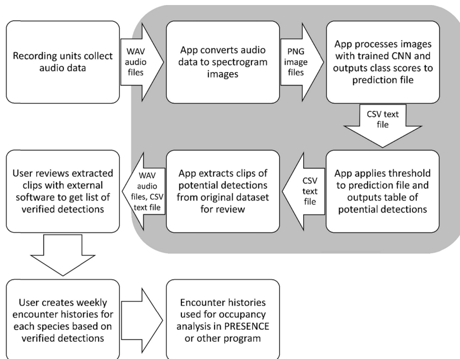
Fig. 2. Diagram of steps involved in audio processing and target species detection workflow. Processing steps in the shaded region can be performed using the desktop application provided, while those outside must be performed using external software or equipment. Arrows between boxes indicate the type and format of the data that are produced during each step and passed to the next step.
