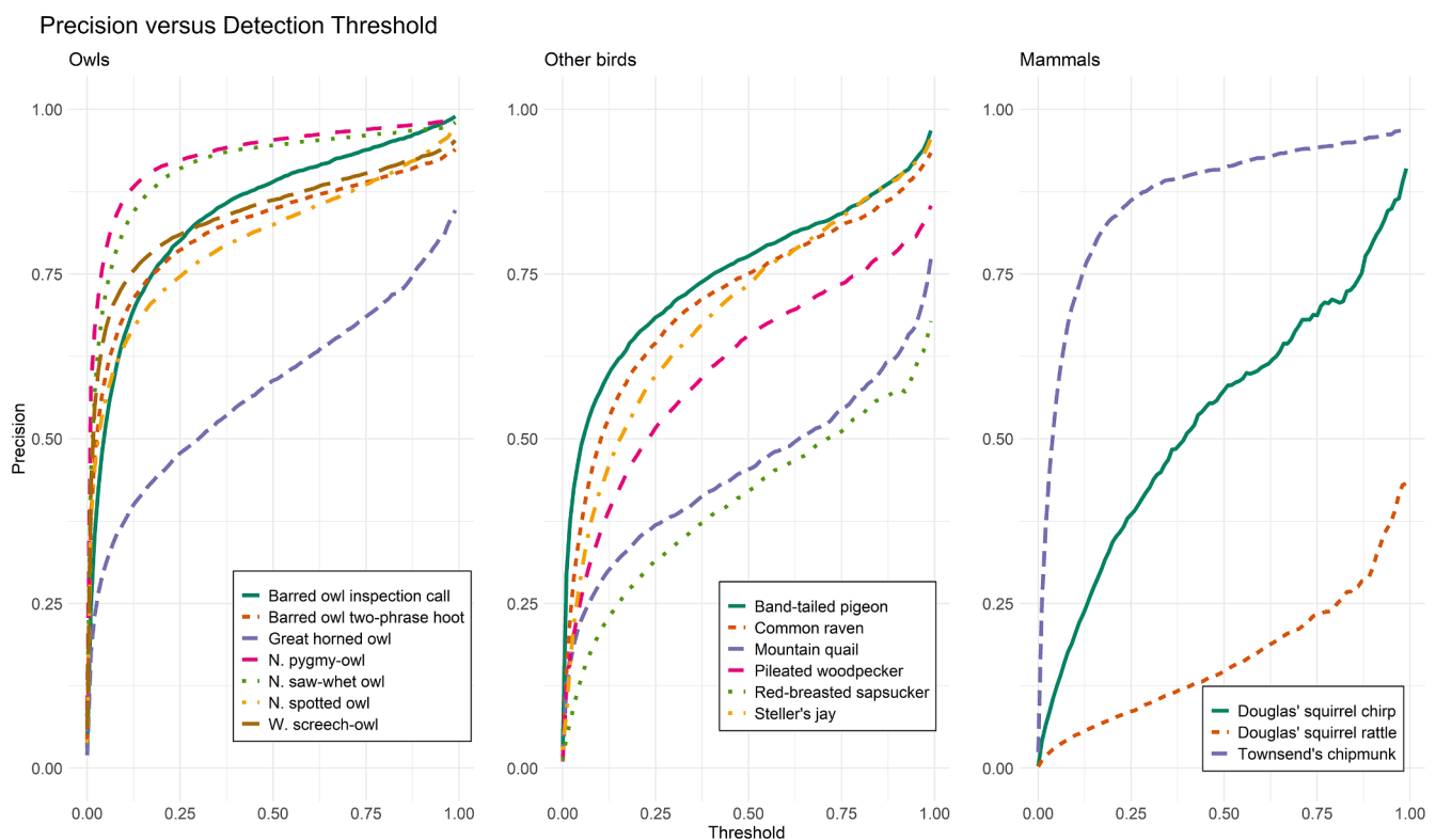
Fig. 3. Precision versus detection threshold for 16 sounds produced by 14 avian and mammalian species. Precision or specificity is calculated as [\text{True Positives}] / [\text{True Positives} + \text{False Positives}] , considering only clips with class score exceeding the detection threshold for each target class. Precision represents the proportion of apparent “hits” that correspond to real instances of the class in question.
