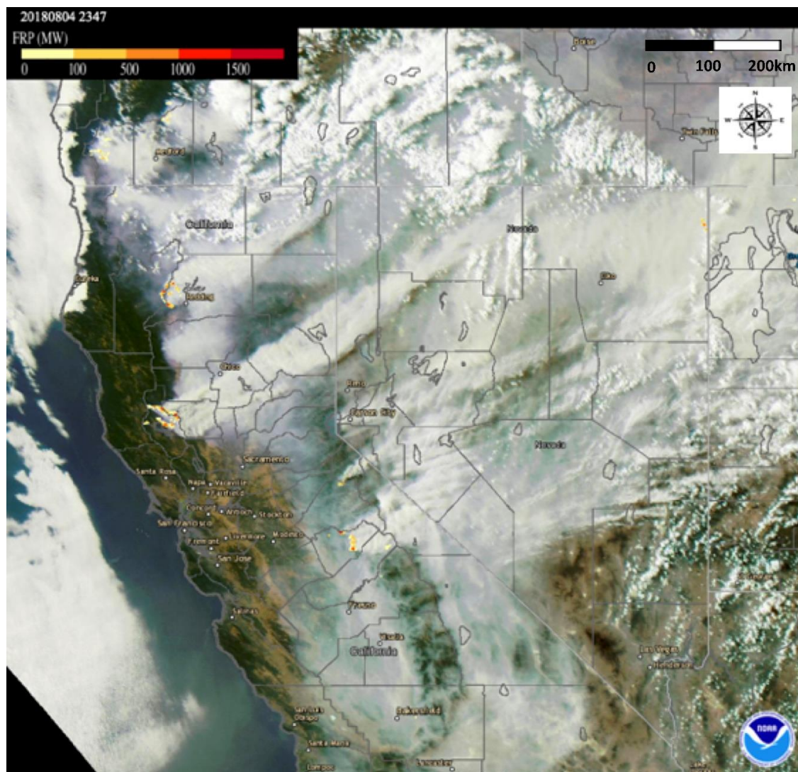
Figure 1. Visible smoke plume from the GOES-16 satellite at 2347 UTC and fire radiative power from the VIIRS instrument aboard Suomi-NPP on August 4 2018. Image from NOAA AerosolWatch.
