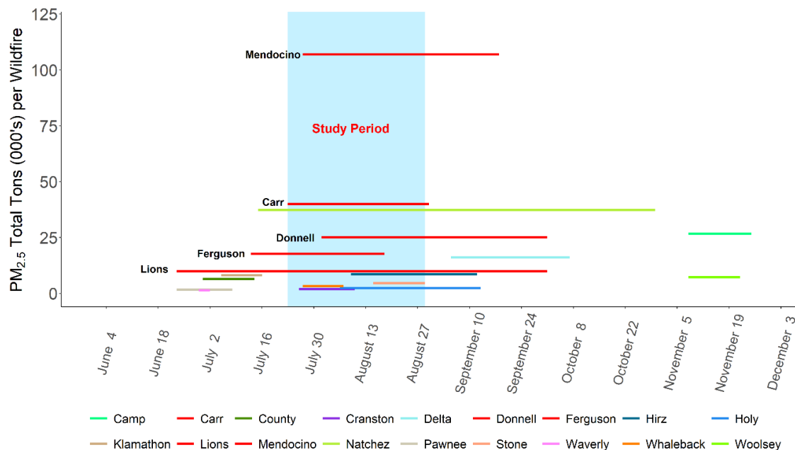
Figure 3. Estimated total emissions ( \text{PM}_{2.5} total tons per wildfire) and the active time of fire spread per fire between 4 June and 3 December 2018, for 18 fires. Fires included in this study have red lines. The study period (time period in which smoke apportionment modeling was performed) is shaded in light blue.
