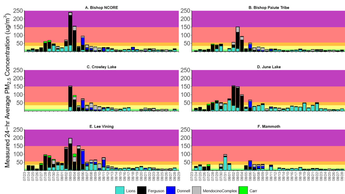
Figure 4. Apportionment of measured 24 h average \text{PM}_{2.5} concentration, 23 July–29 August 2018 by fire (Lions, Ferguson, Donnell, Mendocino Complex, Carr) at each of the six monitoring sites (Bishop NCORE, Bishop Paiute Tribe, Crowley Lake, June Lake, Lee Vining, Mammoth). Background color indicates U.S. Environmental Protection Agency (EPA) Air Quality Index (AQI) category; Green: Good, Yellow: Moderate, Orange: Unhealthy for Sensitive Groups, Red: Unhealthy, and Purple: Very Unhealthy.
