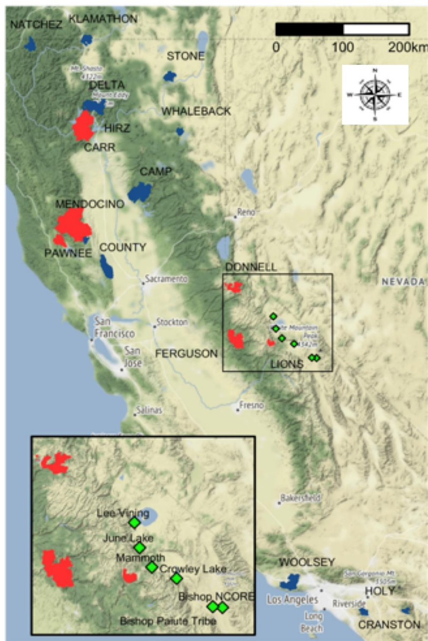
Figure 2. Location of wildland fires greater than 12,000 acres in California in 2018. Red fill: Fires included in this study; green diamonds: The six air quality monitoring sites. Source: United States Department of Agriculture, Forest Service.
