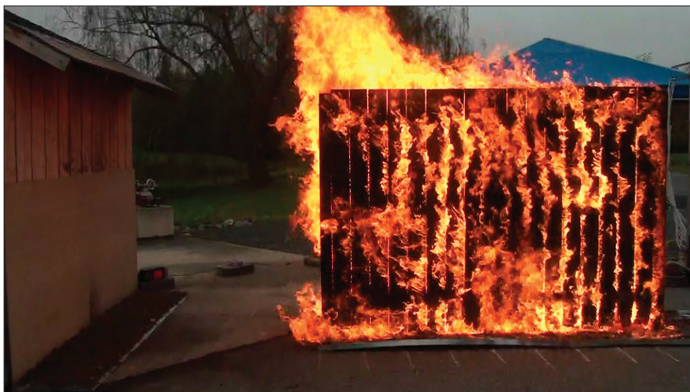
Figure 13 —Parallel western redcedar privacy fences separated by 0.20 m in hardwood mulch at low wind speed ( 6 \text{ m second}^{-1} ).
