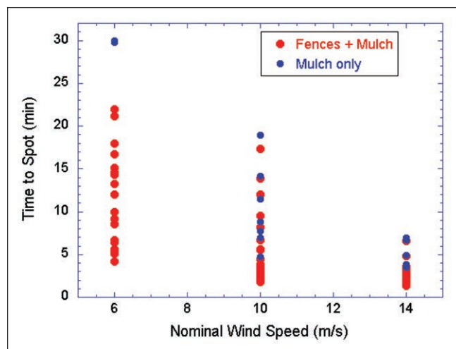
Figure 5 —Spotting time as a function of nominal wind speed for experiments on mulch beds only (blue) and combinations of fence and mulch bed (red).
