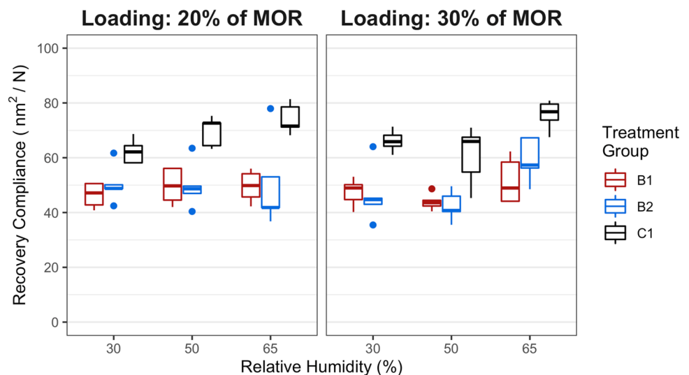
Fig. 3 Recovery compliance as a function of relative humidity and loading level ( n=5 ). The box and whiskers plots represent the distribution of the data, where the lower and upper bounds of the box mark the 25th and 75th percentile of the data, the center bar is at the median of the data set, the whiskers extend to the minimum and maximum of the data set excluding outliers , and the circles represent outliers
