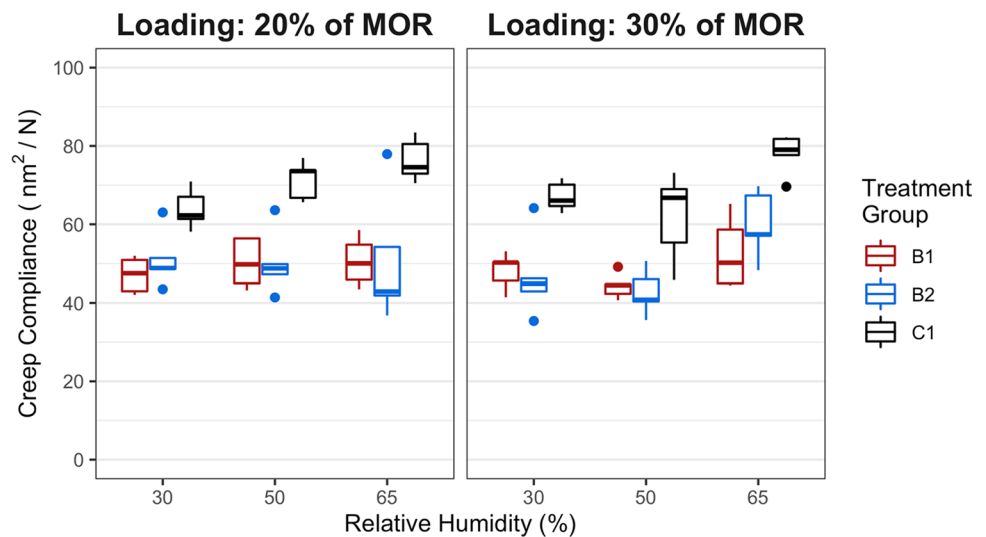
Fig. 2 Creep compliance as a function of relative humidity and loading level ( n=5 ). The box and whisker plots represent the distribution of the data, where the lower and upper bounds of the box mark the 25th and 75th percentile of the data, the center bar is at the median of the data set, the whiskers extend to the minimum and maximum of the data set excluding outliers , and the circles represent outliers
