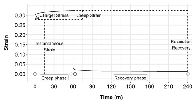
Fig. 1 Experimental creep data highlighting key parameters
