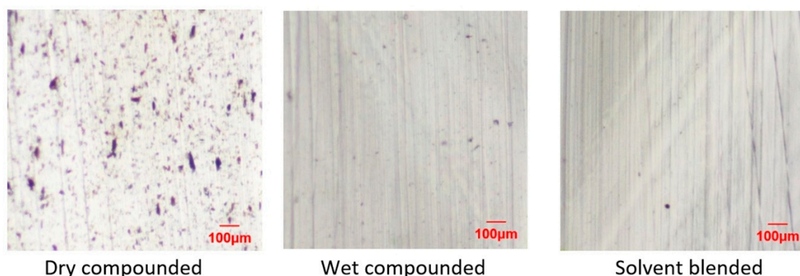
Figure 7. Microscope images of sections of PA6-CNC composites prepared by dry compounding of freeze-dried CNCs, wet compounding of CNC dispersion, and solvent blending in formic acid [8]. All composites contain 5% CNC by weight.
