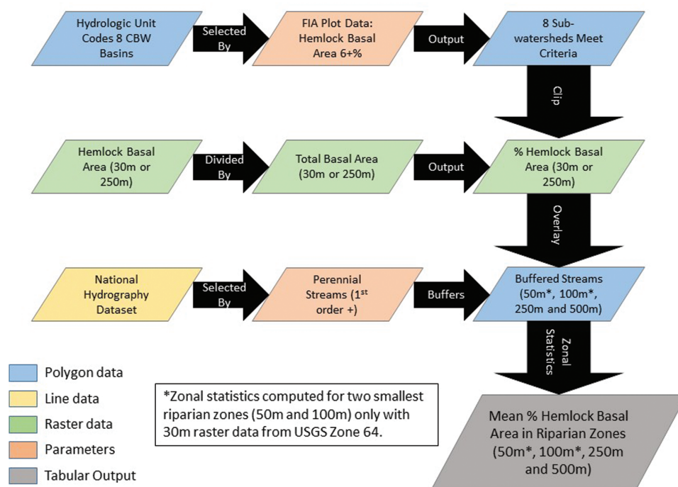
Figure 2. GIS procedure for estimating percent hemlock basal area per acre in riparian zones (50 m, 100 m, 250 m, 500 m) of Chesapeake Bay subwatersheds with at least 6% hemlock basal area. Raster layers of 250 m and 30 m were used to model basal area at two spatial scales.
