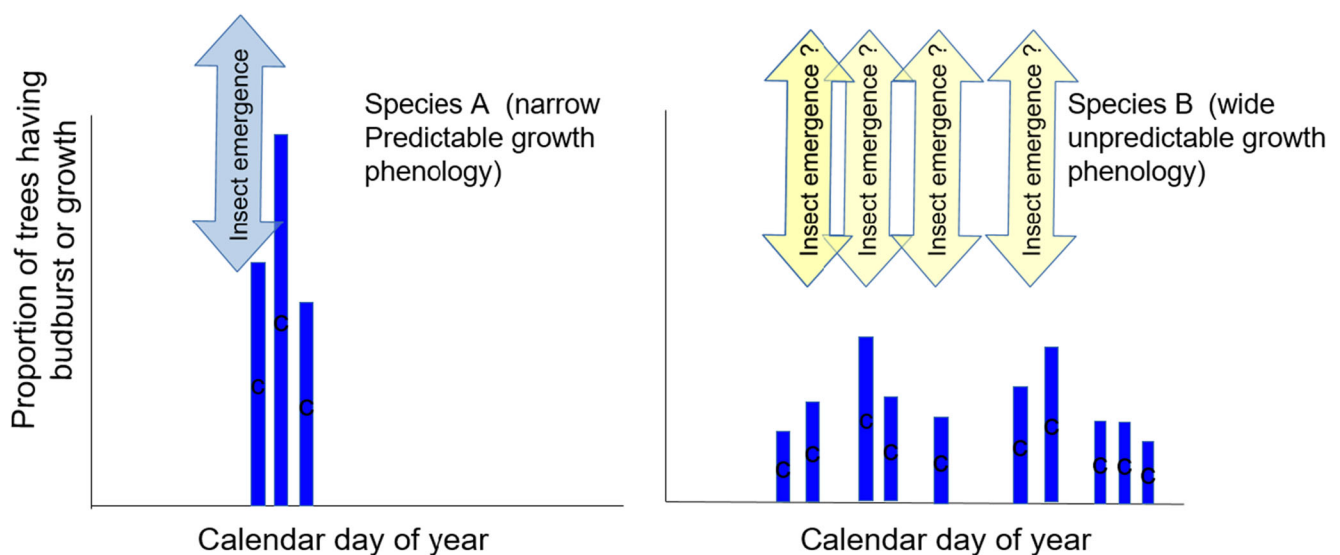
Fig. 2 Synchronism of insect emergence facilitated when tree phenology occurs predictably over a short time window in panel 1 rather than for a tree species with a less predictable or more variable growth phenology (panel 2)
