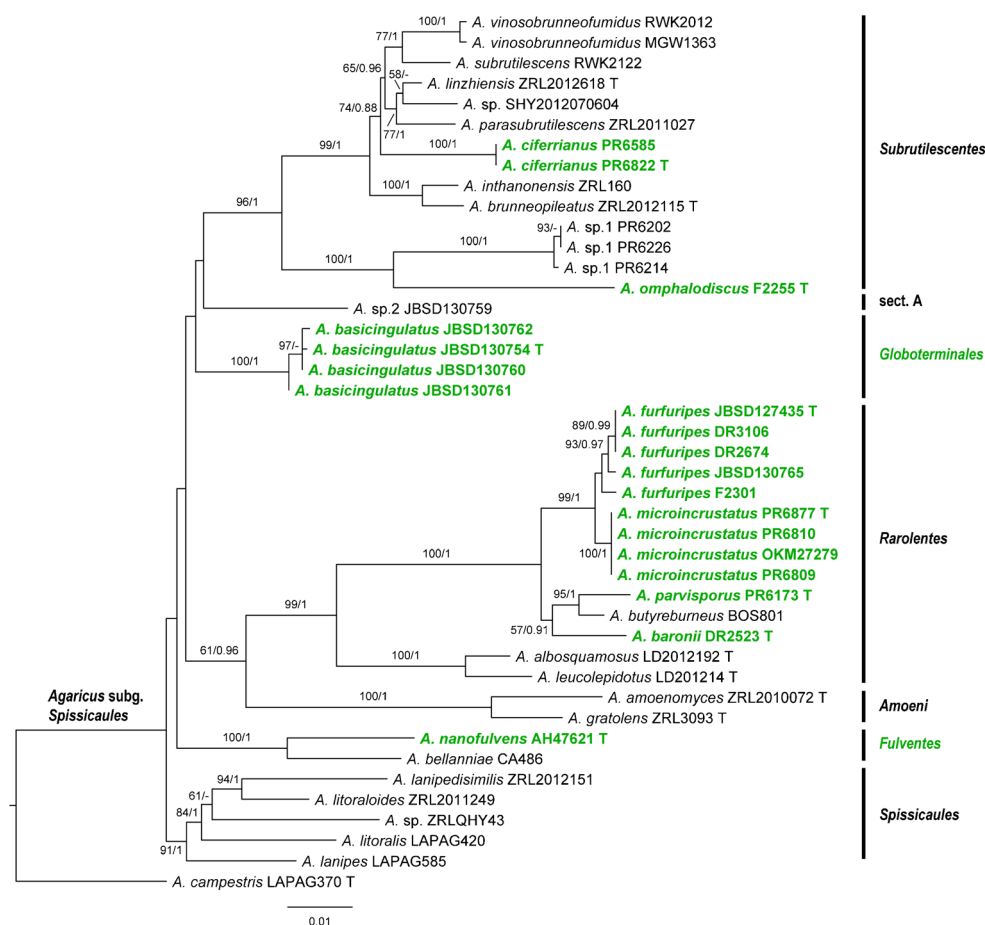
Fig. 2 Phylogeny of Agaricus subg. Spissicaules generated from analyses of ITS, LSU, and TEF1 sequences, rooted with A. campestris . Support values along branches are from ML Bootstrap ( \geq 50\% ), and Bayesian posterior probabilities (PP \geq 0.80 ), respectively. New taxa are highlighted in green
