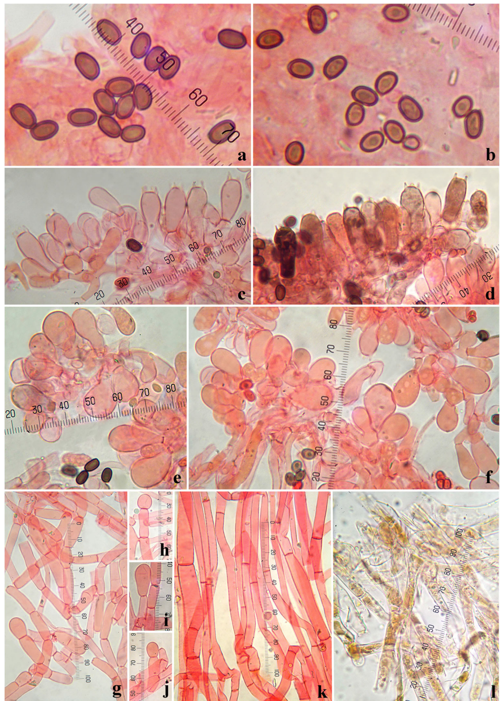
Fig. 6 Microscopic characters of Agaricus basisingulatus . a–k in ammoniacal Congo red; l in water. a, c–e, h, k–l JBSD130754, Holotype. b, f JBSD130767. g, i, j JBSD13076. a–b Spores. c–d Basidia. e–f Cheilocystidia. g–j Hyphae of the lower surface of the annulus ( h–j globose terminal elements). k–l Pileipellis hyphae. Photos by L.A. Parra
