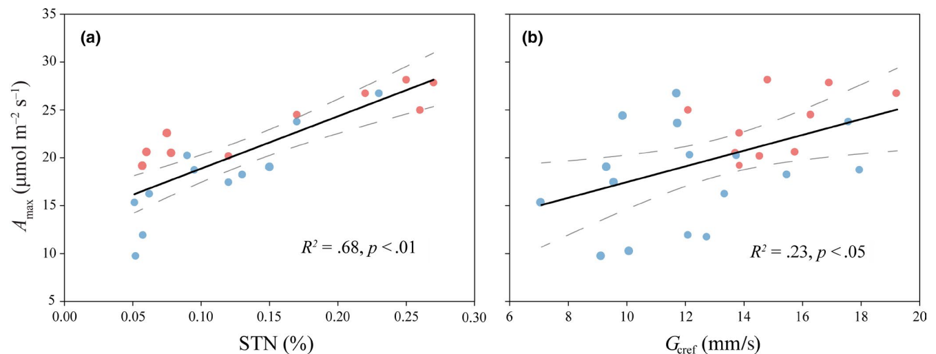
FIGURE 4 Relationship between canopy photosynthetic capacity ( A_{\max} ) and soil total nitrogen (STN) at 0–20 cm (a) and reference canopy conductance ( G_{\text{cref}} ; b) for the mature evergreen forests (blue) and deciduous forests (red) in temperate zones. The black lines are fitted regression lines across two forest types, and the grey dashed lines indicate the 95% confidence intervals. Only the forest sites with STN data available were plotted in panel (a) [Colour figure can be viewed at wileyonlinelibrary.com ]
