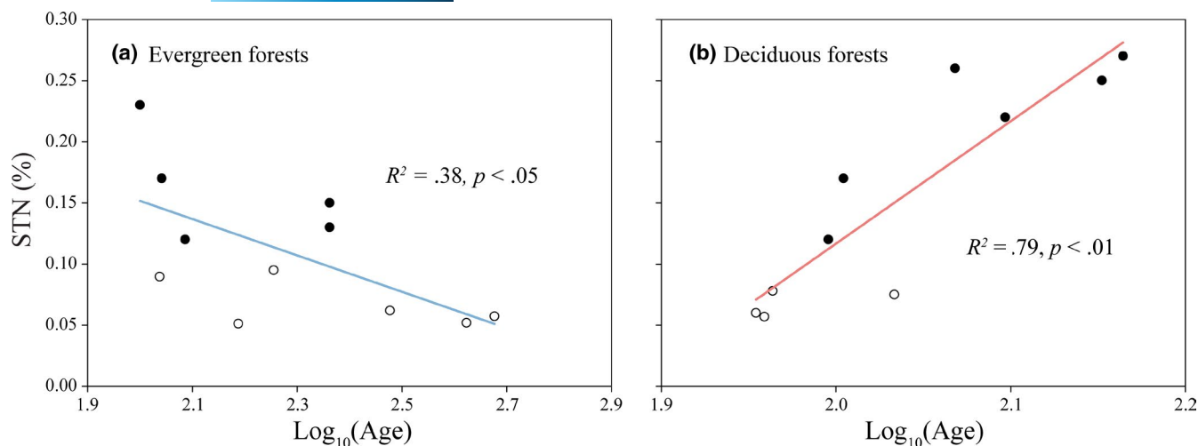
FIGURE 5 Relationship between soil total nitrogen (STN) at 0–20 cm and the logarithm of stand age (Age) for mature evergreen forests (a) and mature deciduous forests (b), respectively. The filled and hollow circles indicate high- and low soil nutrient conditions (SNCs), respectively. The blue and red lines stand for the fitted regressions across SNCs for mature evergreen and deciduous forests, respectively [Colour figure can be viewed at wileyonlinelibrary.com ]
