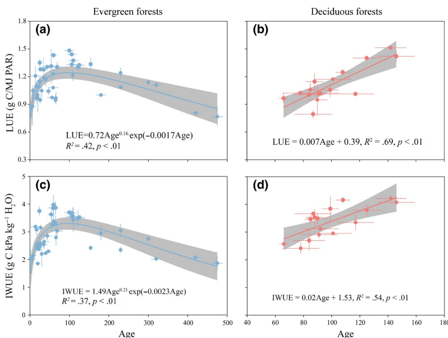
FIGURE 2 Ecosystem-level mean light use efficiency (LUE; a and b) and inherent water use efficiency (IWUE; c and d) over the growing seasons versus stand age (Age) for evergreen forests (blue circles) and deciduous forests (red circles) in temperate regions. The vertical bars indicate the standard errors of multi-year mean resource use efficiencies (RUEs) during the growing season. The horizontal bars represent the study years at each flux site. The blue and red solid lines indicate the fitted equations for evergreen forests and deciduous forests, respectively, and the gray shades are the 95% confidence intervals [Colour figure can be viewed at wileyonlinelibrary.com ]
