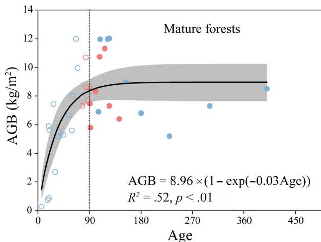
FIGURE 1 Dynamics of aboveground biomass (AGB) with stand age (Age) for the temperate forests. The blue circles and red circles represent evergreen forests and deciduous forests, respectively. Filled circles indicate the mature forests. The gray area around the regression line stands for the 95% confidence interval. Biomass data were not available for all flux sites, and only the sites with AGB data were plotted [Colour figure can be viewed at wileyonlinelibrary.com ]
