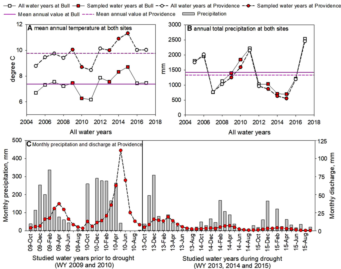
Figure 2. Climatic and stream flow temporal variation within the Kings River Experimental Watersheds in the southern Sierra Nevada, California. Mean annual air temperature ( A ) and total precipitation ( B ) at the Providence and Bull sites for Water Years 2005–2017. Monthly precipitation and stream discharge ( C ) at the Providence site during studied Water Years (data from the Bull site are not shown but followed a similar pattern; Hunsaker and Safeeq 2017, 2018).
