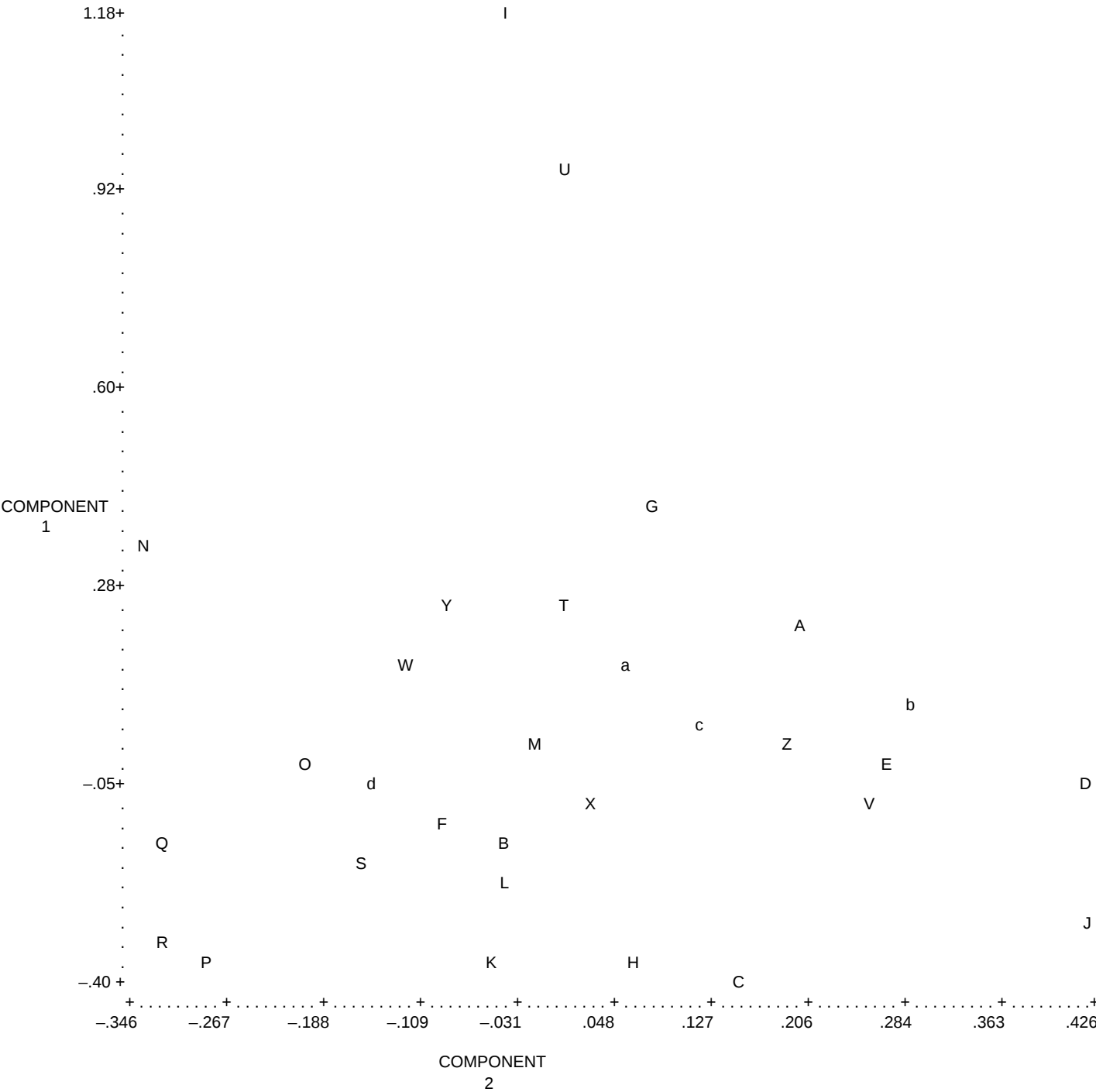
DISPLAY 17. PRINCIPAL COMPONENT ANALYSIS: SCATTERGRAM (LEGEND ON PREVIOUS PAGE) OF COMPONENT SCORES
