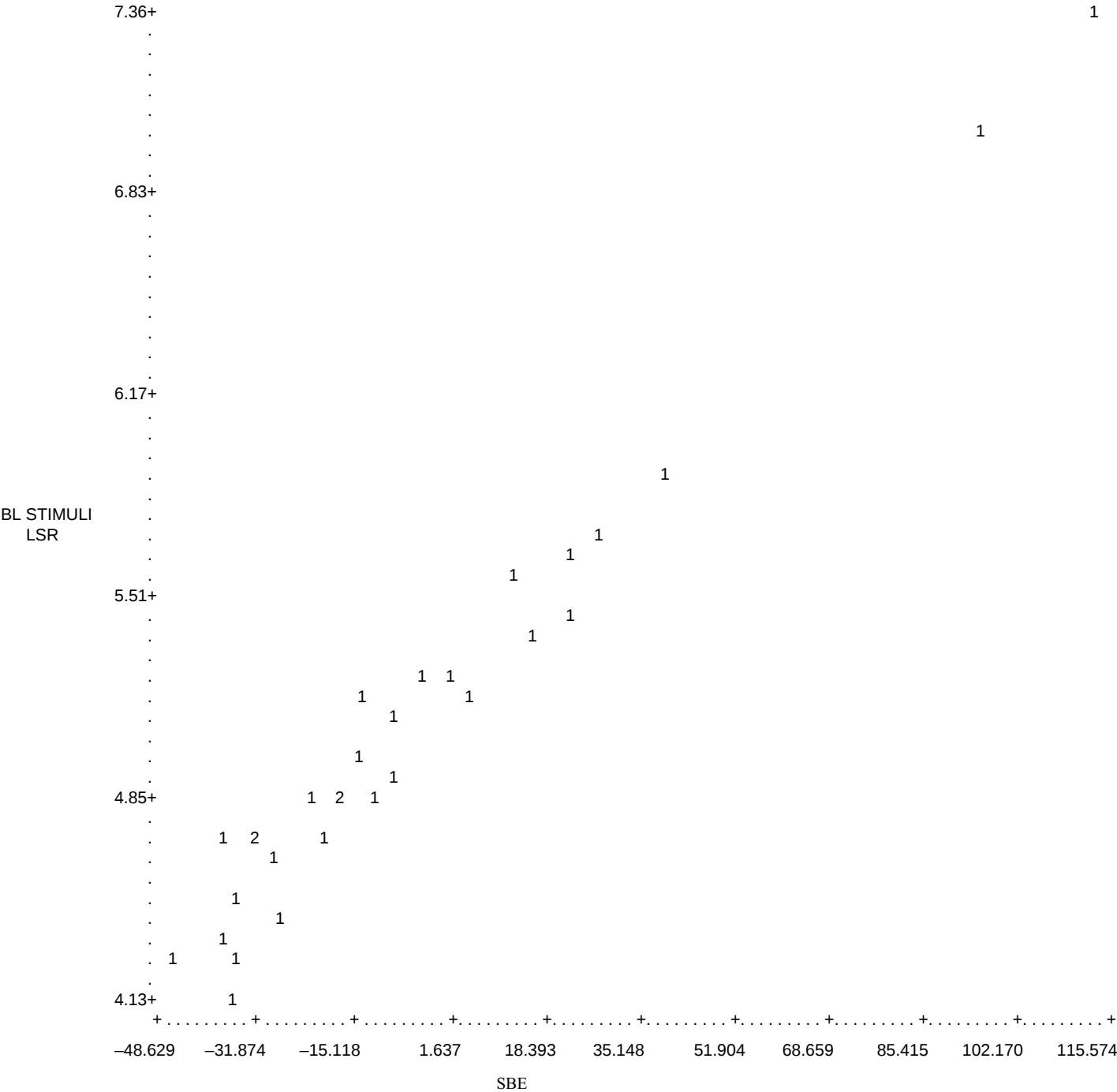
DISPLAY 8. SCATTERGRAM OF TWO OUTPUT MEASURES (CORRELATION LESS THAN .986)
