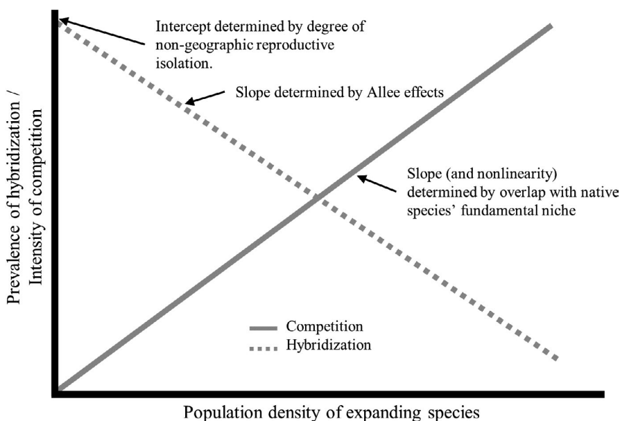
FIGURE 1 The intensity of interspecific competition and prevalence of hybridization between related species in secondary contact may be density-dependent. If so, different niche overlap, a proxy for competition, and hybridization rates should differ between the leading edge of a range expansion and areas where the expanding species has reached high densities in novel sympatry with its congener
