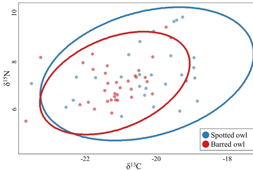
FIGURE 4 Stable isotope signatures of spotted owls and barred owls and the 95% prediction interval of the maximum likelihood estimated ellipse area (Jackson et al., 2012) of their isotopic niches
