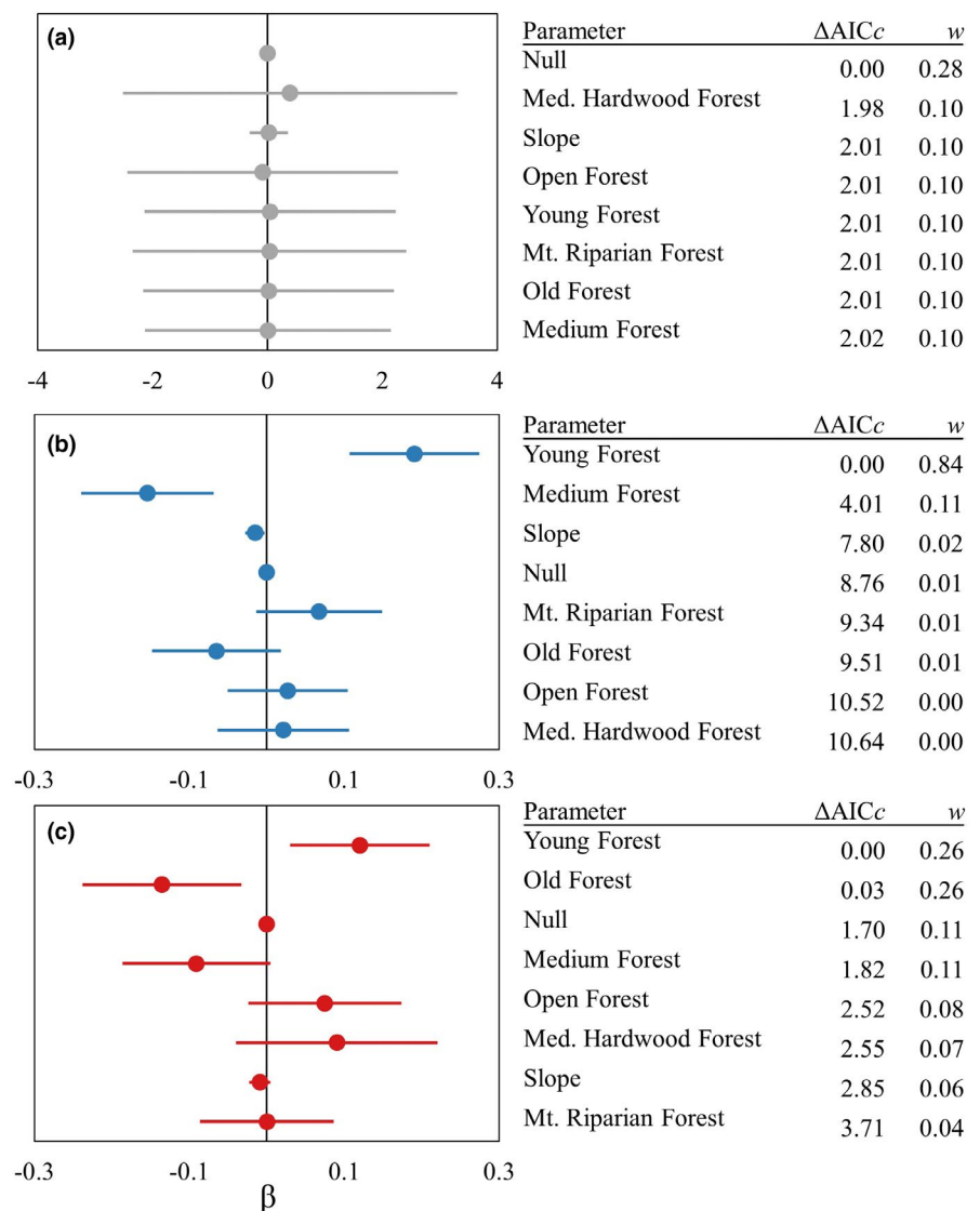
FIGURE 3 Parameter estimates ( \beta ) and model selection tables for logistic regression differentiating spotted and barred owl foraging locations (a) and resource selection functions for spotted owls (b) and barred owls (c). All covariates were standardized. All models included a distance to territory centre term and treated individual owls as random intercepts
