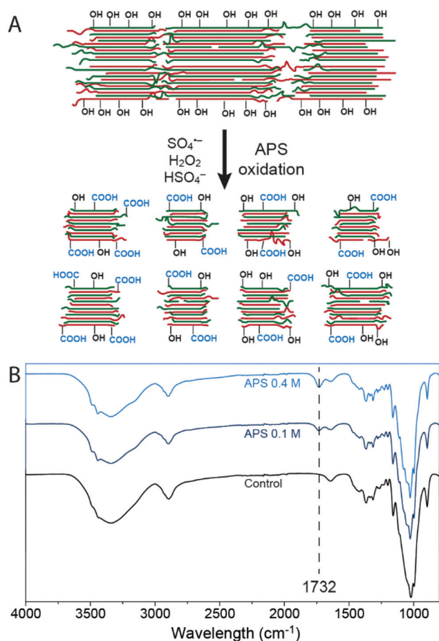
Fig. 6 Schematic illustration of the APS oxidation process introducing surface carboxyl on ox-CNC II (A) and the experimental verification by FTIR (B). Note: Control denotes the CHR after 30 min MLABTH treatment; APS oxidation conditions: temperature 60 °C, time 12 h.
