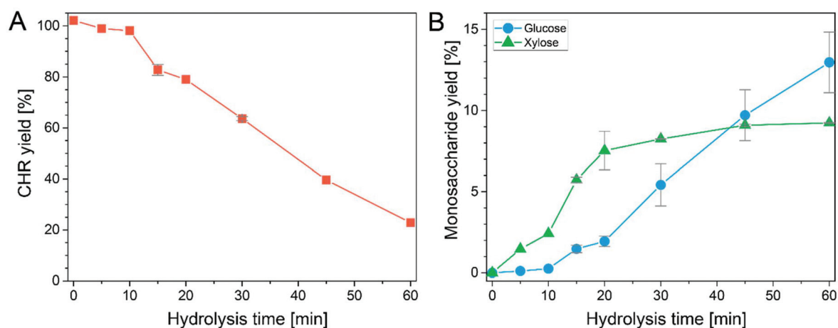
Fig. 2 Yields of CHR (A), glucose, and xylose (B) from BKP as a function of treatment time in the MALBTH.
