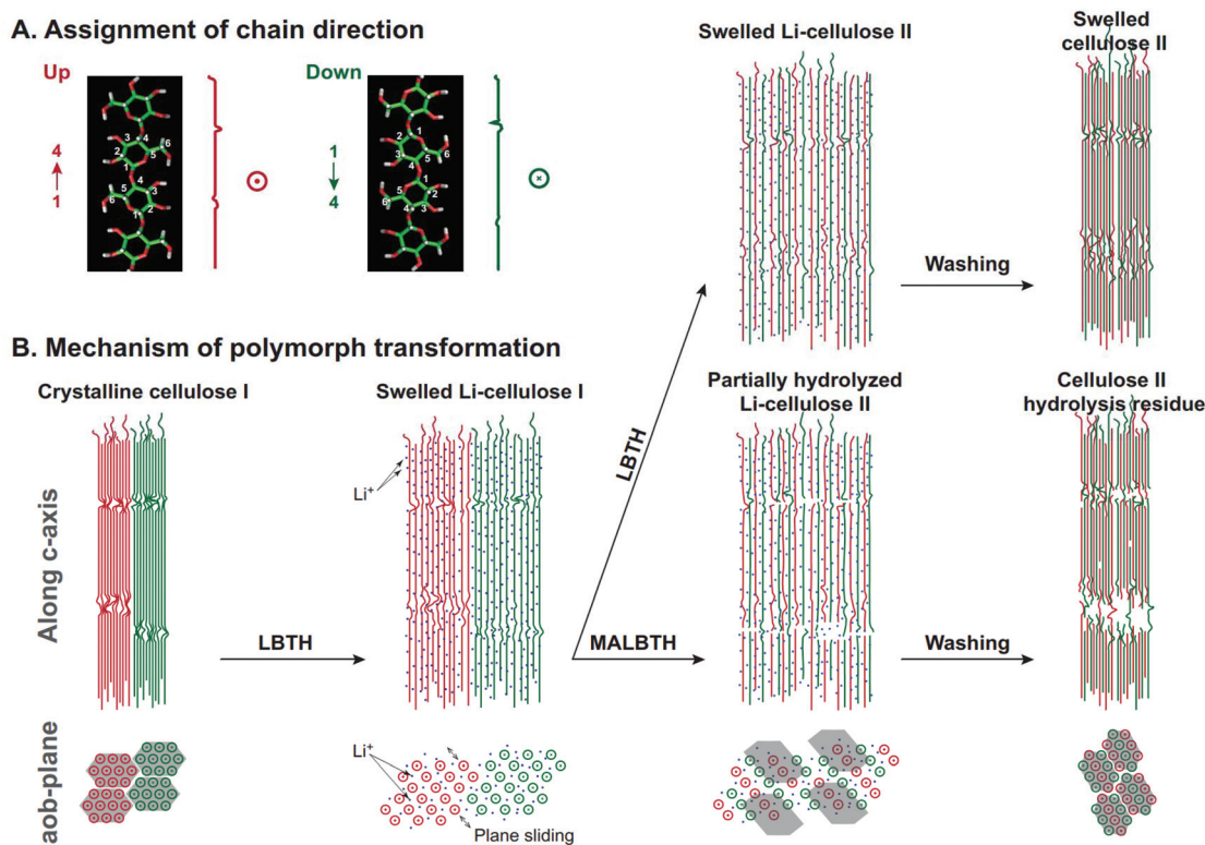
Fig. 5 Schematic illustration of the polymorph transformation from cellulose I to cellulose II under swelling conditions in the MALBTH. (A) Assignment of cellulose chain orientation; (B) Proposed mechanism of polymorph transformation.
