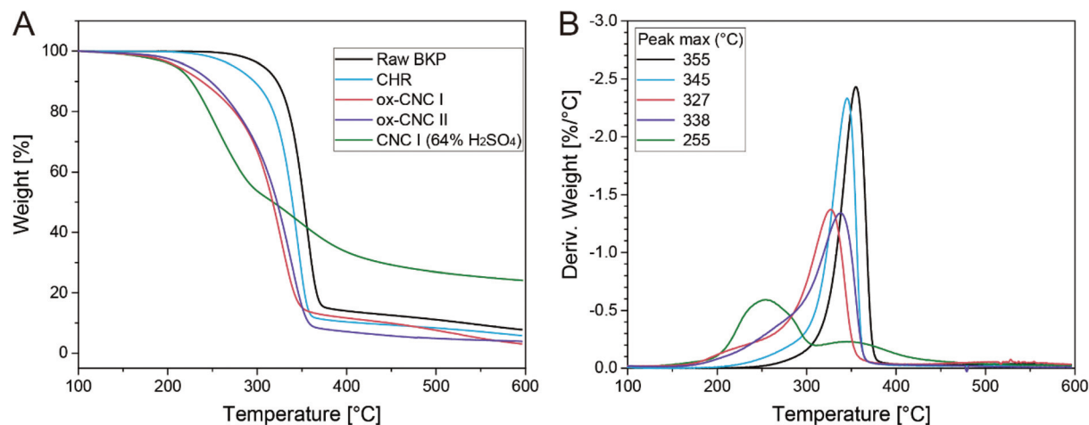
Fig. 8 TGA (A) and the first derivative curves (B) of various cellulose samples.
