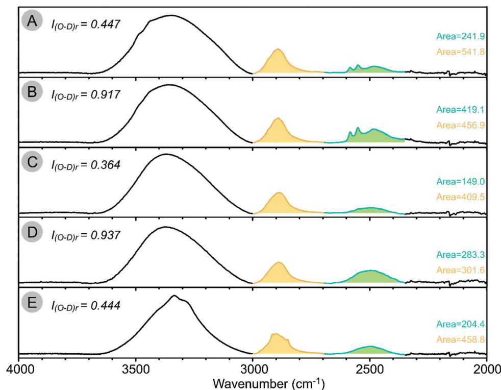
Fig. 3 FTIR spectra of cellulose samples from the hydrogen–deuterium exchange experiment. ((A) Partially hydrolyzed in LiBr-3D 2 O for 30 min and washed with H 2 O; (B) partially hydrolyzed in LiBr-3D 2 O for 30 min and washed with D 2 O; (C) swelled in LiBr-3D 2 O for 45 min and washed with H 2 O; (D) swelled in LiBr-3D 2 O for 45 min and washed with D 2 O; (E) Swelled in D 2 O for 45 min and washed with D 2 O.) Note: All the treatments were at 100 °C. A and B were subjected to a swelling process in LiBr-3H 2 O and LiBr-3D 2 O, respectively before the acid (2.5 mM H 2 SO 4 ) was added. The FTIR spectra were baseline-corrected, normalized and integrated from 3000–2700 cm −1 for the C–H vibrational signal and from 2700–2350 cm −1 for the O–D vibrational signal. The Y-axis denotes absorbance.
