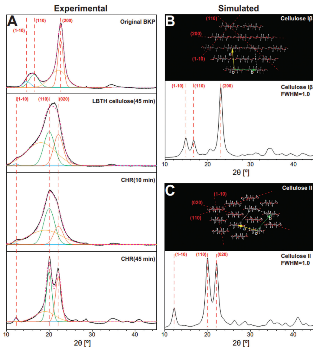
Fig. 4 The experimental XRD patterns of BKP and the CHR prepared in the MALBTH (A), the simulated XRD patterns of cellulose I \beta (B), and cellulose II (C).
