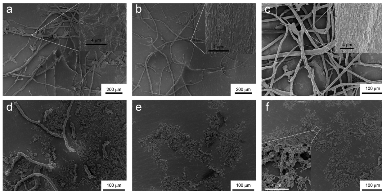
Fig. 1 SEM images of the original BKP (a), swelled BKP in LBTH (b), CHR after the MALBTH treatment (c, 10 min; d, 20 min; e, 30 min; f, 60 min).
