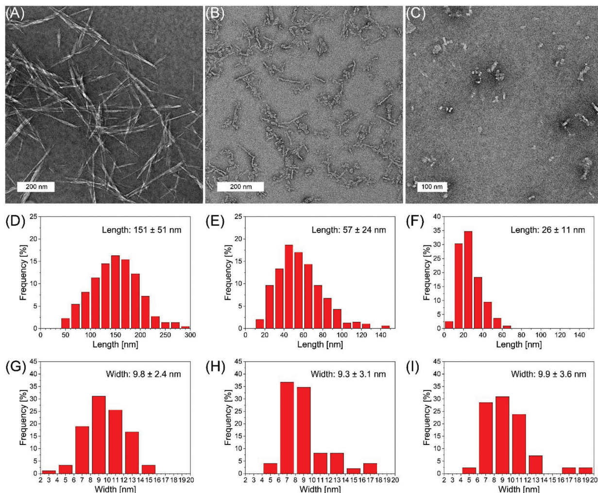
Fig. 7 TEM images and dimensional distributions of ox-CNC I from BKP treated with 0.8 M APS (A, D, and G); ox-CNC II from CHR (15 min MALBTH treatment) treated with 0.2 M APS (B, E, and H); ox-CNC II from CHR (15 min MALBTH treatment) treated with 0.6 M APS (C, F, and I). APS oxidation conditions: temperature 60 °C, oxidation time 12 h.
