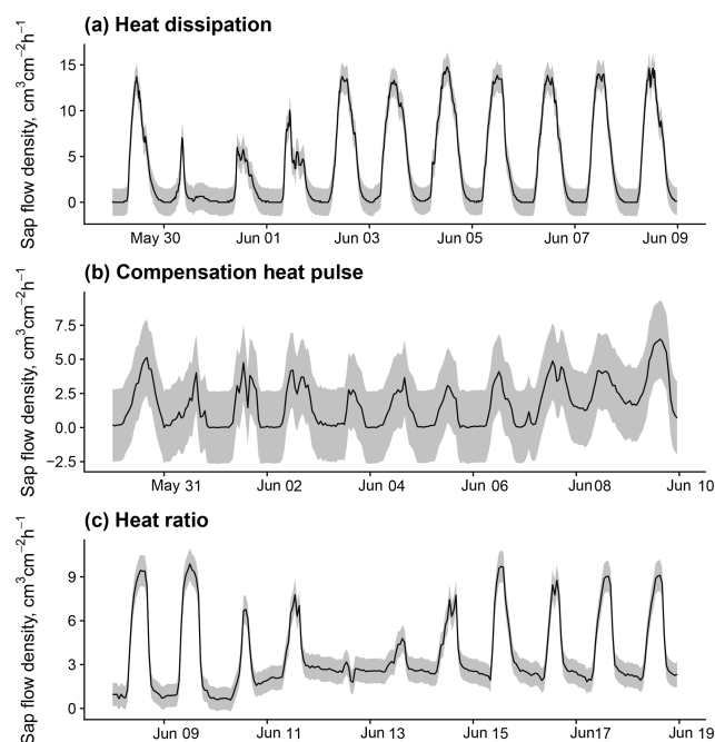
Figure B2. Sub-daily time series of sap flow and methodological uncertainty estimations (1 standard error) according to the model in Fig. B1 for 10 d periods in trees measured with (a) heat dissipation, (b) compensation heat pulse, and (c) heat ratio sensors. Data for panel (a) from a Pinus sylvestris tree in dataset ESP_VAL_SOR; data for panel (b) from a Pinus sylvestris tree in GBR_DEV_CON; and data for panel (c) from a Eucalyptus victrix tree in AUS_KAR.
