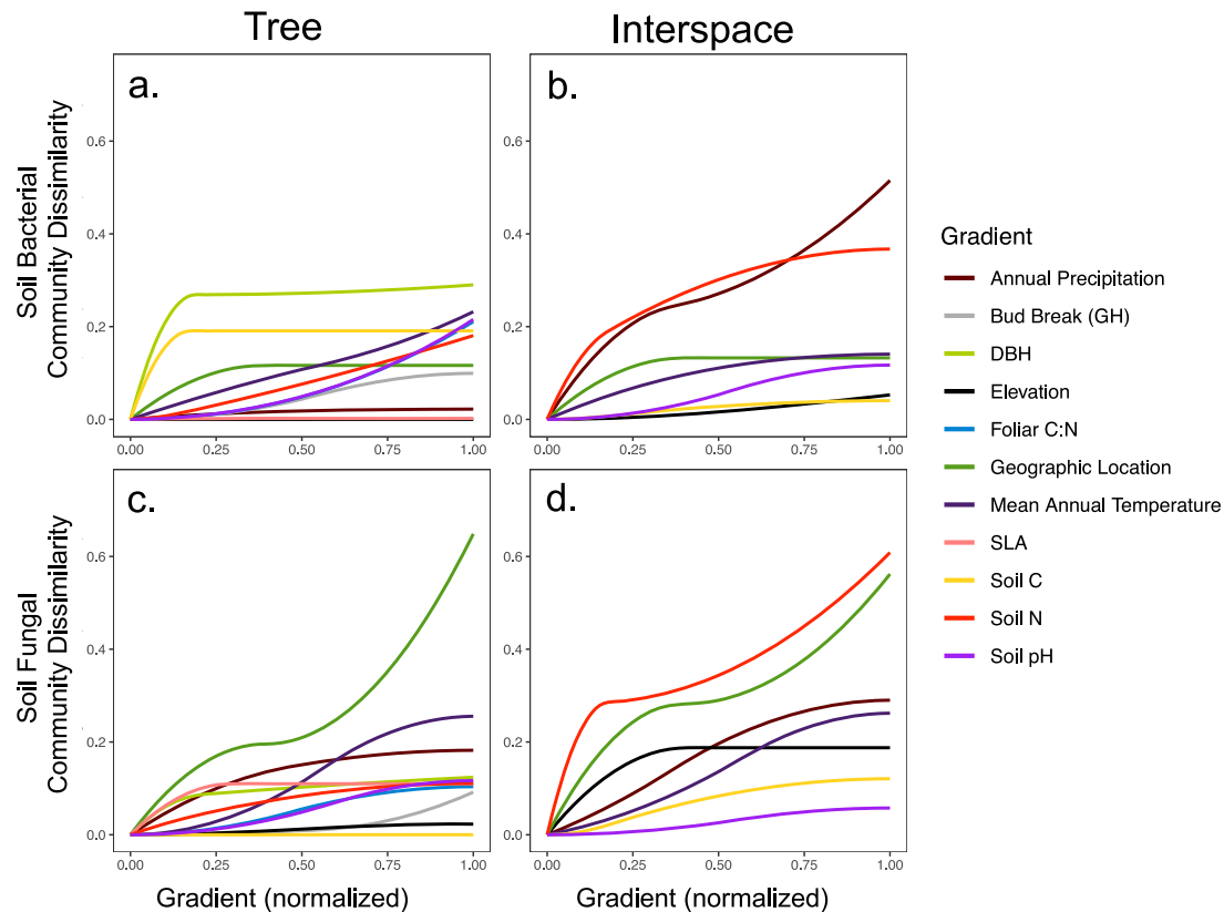
Fig. 3 Landscape-level variation in climate, edaphic characteristics, and plant phenotypes drive turnover in soil bacterial and fungal communities.
