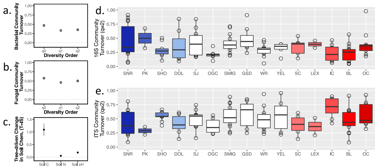
Fig. 2 Tree-driven differences in soil microbial communities and soil chemistry. a Mean bacterial community turnover for diversity orders q = 0-2 (when turnover/ \beta -diversity = 0 tree and interspace communities are identical; when turnover/ \beta -diversity = 1 tree and interspace communities did not share any members). b Mean fungal community turnover for diversity orders q = 0-2 . c Mean differences in soil carbon (C), soil nitrogen (N), and soil pH between each tree-interspace pair. Error bars in each panel represent 95% confidence interval of the mean. d Population-level differences in bacterial community turnover ( q = 2 ; 1/\gamma (reciprocal of Simpson's \gamma )) between tree-interspace pairs. e Population-level differences in fungal community turnover ( q = 2 ) between tree-interspace pairs. P. angustifolia populations across the 15 watersheds are arranged from coolest to warmest. Center line in each boxplot represents the median turnover for each tree population, end lines represent lower and upper quartiles, and whiskers represent the minimum and maximum turnover estimates within each tree population. Blue and red boxplots match Fig. 1 and represent populations re-sampled in 2015 for soil inoculation experiment. *The soil microbiome was not sequenced for the Gros Ventre River population but was included in the inoculation experiment.
