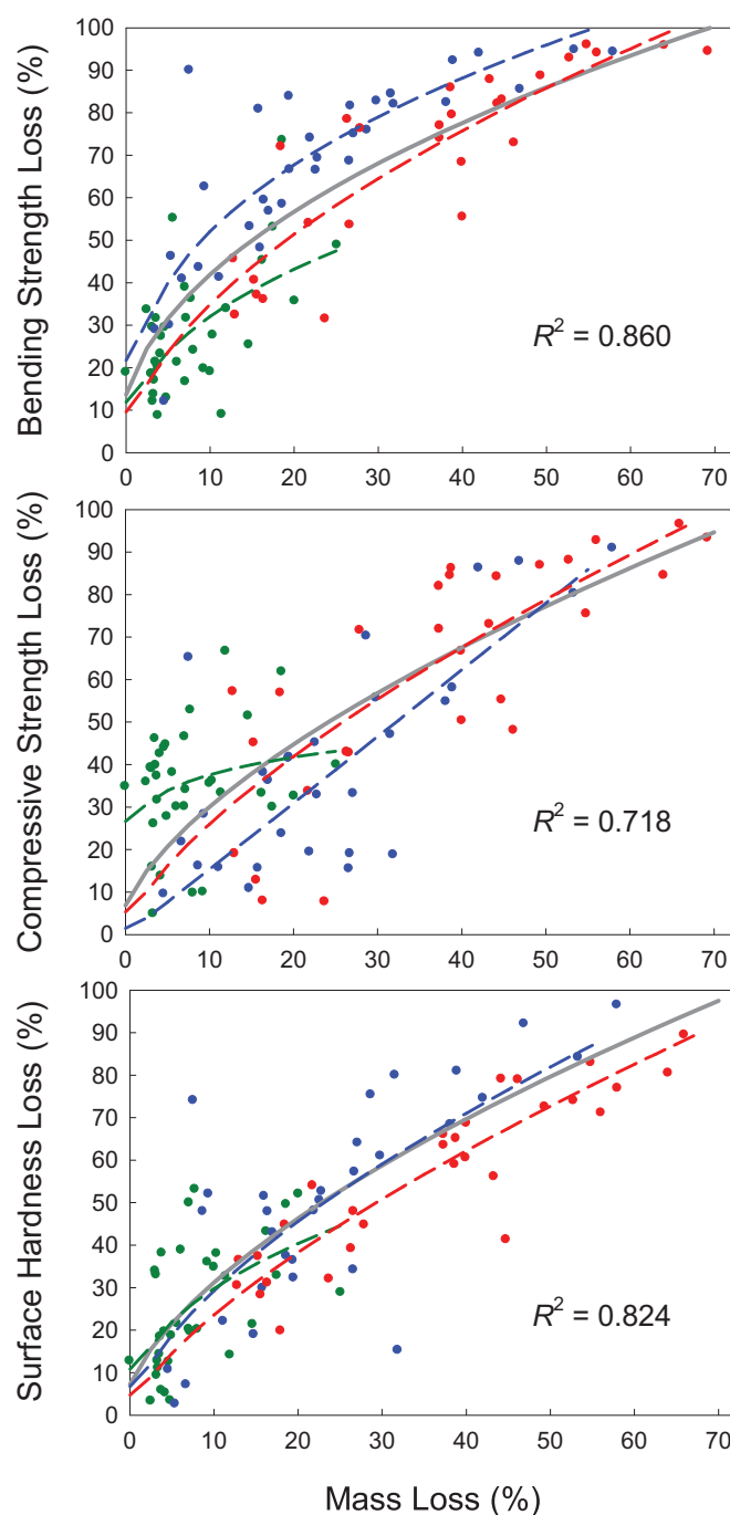
Fig. 1. Relationship between three strength-loss metrics (bending strength, compressive strength, and surface hardness) and mass loss of decaying wood. Colored dots and lines represent the three species tested ( Abies balsamea = green, Acer saccharum = blue, Populus tremuloides = red); the grey line represents pooled species data. R^2 values refer to pooled data. Model parameters for individual species are shown in Table 1. Intercepts of the fitted curves are positive for all three metrics, meaning that strength is reduced before any mass loss has occurred.
