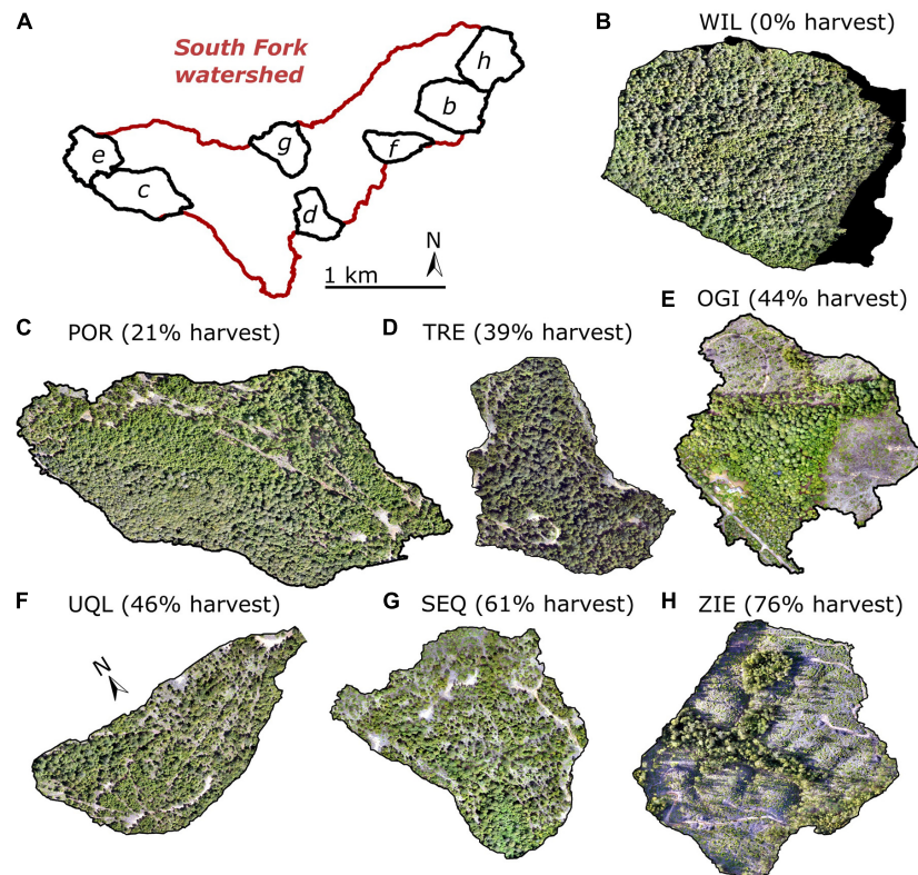
FIGURE 6 | Orthomosaics showing harvested sub-watersheds and a control sub-watershed (WIL). Panels (B–H) are marked on the map in panel (A). The images for the orthomosaics were collected with an unmanned aerial system (UAS) in spring 2020 after the Third Experiment harvesting was completed.
