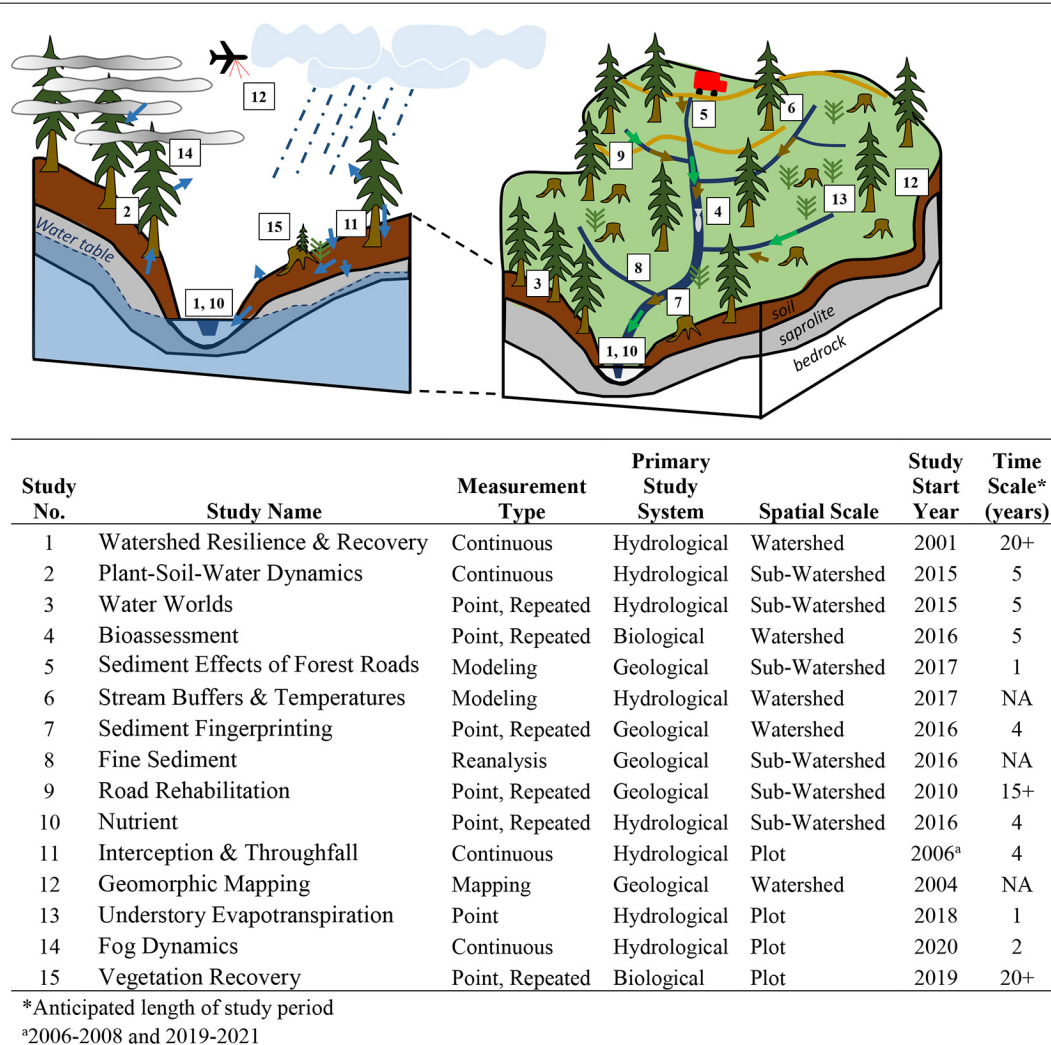
FIGURE 2 | Conceptual study diagram depicting approximate spatial representation of 15 studies associated with the Third Experiment. Study numbers and descriptions are located in the table. Arrows represent the following (not to scale): blue, hydrologic fluxes; green, nutrient fluxes; brown, sediment fluxes.
