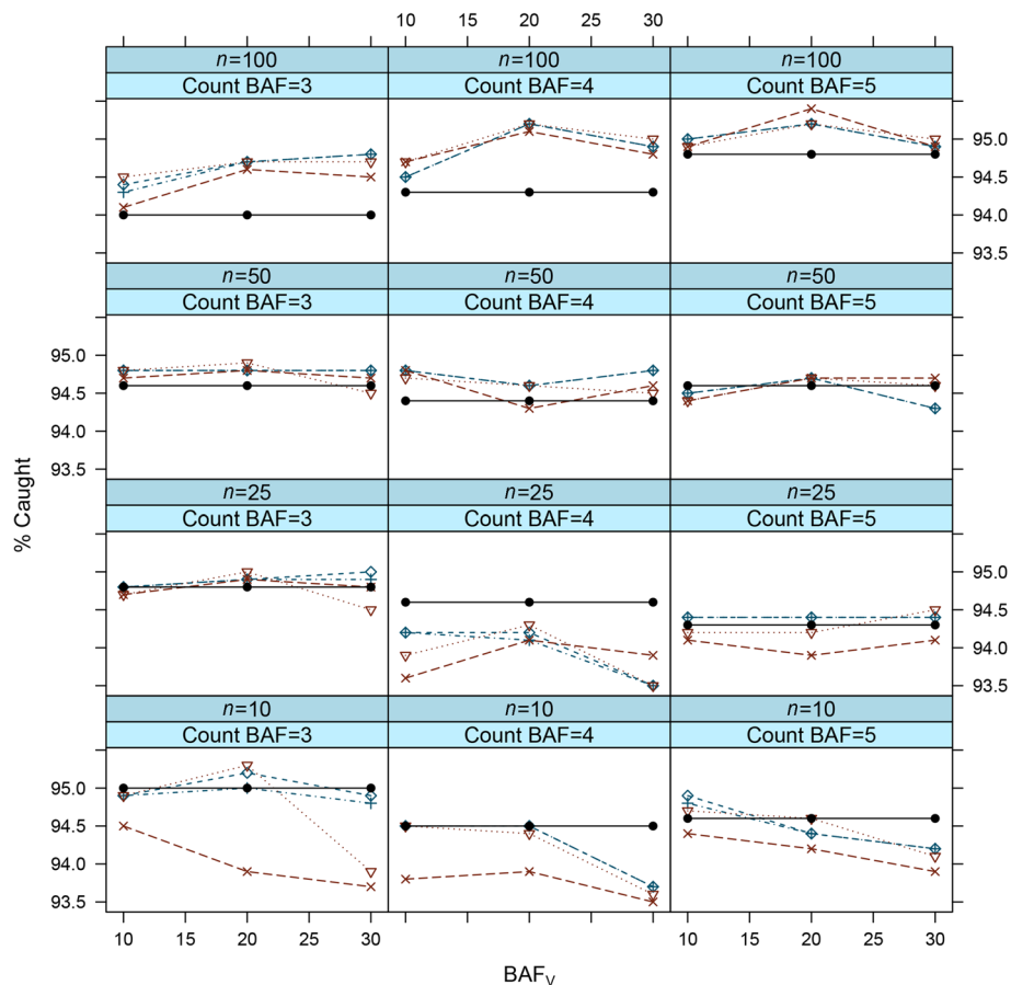
Fig. 4 The northern hardwoods Monte Carlo simulation results for confidence interval capture rates as the average over 1,000 replications for each BAF pair and sample size with the Delta Method (dashed, \diamond ), Goodman's (dot-dashed, + ), the point-based Delta method (dotted, \nabla ) and the simplified point-based Delta method (long-dash, \times ). The reference line (solid, \bullet ) is the average Monte Carlo standard error for the BAF_c HPS results
