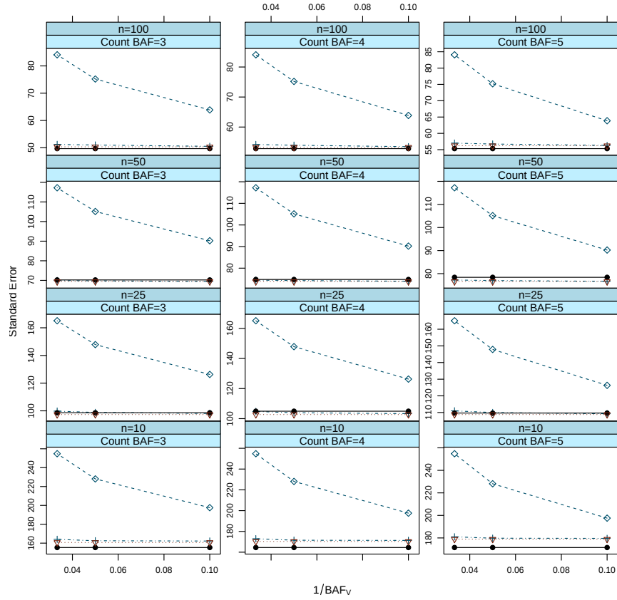
Figure S.9: The white pine Monte Carlo standard error simulation results as the average over 1,000 replications for each BAF pair and sample size with \bar{s}_{\hat{V}_v} = (dashed, \diamond ), \bar{s}_{\hat{V}_B} = (dot-dashed, + ), \bar{s}_{\hat{V}_c} = (dotted, \nabla ), and the “reference” \bar{s}_{\hat{V}_c} = (solid, \bullet ).
