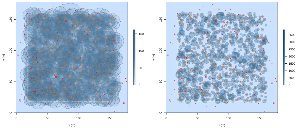
(S.1a) Basal area: \mathcal{F}_c = 3
