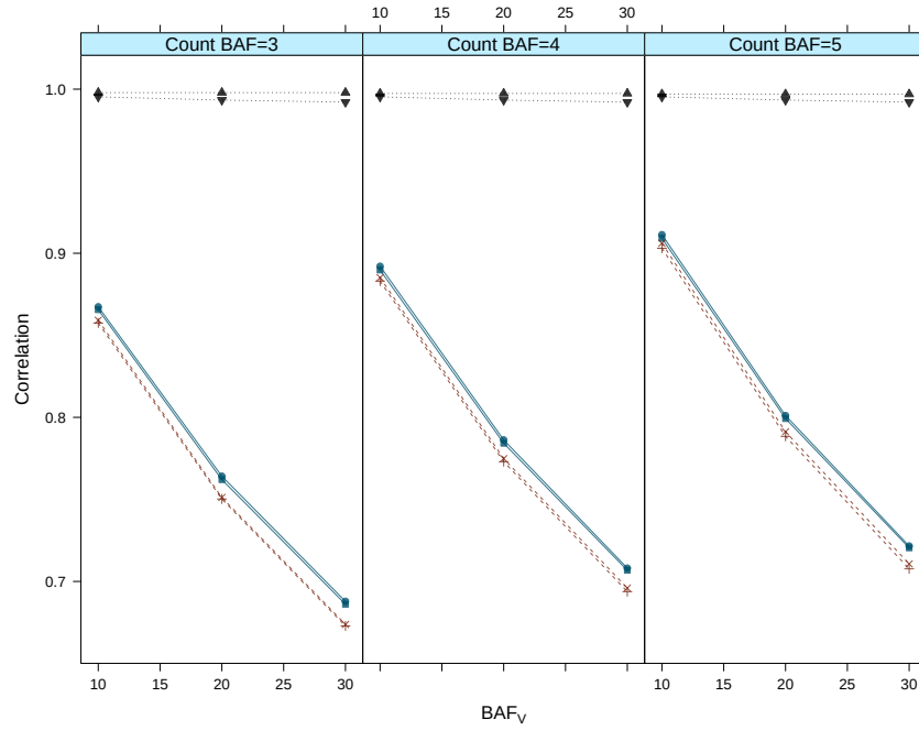
Figure S.5: The white pine ‘population’ correlation results. The point-wise correlations, given are: \rho(B_{cs}, B_{vs}) (solid, \bullet ), \rho(B_{cs}, V_{vs}) (dash, + ), \rho(V_{cs}, B_{cs}) (dotted, \blacktriangle ), \rho(V_{cs}, B_{vs}) (solid, \blacksquare ), \rho(V_{cs}, V_{vs}) (dash, \times ), \rho(V_{vs}, B_{vs}) (dotted, \blacktriangledown ). Here s ranges over all 18,496 sample points (grid cells) in the population.
