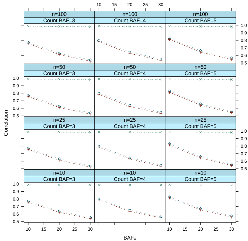
Figure S.8: The northern hardwood Monte Carlo simulation correlation results as the average over 1,000 replications for each BAF pair and sample size. The point-wise correlations, \hat{\rho}(V_{V_s}, B_{V_s}) (dot-dashed, \times ), \hat{\rho}(B_{C_s}, V_{V_s}) (dash, + ) and \hat{\rho}(B_{C_s}, B_{V_s}) (dotted, \diamond ), are presented.
