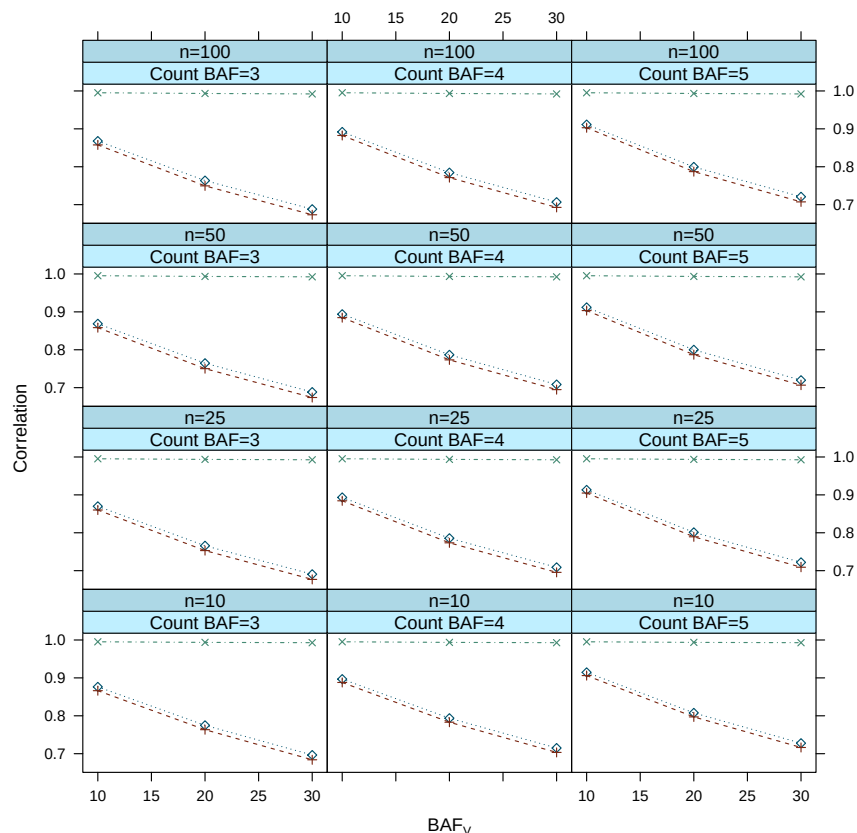
Figure S.10: The white pine Monte Carlo simulation correlation results as the average over 1,000 replications for each BAF pair and sample size. The point-wise correlations, \hat{\rho}(V_{v_s}, B_{v_s}) (dot-dashed, \times ), \hat{\rho}(B_{c_s}, V_{v_s}) (dash, + ) and \hat{\rho}(B_{c_s}, B_{v_s}) (dotted, \diamond ), are presented.
