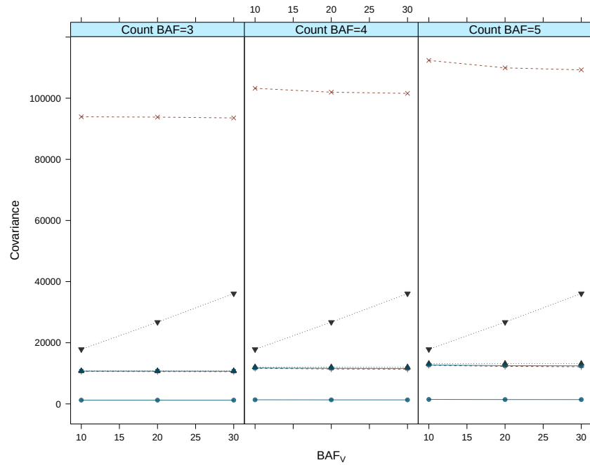
Figure S.3: The northern hardwoods ‘population’ covariance results. The point-wise covariances, given are: \rho(B_{c_s}, B_{v_s}) (solid, \bullet ), \rho(B_{c_s}, V_{v_s}) (dash, + ), \rho(V_{c_s}, B_{c_s}) (dotted, \blacktriangle ), \rho(V_{c_s}, B_{v_s}) (solid, \blacksquare ), \rho(V_{c_s}, V_{v_s}) (dash, \times ), \rho(V_{v_s}, B_{v_s}) (dotted, \blacktriangledown ). Here s ranges over all 31,684 sample points (grid cells) in the population.
