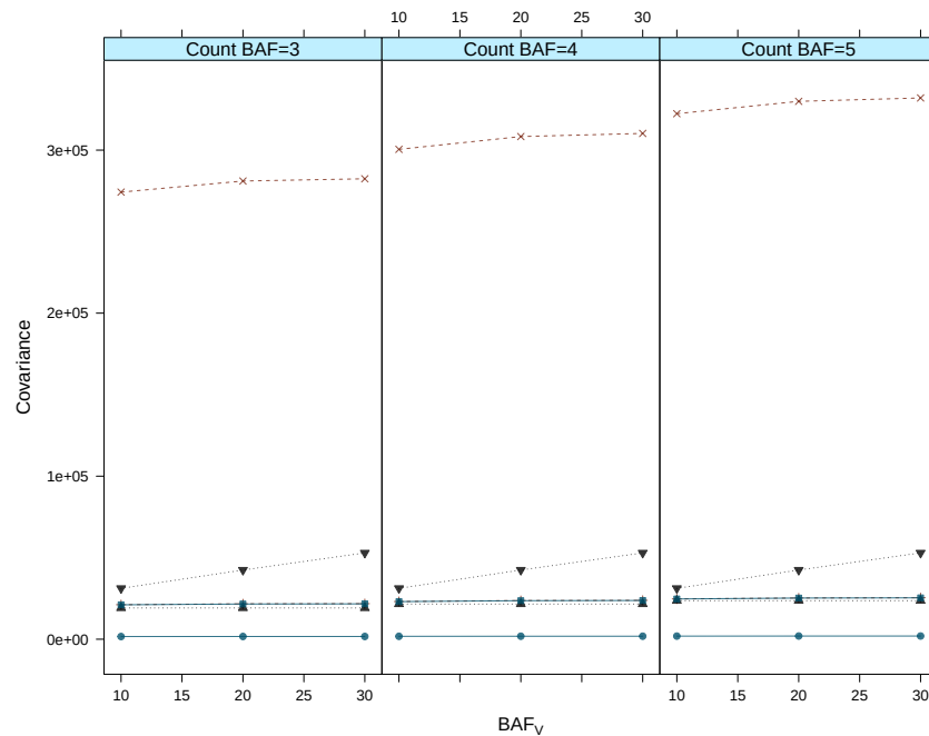
Figure S.6: The white pine ‘population’ covariance results. The point-wise covariances, given are: \rho(B_{c_s}, B_{v_s}) (solid, \bullet ), \rho(B_{c_s}, V_{v_s}) (dash, + ), \rho(V_{c_s}, B_{c_s}) (dotted, \blacktriangle ), \rho(V_{c_s}, B_{v_s}) (solid, \blacksquare ), \rho(V_{c_s}, V_{v_s}) (dash, \times ), \rho(V_{v_s}, B_{v_s}) (dotted, \blacktriangledown ). Here s ranges over all 18,496 sample points (grid cells) in the population.
