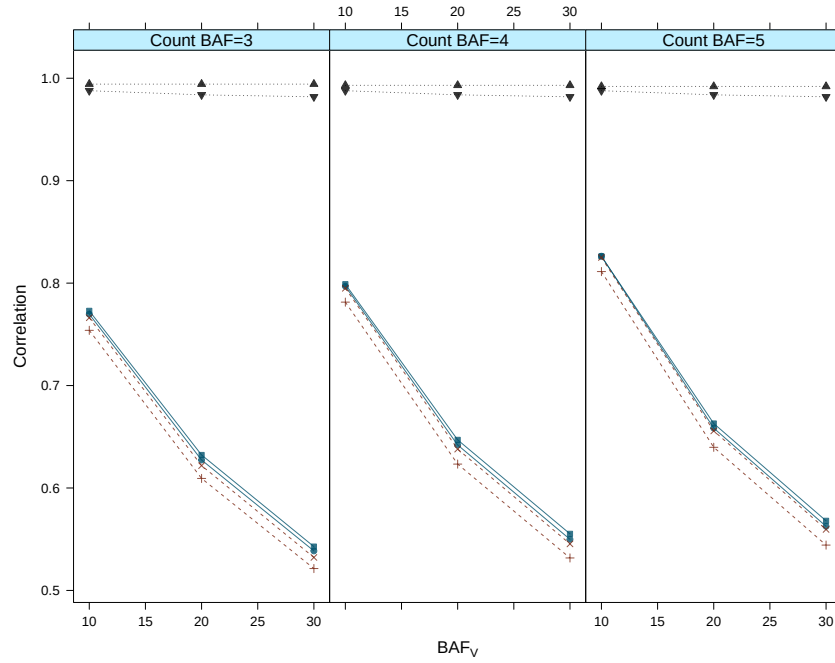
Figure S.2: The northern hardwoods ‘population’ correlation results. The point-wise correlations, given are: \rho(B_{c_s}, B_{v_s}) (solid, \bullet ), \rho(B_{c_s}, V_{v_s}) (dash, + ), \rho(V_{c_s}, B_{c_s}) (dotted, \blacktriangle ), \rho(V_{c_s}, B_{v_s}) (solid, \blacksquare ), \rho(V_{c_s}, V_{v_s}) (dash, \times ), \rho(V_{v_s}, B_{v_s}) (dotted, \blacktriangledown ). Here s ranges over all 31,684 sample points (grid cells) in the population.
