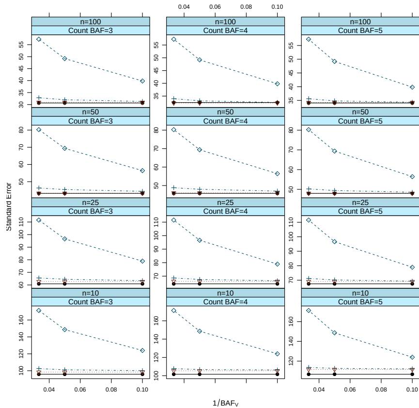
Figure S.7: The northern hardwood Monte Carlo standard error simulation results as the average over 1,000 replications for each BAF pair and sample size with \bar{s}_{\hat{V}_v} = (dashed, \diamond ), \tilde{s}_{\hat{V}_B} = (dot-dashed, + ), \tilde{s}_{\hat{V}_c} = (dotted, \nabla ), and the “reference” \bar{s}_{\hat{V}_c} = (solid, \bullet ).
