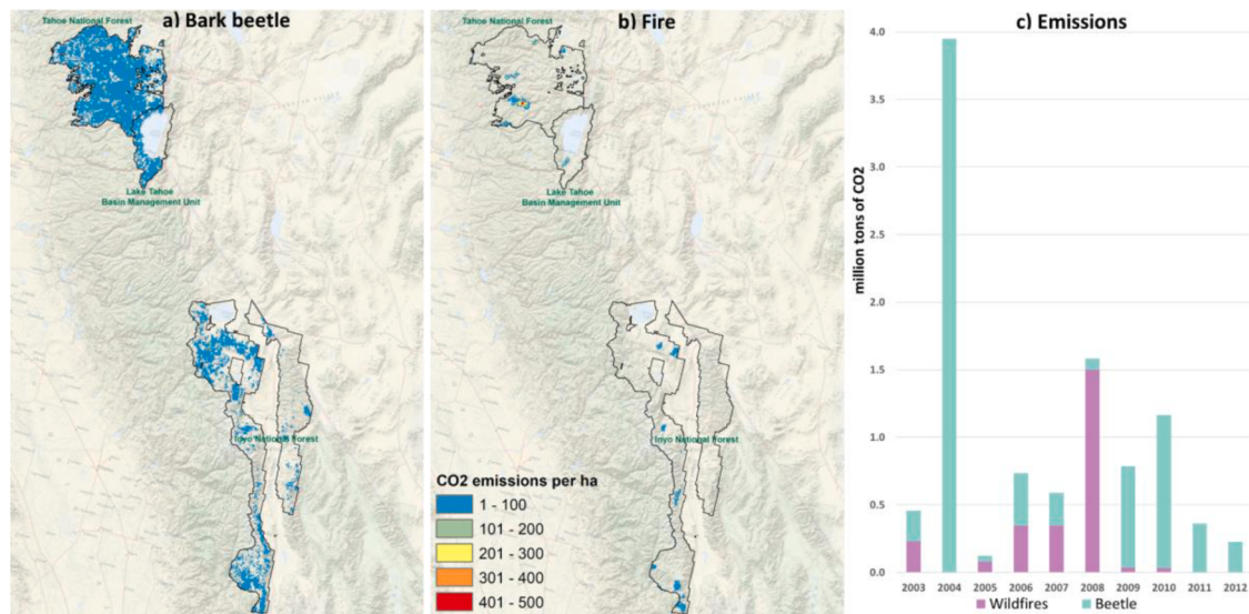
Fig. 4. CO 2 emissions from biomass loss due to bark beetle and wildfires tree mortality (cumulative emissions from 2003 to 2012).
