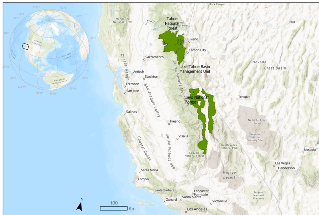
Fig. 1. Study area: Tahoe national forest, lake Tahoe basin management unit, and Inyo national forest.
