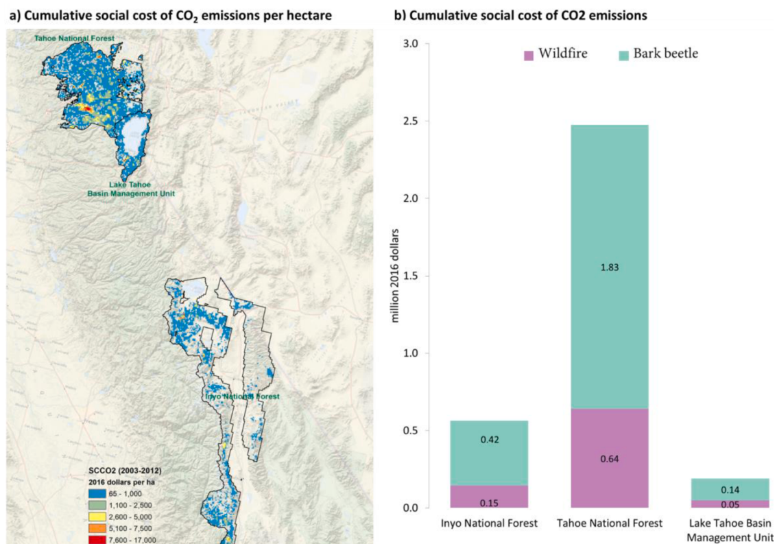
Fig. 5. Cumulative social cost of CO 2 emissions from tree mortality due to bark beetle and wildfire disturbances (2003-2012). Estimates using the global social cost of CO 2 emissions discounted at 3%.
