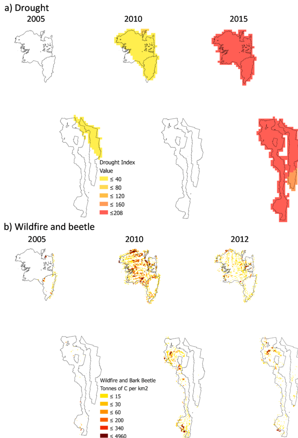
Fig. 2. Spatial distribution and intensity of forest disturbances: Drought, and wildfire and bark beetle tree damage. Note: Wildfire and beetle mortality are only available for the period 2003-2012. The legend in panel b is based on the quantile distribution of the carbon emissions.
