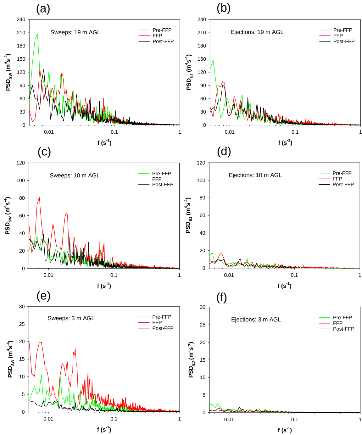
Figure 10. Mean power spectral density (PSD: \text{m}^4 \text{s}^{-4} ) vs. frequency ( f : \text{s}^{-1} ) curves for the negative vertical momentum flux contributors of (a,c,e) sweeps (PSD SW ) and (b,d,f) ejections (PSD EJ ) at the 19-m (top row), 10-m (middle row), and 3-m (bottom row) levels for the pre-FFP, FFP, and post-FFP periods, computed from all five in situ towers.
