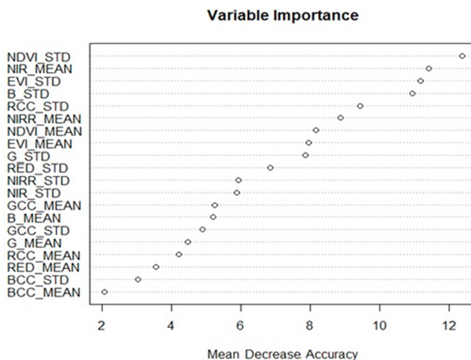
Figure 4. Graph of variable importance produced by the Random Forest model. Vertical axis values are the predictor variables and the horizontal axis shows the decrease in model accuracy if the variable is removed.
