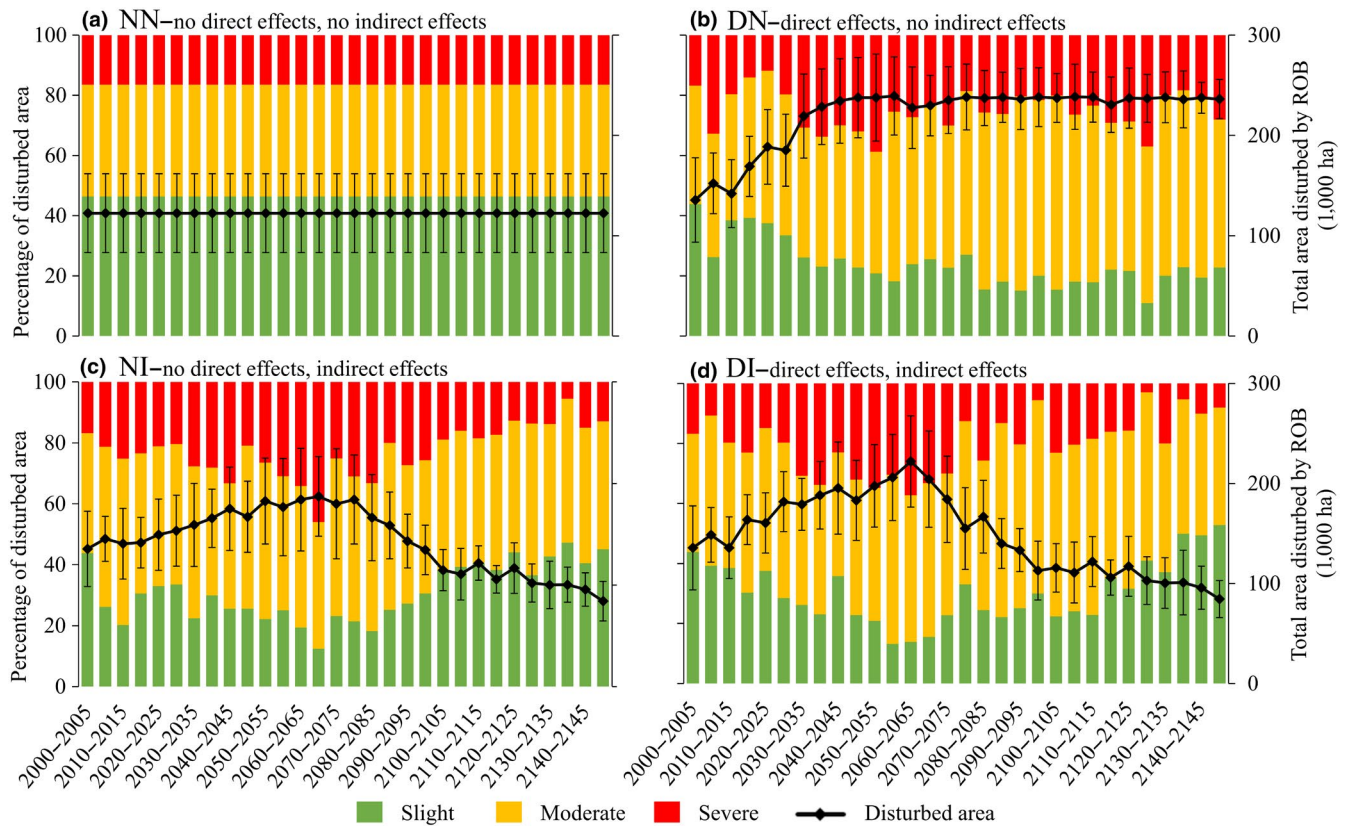
FIGURE 3 Temporal changes in ROB severity distributions within the ROB disturbed area under each simulation scenario. Coloured bars represent the percentage of the disturbed area by three ROB severity classes at each time step (left y-axis), whereas the superimposed line plots represent the trend in the total area disturbed by ROB (right y-axis). Values are averaged across 10 replicates. Error bars represent \pm 1 SD of area disturbed. (a–d) Plots for NN, DN, NI and DI, respectively
