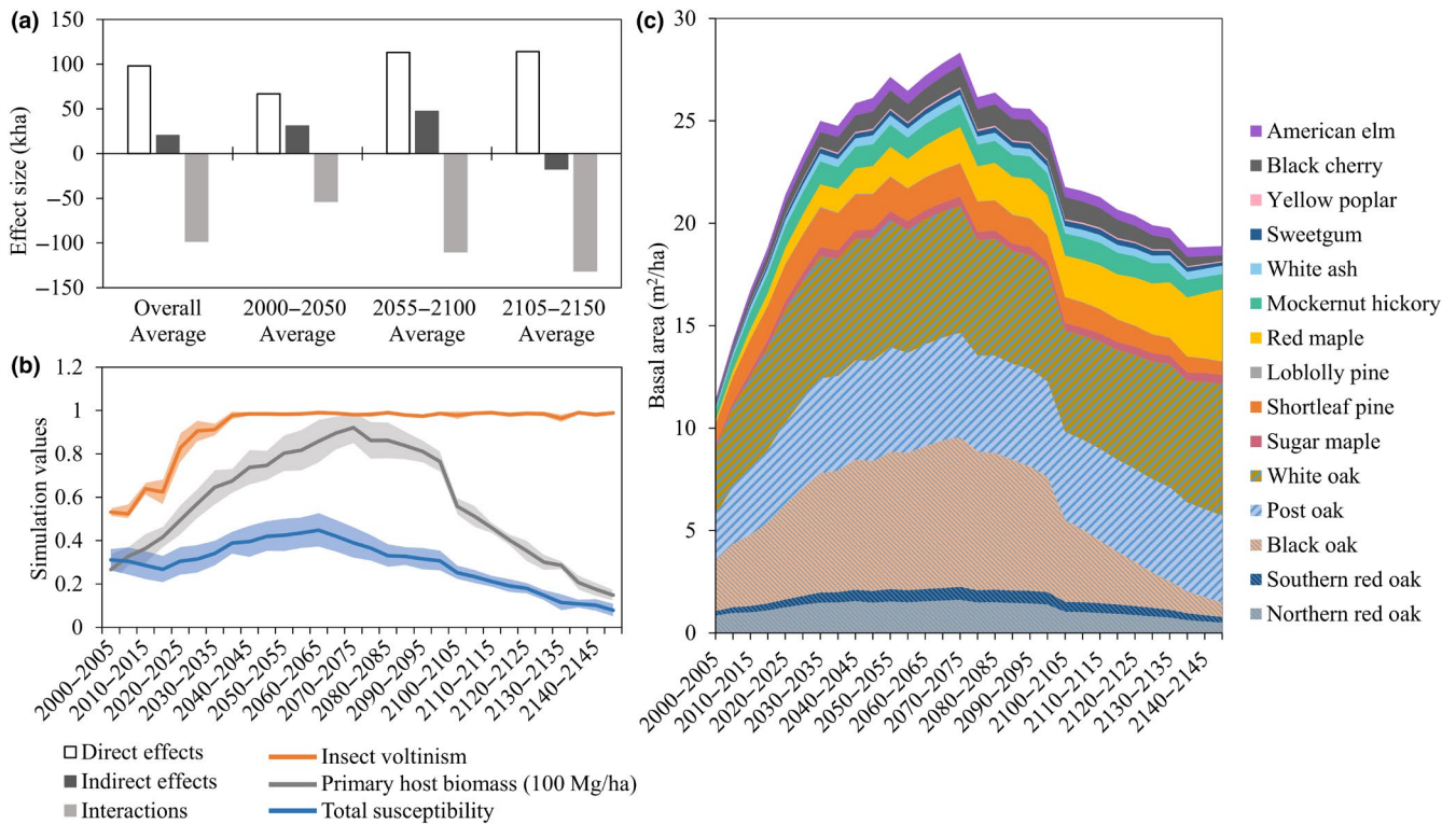
FIGURE 4 (a) The average effect size of direct effects, indirect effects and their interactions under four simulation scenarios. (b) Temporal changes of insect voltinism ( V ), primary host biomass (100 Mg/ha) and total susceptibility ( S ) simulated in LANDIS PRO for the DI scenario. (c) Temporal changes of the species composition in LANDIS PRO for the DI scenario. The backslash and forward slash indicate primary and secondary host tree species, for ROB, respectively. See Table S3 for species' scientific name
