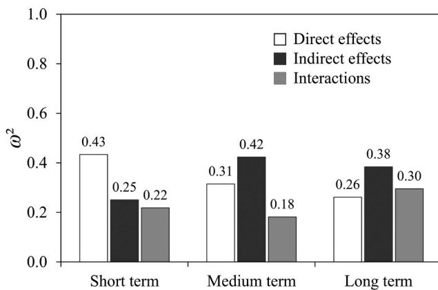
FIGURE 5 Relative importance of direct effects, indirect effects and their interactions on (a) total ROB disturbed area at different time steps. The \omega^2 values were obtained through two-way factorial ANOVA analyses performed at time step 2050 (short term), 2100 (medium term) and 2150 (long term)
