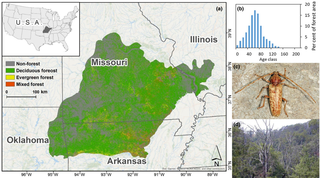
FIGURE 1 (a) Geographical location and forest distribution of the study area. (b) Forests in this study area have a unimodal age distribution with the majority of acres clumped between 40 and 90 years of age. (c) Adult red oak borer. (d) The outbreaks of red oak borer have been observed and suggested as one of the important contributing factors to the severe oak decline in the central U.S. (from Wargo et al., 1983)
