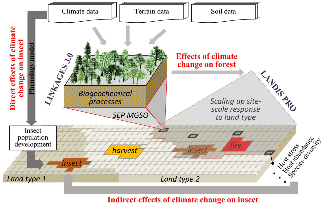
FIGURE 2 The framework of coupling LANDIS PRO and LINKAGES (3.0) to include both direct effects and indirect effects under alternative climates
