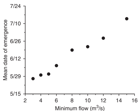
FIGURE 5 Timing of fry emergence from redds in simulations of the eight flow scenarios. The Y axis is the mean day on which emergence was completed, over all simulated redds
