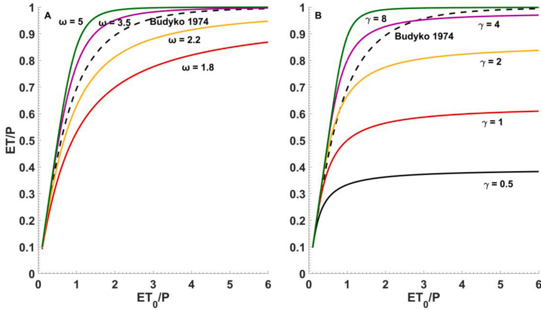
Fig. 1. Budyko-type curves, using (A) The original Budyko equation and Fu's equation when \omega was taken as 1.8, 2.2, 3.5, and 5 (from bottom to top), respectively; (B) Milly's equation when \gamma was taken as 0.5, 1, 2, 4, and 8 (from bottom to top), respectively. The default Budyko-curve (Budyko, 1974) corresponds to a n value of 1.9 and a \omega value of 2.6.
