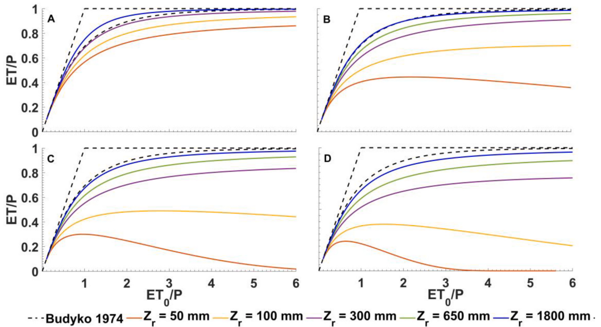
Fig. 3. Annual ET_0/P \sim ET/P curves from the BCP model (Yang et al., 2016) under conditions with different values of Z_r (50, 100, 300, 650, 1800 mm) and \alpha (5, 100, 300, 650, 1800 mm). (A) \alpha = 5 mm; (B) \alpha = 20 mm; (C) \alpha = 35 mm; (D) \alpha = 50 mm.
