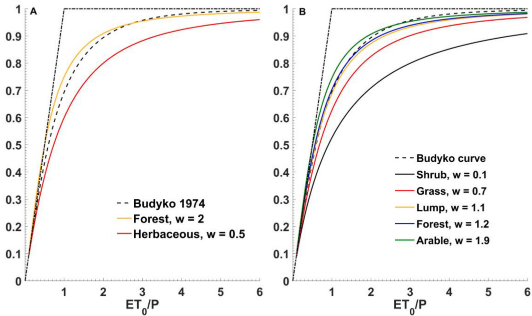
Fig. 2. Characterization of vegetation effects on annual water balances using Budyko curves with different values of plant-available water coefficient ( w ), (A) Forests and herbaceous plants were discriminated in Zhang et al. (2001), and (B) w were taken as 0.1, 0.7, 1.2, and 1.9 for shrubland, grassland, forests, and arable land, respectively, in Oudin et al. (2008).
