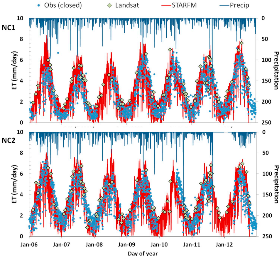
Fig. 5. Time series plot of simulated and observed 30-m daily ET at the NC1 (top, young plantation) and NC2 (bottom, mid-rotation plantation) site, respectively. Shown are the observed fluxes (blue circles), ET retrievals on Landsat overpass days (yellow diamonds), STARFM fused daily ET (red line) and precipitation observed at each flux tower (blue bars). There is a measurement gap at the end of 2011 and beginning of 2012 at NC2. (For interpretation of the references to color in this figure legend, the reader is referred to the web version of this article.)
