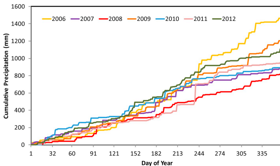
Fig. 2. Annual cumulative measured daily precipitation for the period from 2006 to 2012 at the NC1 flux tower site.
