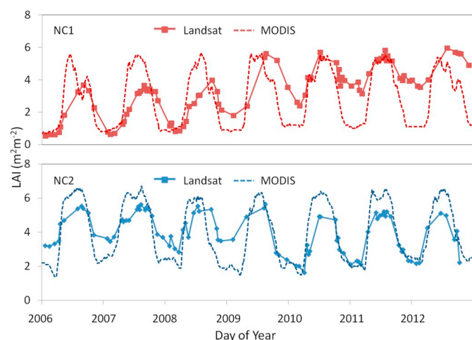
Fig. 6. LAI values extracted from Landsat and MODIS DisALEXI model inputs over the NC1 and NC2 eddy flux sites.
