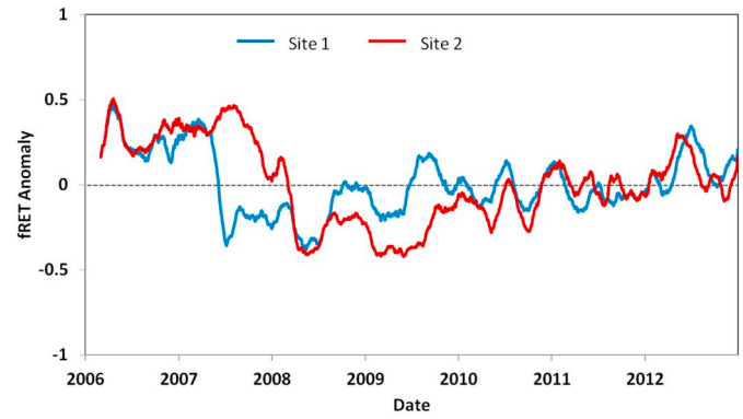
Fig. 12. Daily time series of \Delta f_{RET} over Site 1 and Site 2 (extracted over the polygons containing the disturbed stands located within the red and blue rectangles highlighted in Fig. 11) from 2006 to 2012. (For interpretation of the references to color in this figure legend, the reader is referred to the web version of this article.)
