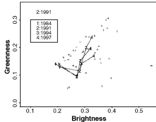
Fig. 6. Spectral history for age class 1 stands in the brightness/greenness space in the 1984 image, indicating that some stands were clear cut between 1984 and 1991. Stand age classes 1 and 2 in the FIA dataset will not apply to the 1984 image. Similar problem can occur to some plots in other age classes in 1997 image because such change could happen during the time between FIA data collection and image acquisition. These stands can be identified and removed from statistical analysis.
