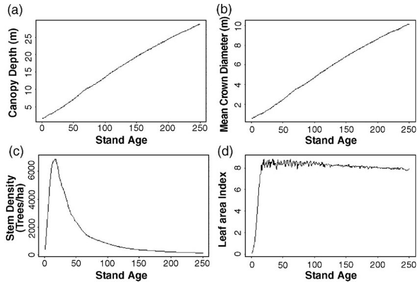
Fig. 2. Change of overstory canopy structure as simulated with ZELIG model for the H. J. Andrews Experimental Forest over 250 years. The simulation is conducted for 50 independent plots. The canopy structure parameters shown here are the mean values averaged over all plots simulated.
