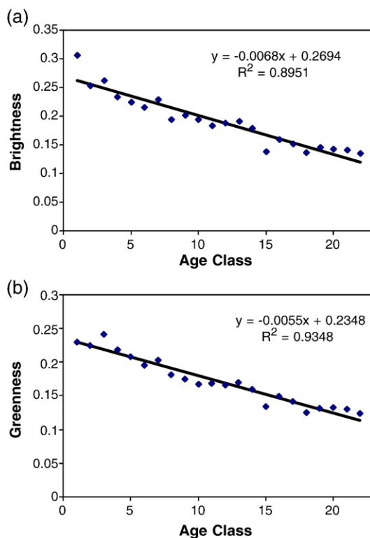
Fig. 7. A linear model fits the regional mean succession trajectories in (a) brightness and (b) greenness well with the 1997 image. Note points in this Figure are the same points as seen in Fig. 4(a, b). The large cross-site variation almost masked the nonlinearity at individual stand scale.
