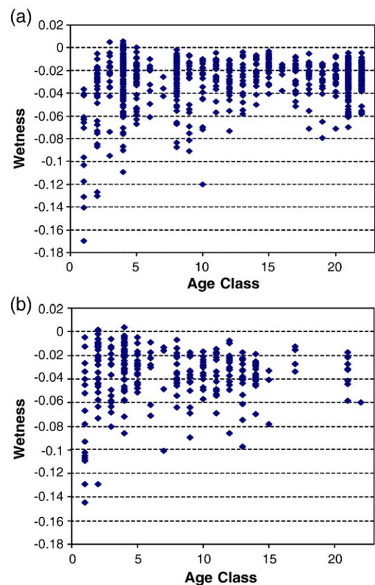
Fig. 5. Spectral trajectory of wetness separated for (a) western Cascades and (b) Coastal Ranges. The decreasing trend of wetness from mature to old-growth is much clearer when the two ecoregions are viewed separately than view together as seen in Fig. 4c.
