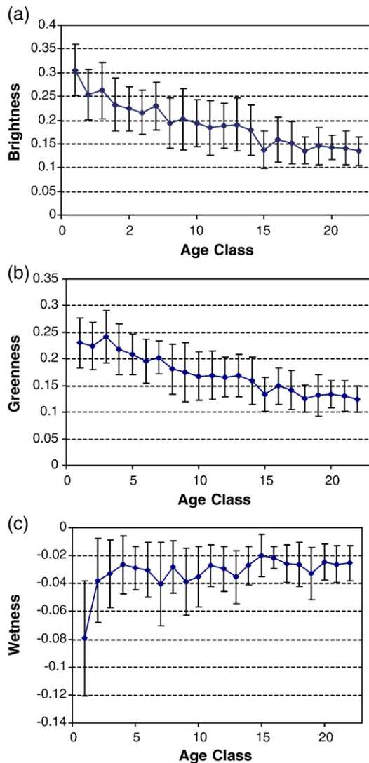
Fig. 4. Observed trajectory of brightness, greenness and wetness of Tasseled Cap transformation with stand age from FIA plots in the 1997 image. Each point is the mean value from all plots within the age class, and the vertical error bars are \pm 1 SD. The simulated trajectories in Fig. 3 captured the major characteristics of the observed trajectories here. (a) Regional mean successional trajectory of brightness; (b) regional mean successional trajectory of greenness; (c) regional mean successional trajectory of wetness.
