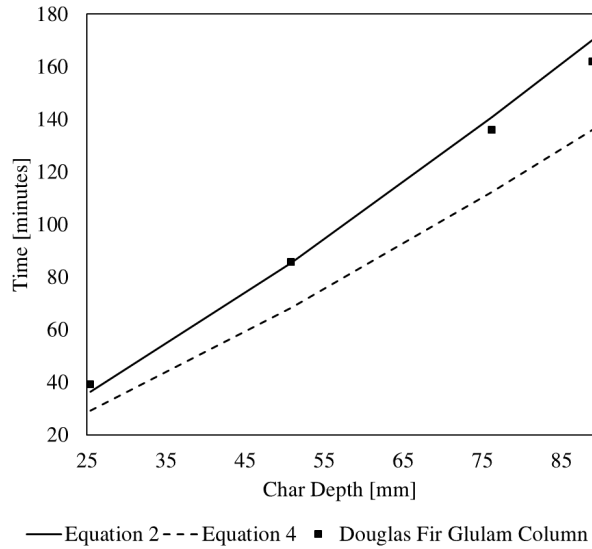
Figure 6: Average measured time to char (300°C) to different depths compared with the models described in Equations 2 and 4.
