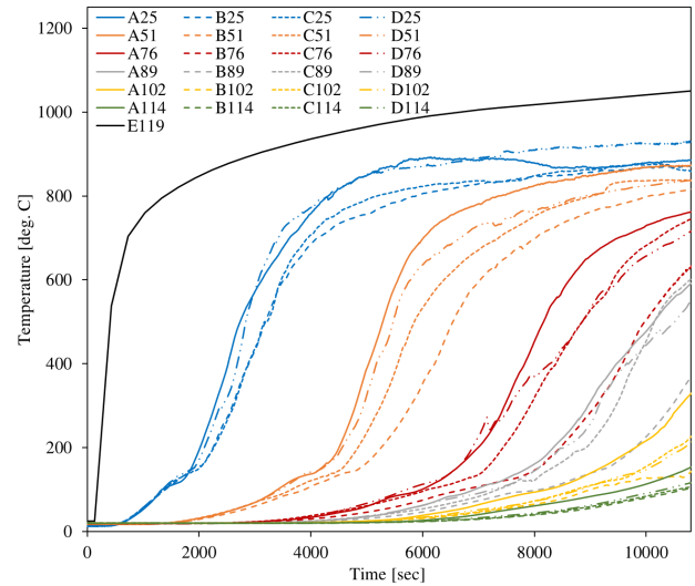
Figure 4: Thermocouple Data from a Douglas-fir glulam column.
