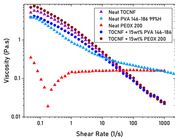
Fig. 8 Rheology data for neat TOCNF, neat PVA 146–186 99%H, and neat PEOX 200 solutions shown as triangular dots and composite fluids in circular dots. All TOCNF specimens are at constant 0.53 wt% TOCNF with any polymer added at 15 wt% to this
