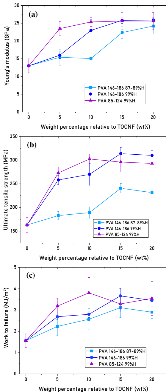
Fig. 3 Tensile mechanical properties of c-TOCNF and PVA nanocomposites. a Young's modulus, b Ultimate tensile strength and c Work of failure
