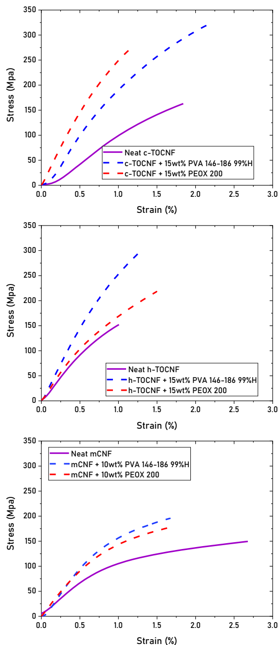
Fig. 6 Representative stress–strain plots of neat and optimized PVA and PEO 200 composite c-TOCNF, h-TOCNF and mCNF films
