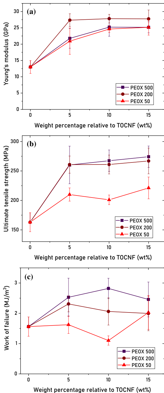
Fig. 4 Tension properties of c-TOCNF and PEOX nanocomposites. a Young's modulus, b Ultimate tensile strength and c Work of failure
