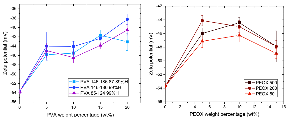
Fig. 7 Zeta potential (mV) measurements of neat c-TOCNF and c-TOCNF composite solutions were fixed at 0.1 wt%. PVA (left) PEOX (right)
