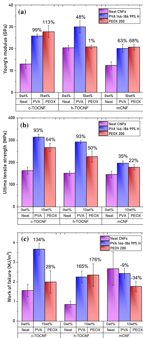
Fig. 5 Mechanical response of different CNFs (c-TOCNF, h-TOCNF, mCNF) with different weight percentages of PVA and PEOX. a Young's modulus, b Ultimate tensile strength and c Work of failure
