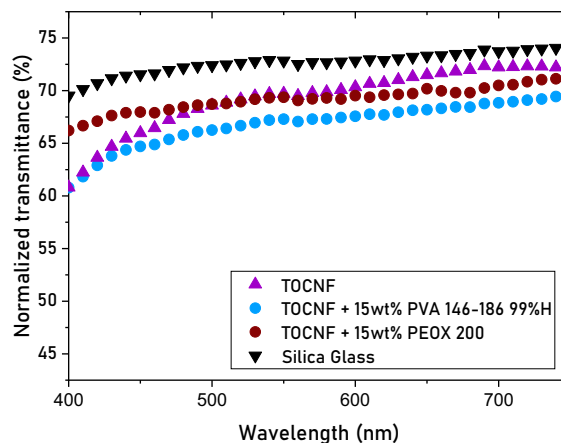
Fig. 2 Visible transmittance via UV–Vis spectroscopy of neat TOCNF, TOCNF composites and silica glass. Thickness was normalized using the silica glass thickness as reference (0.9 mm)
