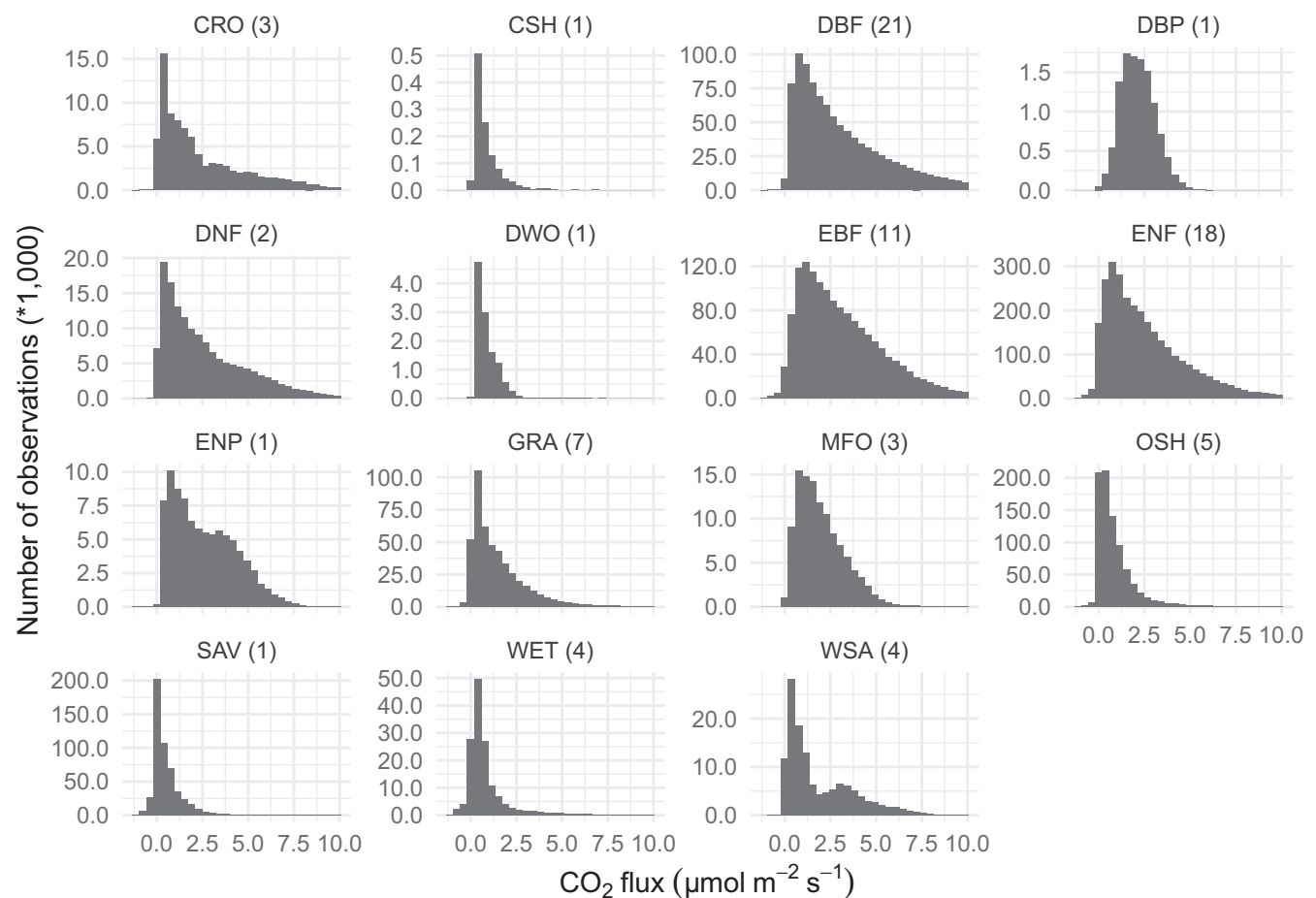
FIGURE 8 Distribution of CO 2 fluxes in COSORE datasets, by IGBP classification (cf. Table 1). For visual clarity this figure excludes fluxes <-1 and >10 μmol m -2 s -1 (210,752 observations, 2.6% of the data). Number of datasets (sites) making up data is given in parentheses after IGBP abbreviations in each panel
