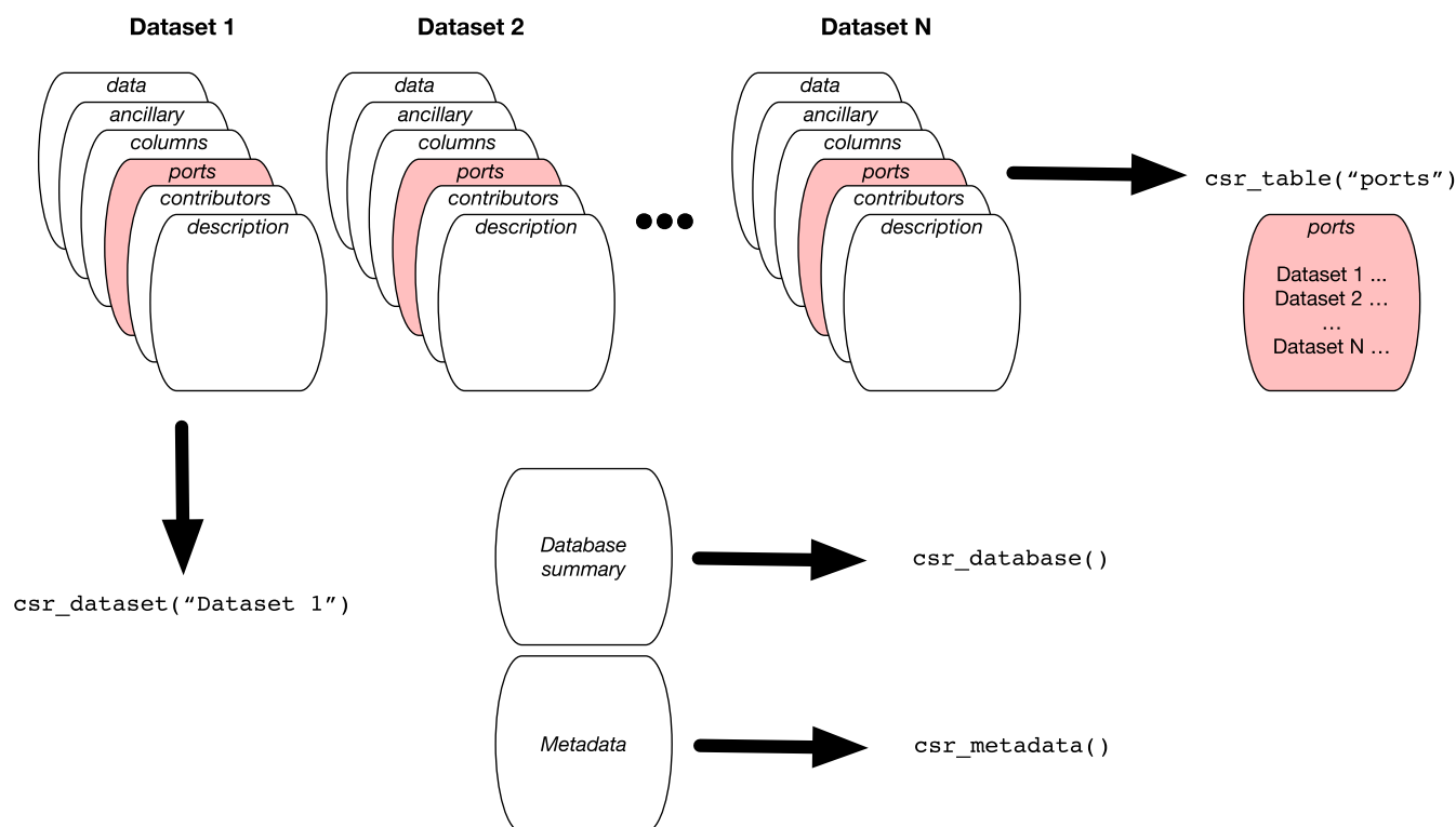
FIGURE 1 Summary of COSORE structure (multiple datasets, each with six tables; Tables 2–7) and primary accessor R functions, as described in the text (see Section 2.1 in text). For example, R users can join specific tables across all datasets using the csr_table() function, and can access individual datasets with csr_dataset() . Non-R users access flat-file versions of the same data, with essentially the same structure as the R internal structure shown here
