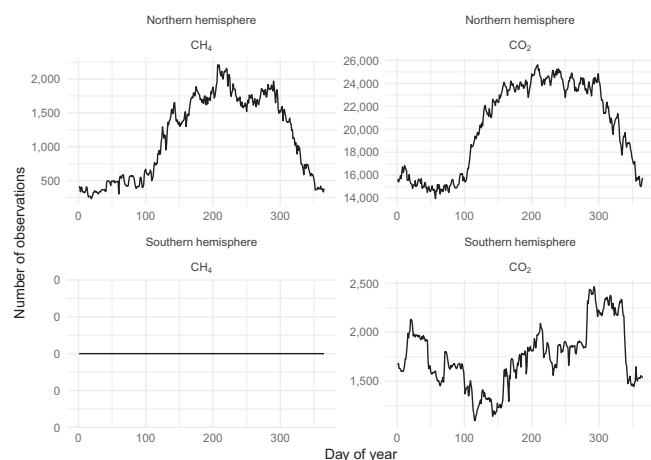
FIGURE 6 Number of observations by day of year, for northern and southern hemisphere and by gas ( \text{CO}_2 or \text{CH}_4 ), in the current COSORE datasets; the database currently has no \text{CH}_4 data from the Southern hemisphere (bottom left)
