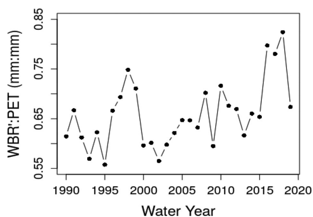
FIGURE 11 Time series of the area weighted water budget residual (WBR') to potential evapotranspiration (PET) ratio from water year 1990 to 2019
