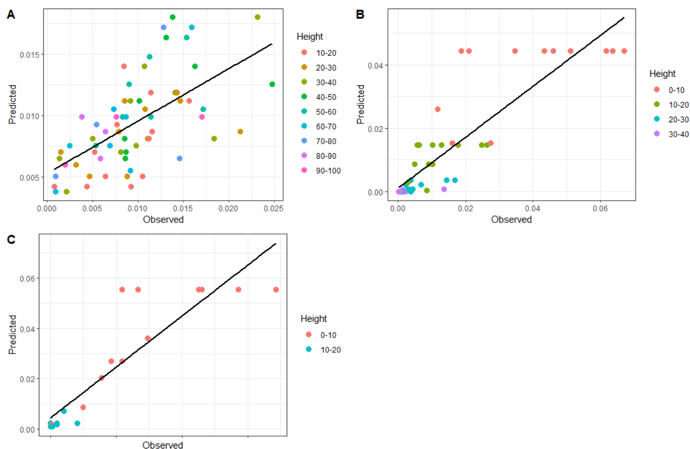
Figure 3. Predicted vs. actual plots for live woody material (A), herbaceous fuel (B), and woody litter (C). Lines represent linear regression with R^2 values of 0.37, 0.75, and 0.79 for A, B, and C respectively.
