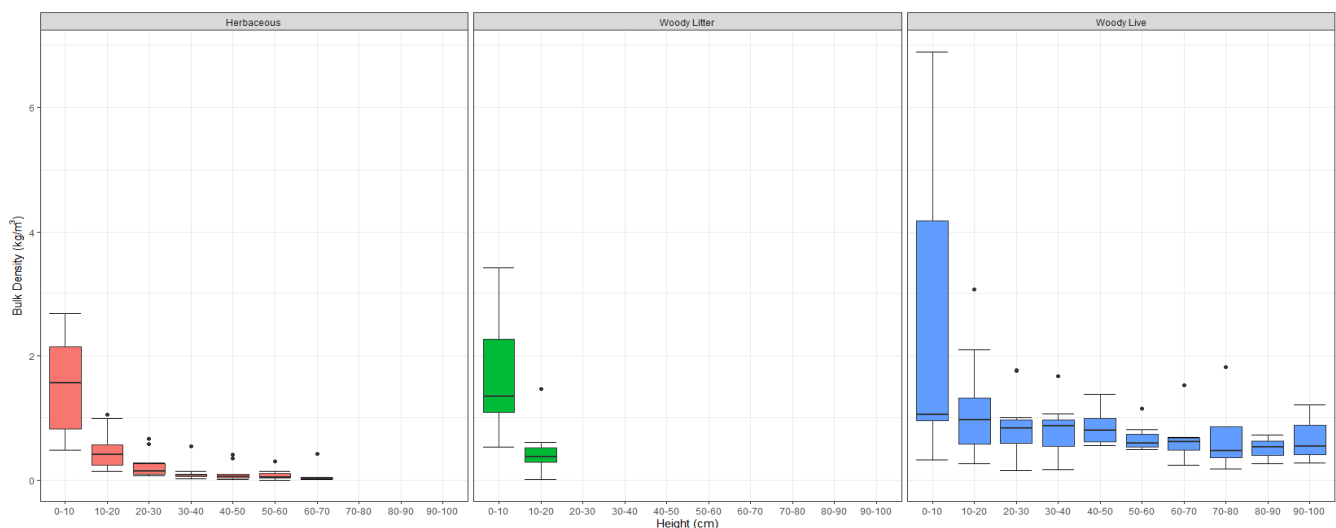
Figure 1. Bulk density values for all fuel types from stratum 0 to 100 cm, in 10 cm increments.
