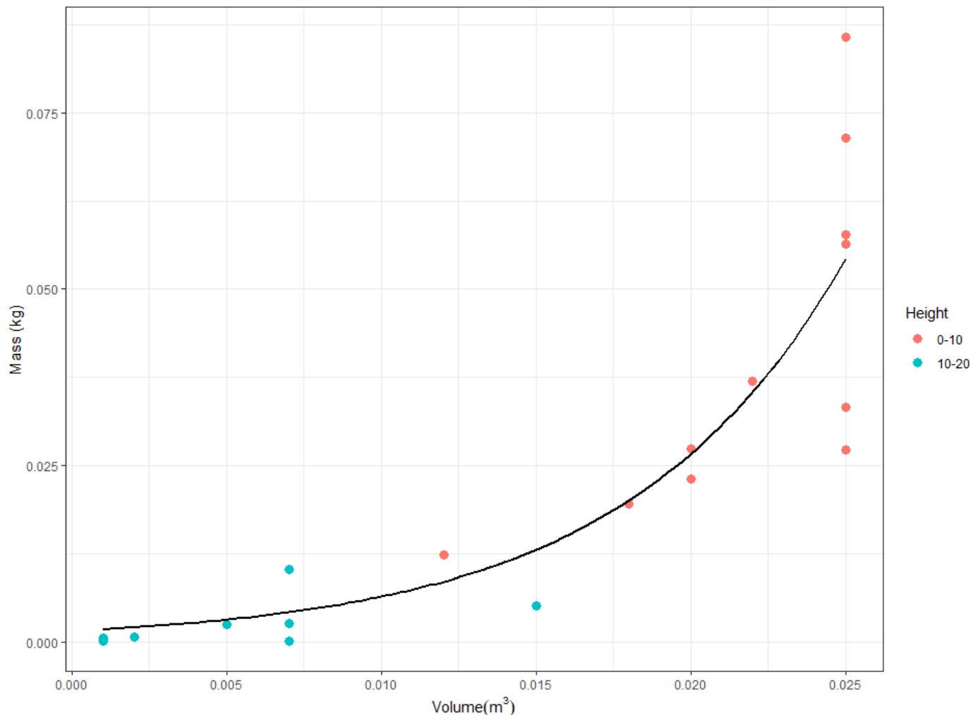
Figure 5. Exponential, nonlinear regression for woody litter fuel material with both volume and height as predictors of mass. Only mass and volume observations associated with the strata between 0 and 20 cm were included. Using this equation, loading was calculated for each plot pre-fire using both the voxelized volume and height (Figure 3). The median ( \pm IQR) fuel consumption was 19.83 \pm 4.01 g (Table 3). For the paired plots, the median ( \pm IQR) fuel consumption was 20.83 \pm 4.53 g (Table 3).
