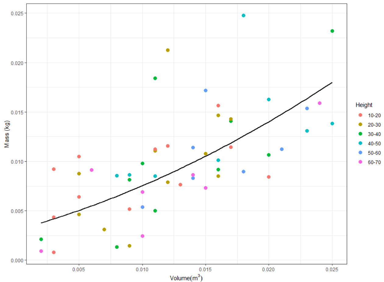
Figure 2. Regression for live woody fuel material with volume as a predictor of mass (mass has been backtransformed from square root). The equation was significant ( p < 0.001 ), with an R^2 of 0.44. Only mass and volume observations associated with the strata between 10 and 70 cm were included.
