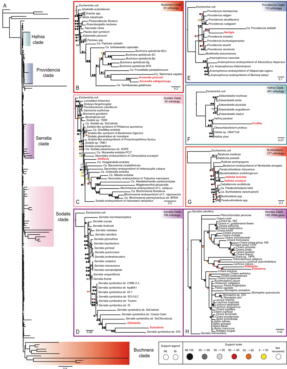
Fig. 2 Phylogenetic relationships of adelgid endosymbionts within each major Adelgidae lineage. A Multi-gene Bayesian phylogeny of the Enterobacterales with 158 taxa inferred from 70 orthologs recoded under the Dayhoff-6 scheme. Colors indicate clades of taxa at the family level to which adelgid symbionts belong. B–F Maximum likelihood (shown) and Bayesian phylogenies of individual clades in which adelgid symbionts clustered in (A) using orthogroups where all taxa were represented, G Multi-gene maximum likelihood (shown) and Bayesian phylogeny of the Burkholderiales . H. Bayesian 16 S rRNA gene phylogeny of the Serratia symbiotica clade; Serratia symbiotica from aphid species are denoted by aphid species names. Adelgid symbiont names are shown in red. Support values are listed as bootstrap replicates supporting nodes for maximum likelihood trees (ML) and percentage posterior probabilities for Bayesian inference phylogenies (BI). Bayesian support values are from analyses conducted on Dayhoff-6-recoded datasets, except for C, where sequences were left uncoded.
