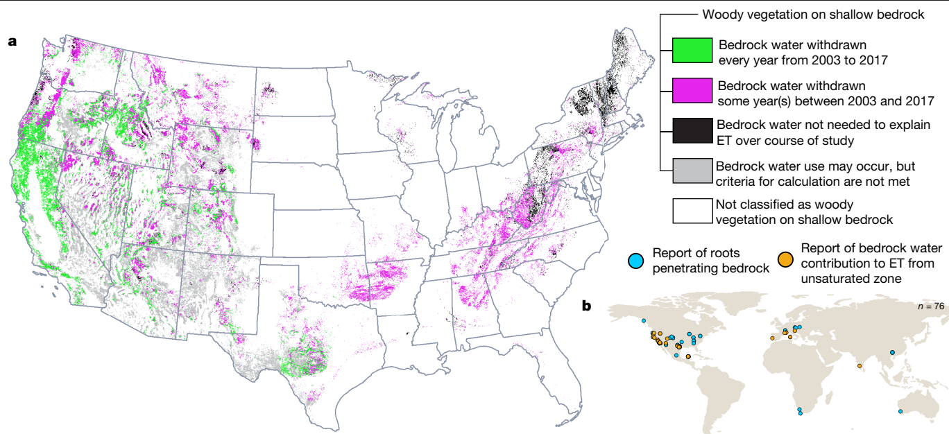
Fig. 2 | Bedrock water use by woody plants is spatially extensive and can be routine. a, The occurrence of bedrock water withdrawal by woody plants in the CONUS from 2003 to 2017. Coloured areas indicate the extent of woody vegetation where bedrock is encountered within the upper 1.5 m. This area is divided into four colours reflecting locations where the annual bedrock water storage deficit ( D_{\text{bedrock},y} ) is greater than zero for every year of the study (green), D_{\text{bedrock},y} is greater than zero for at least one year of the study (pink), D_{\text{bedrock},y} is not greater than zero for any years of the study (black) and D_{\text{bedrock},y} is not reported because our analysis criteria are not met (grey; Methods). An annual
