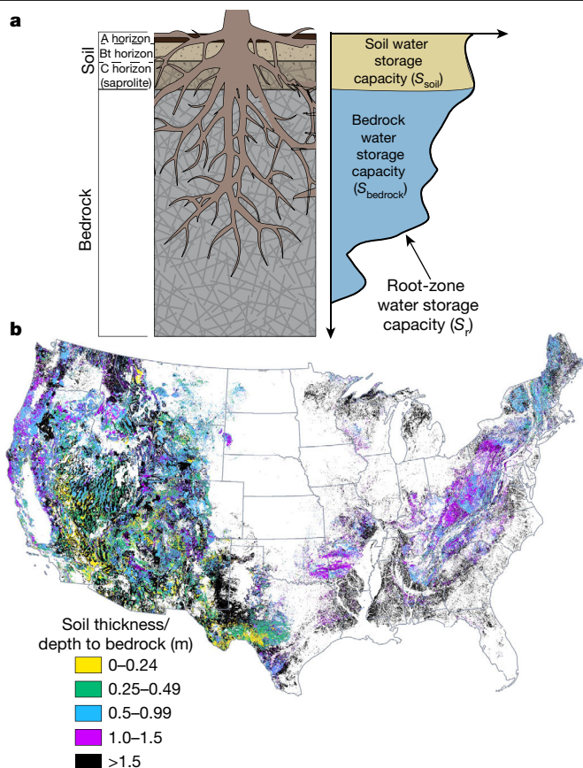
Fig. 1 | Over 45% of the wooded land area across the CONUS is underlain by shallow (<1.5 m deep) bedrock. a, Conceptual diagram of a root-zone including bedrock (left) and a depth profile of root-zone water storage capacity (right). The root-zone water storage capacity is partitioned into soil and bedrock components. b, The extent of woody vegetation is coloured by soil thickness, which could also be considered the depth to bedrock because only areas mapped as underlain by bedrock are shown. Landcover data were sourced from the USGS NLCD 40 and soil thickness from the USDA gNATSGO 41 . All raster maps in all figures and Extended data were plotted in QGIS 42 , with map data generated in Python in the Google Colaboratory environment. All raster data are publicly available and were processed using the Google Earth Engine Python application programming interface (API).
