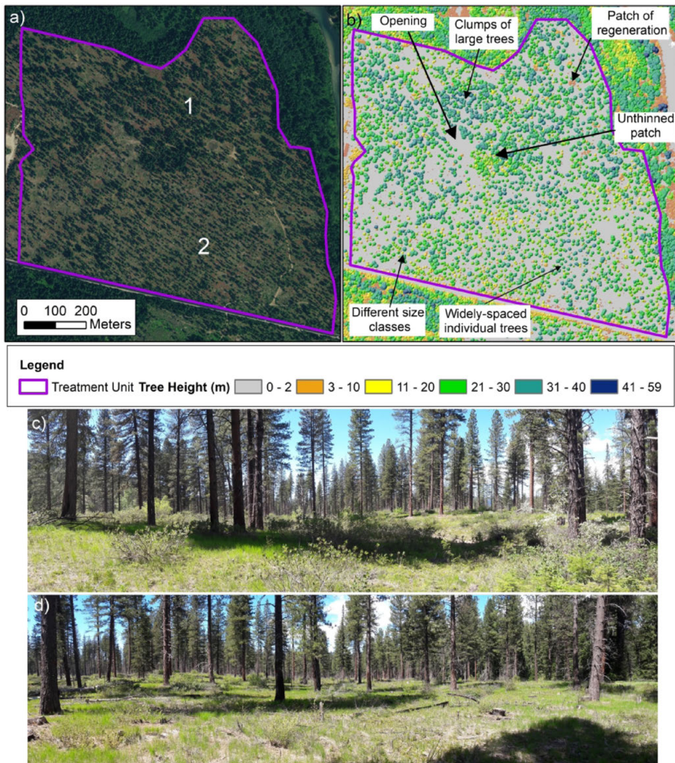
Figure 4. Aerial photograph (a), LiDAR canopy surface image (b), and panoramic photos (c, d) of a treated unit in the Okanogan-Wenatchee National Forest in central Washington, showing design elements of a restoration and fuels reduction prescription. The unit was treated with commercial thinning and prescribed fire. A more spatially variable restoration approach was used in the north half of the unit (no.1 in panel a, photo c), whereas a less variable prescription with a fuels reduction focus was used in the southern half (no.2 in panel a, photo d), which is adjacent to a highway. In photos c and d, note the separation between tree crowns and the base of the crown and the ground, as well as the recovery of understory plant communities. Photographs: Derek Churchill.
